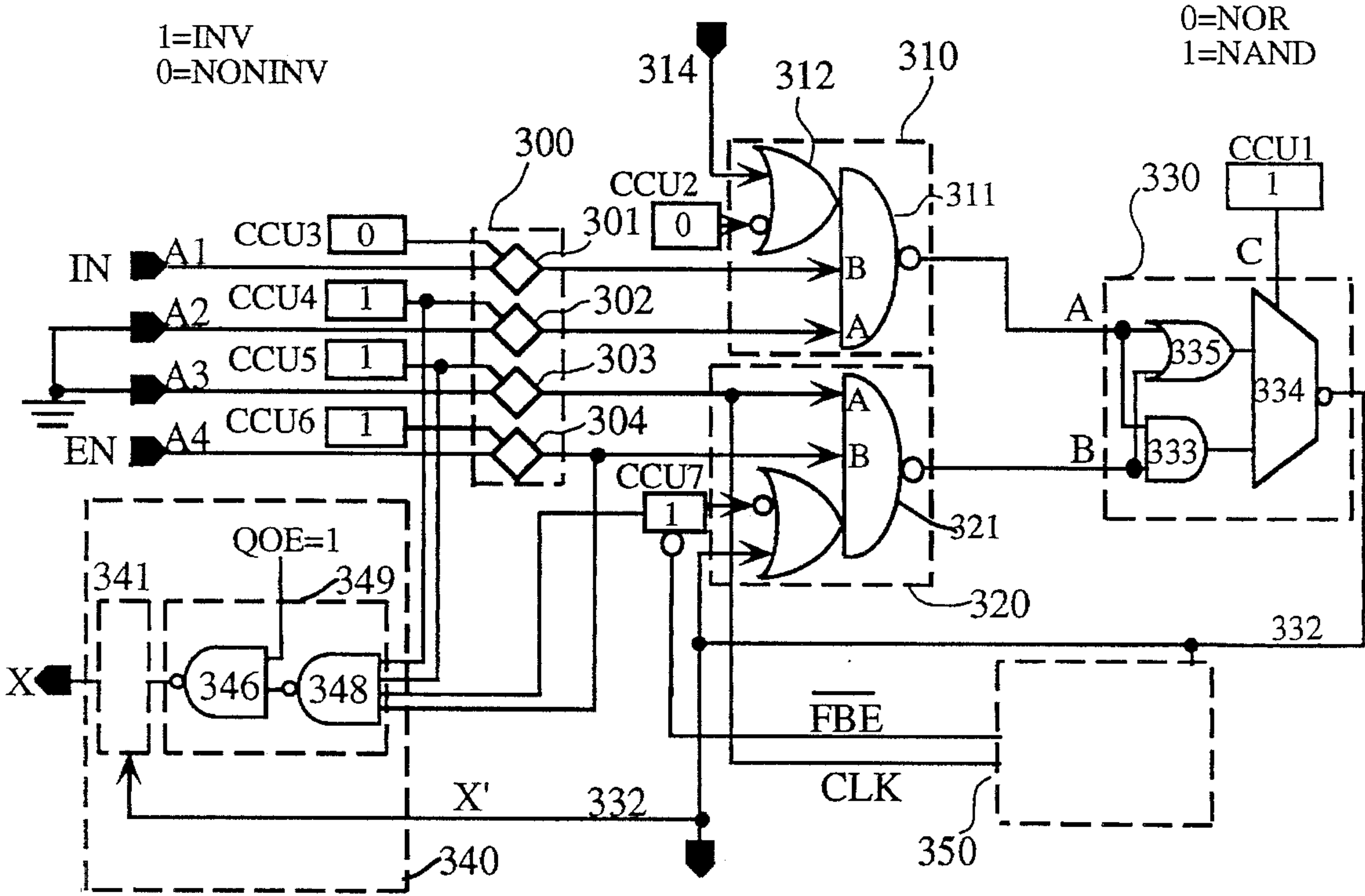
FIG. 20B 3-STATE BUFFER
