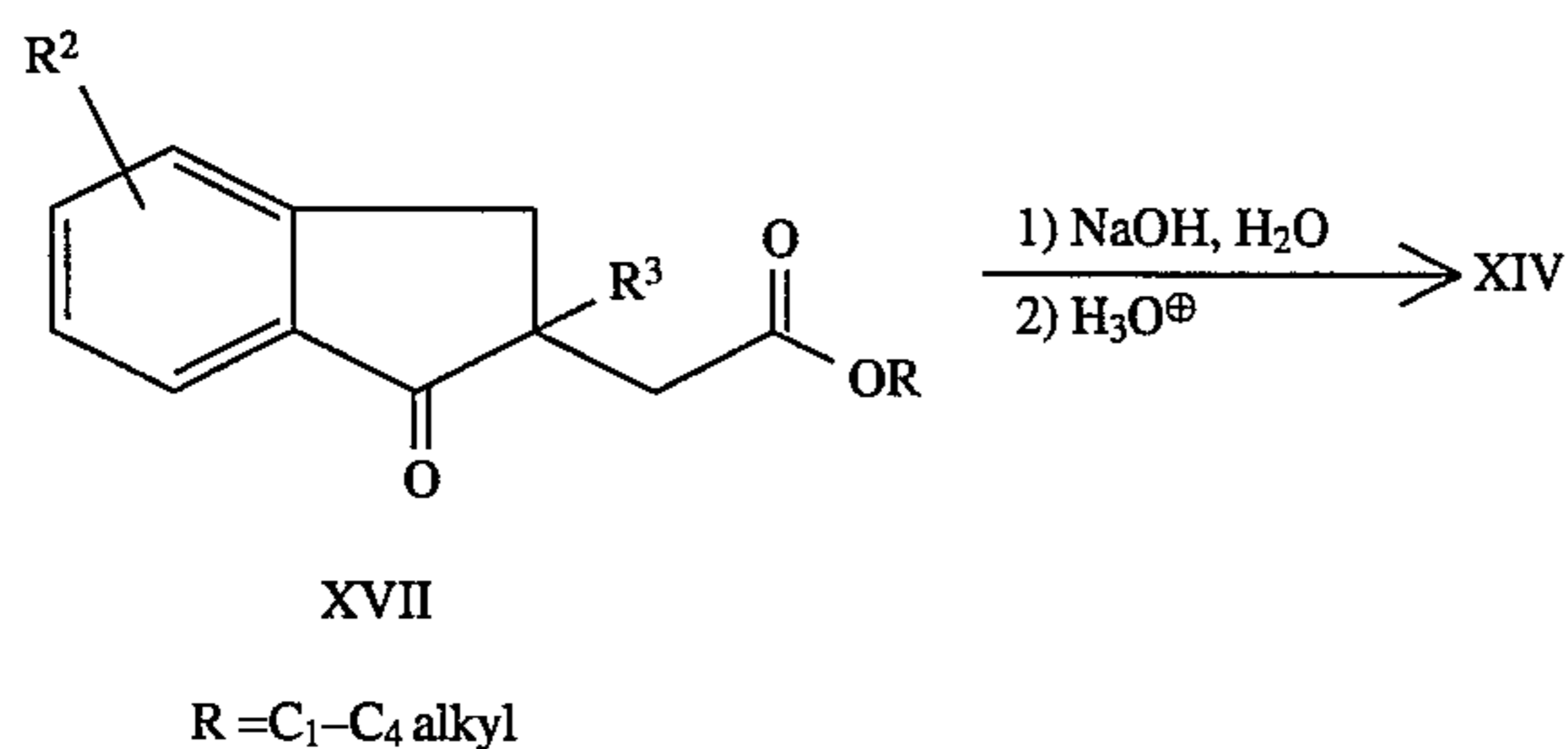
SCHEME 18
