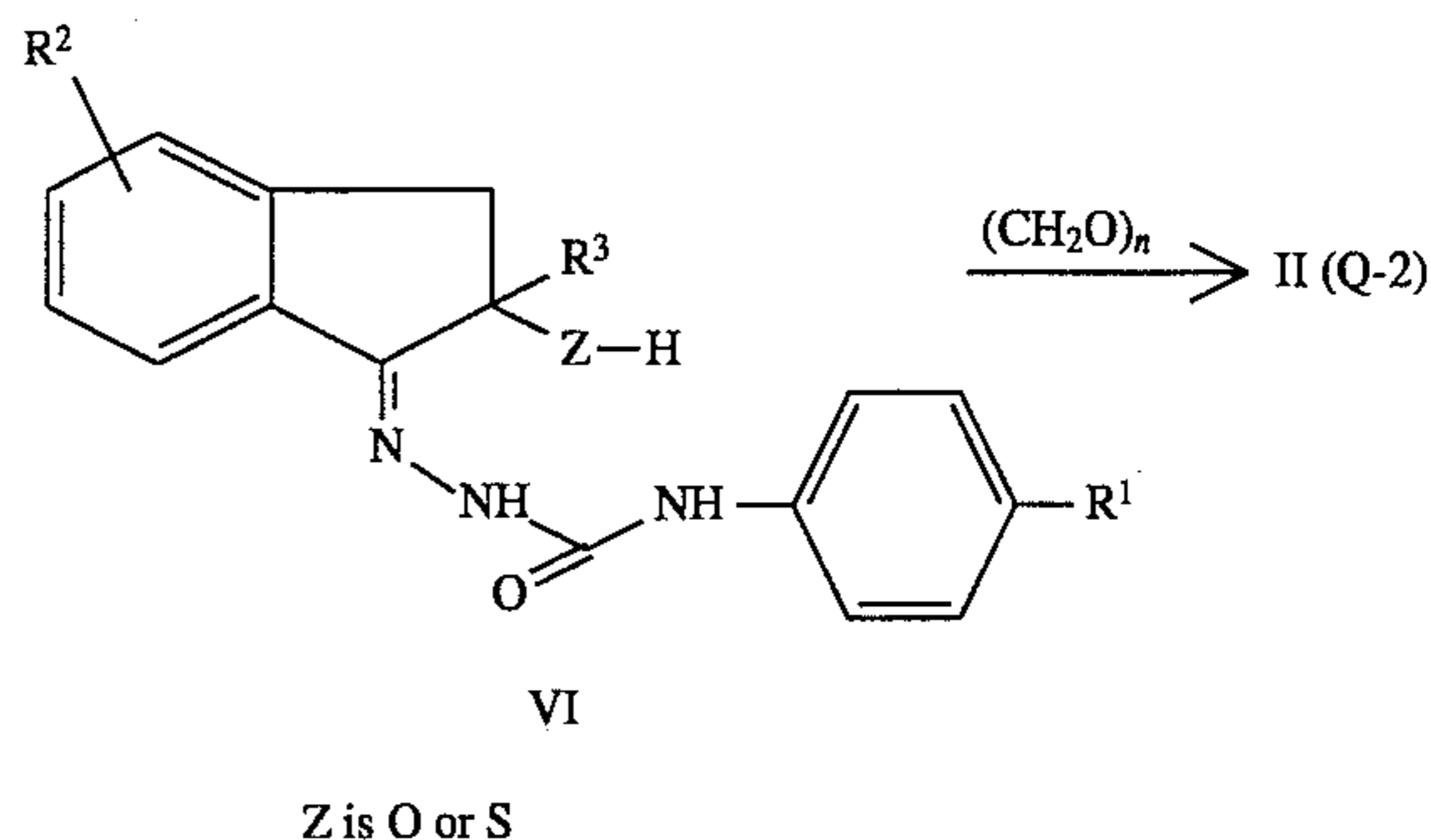
SCHEME 5
