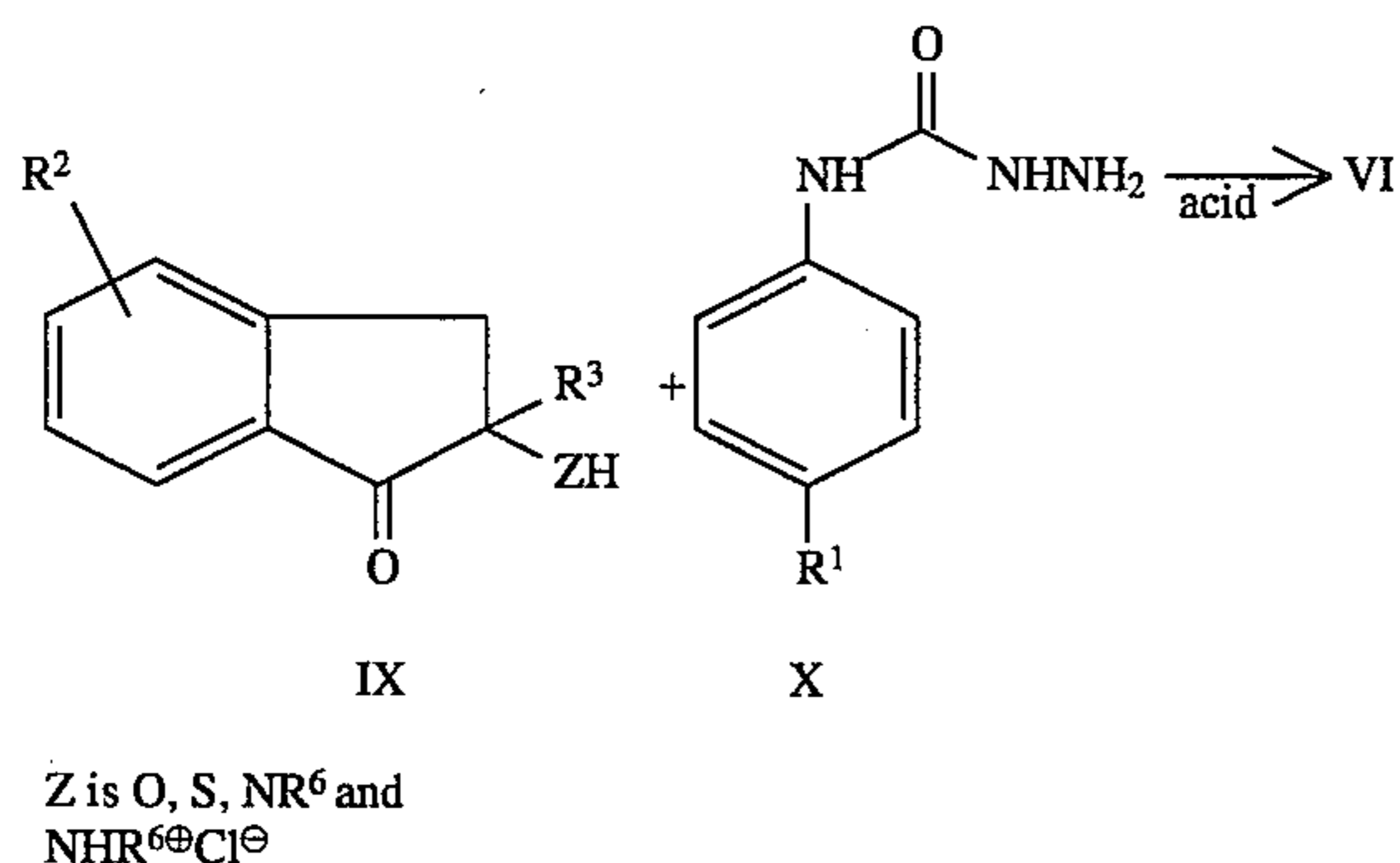
SCHEME 9
