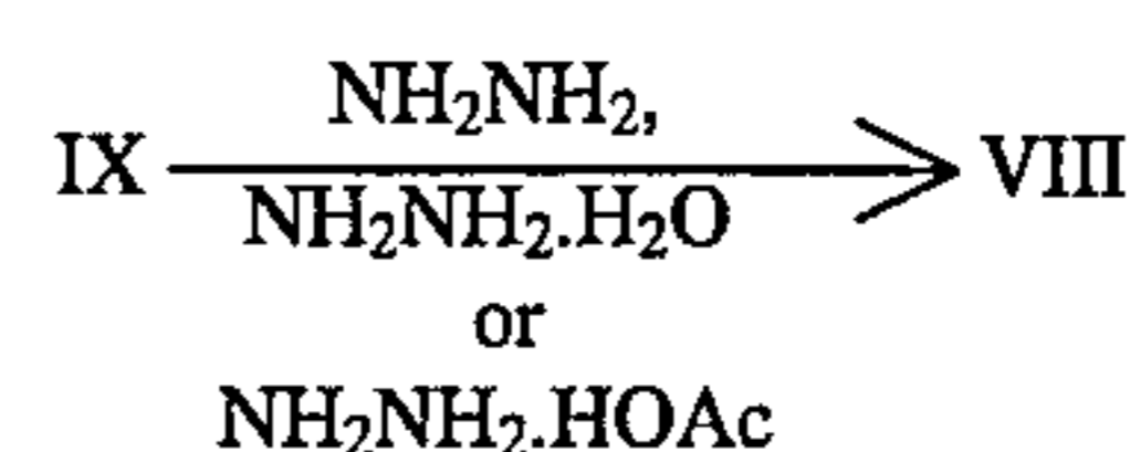
SCHEME 10
