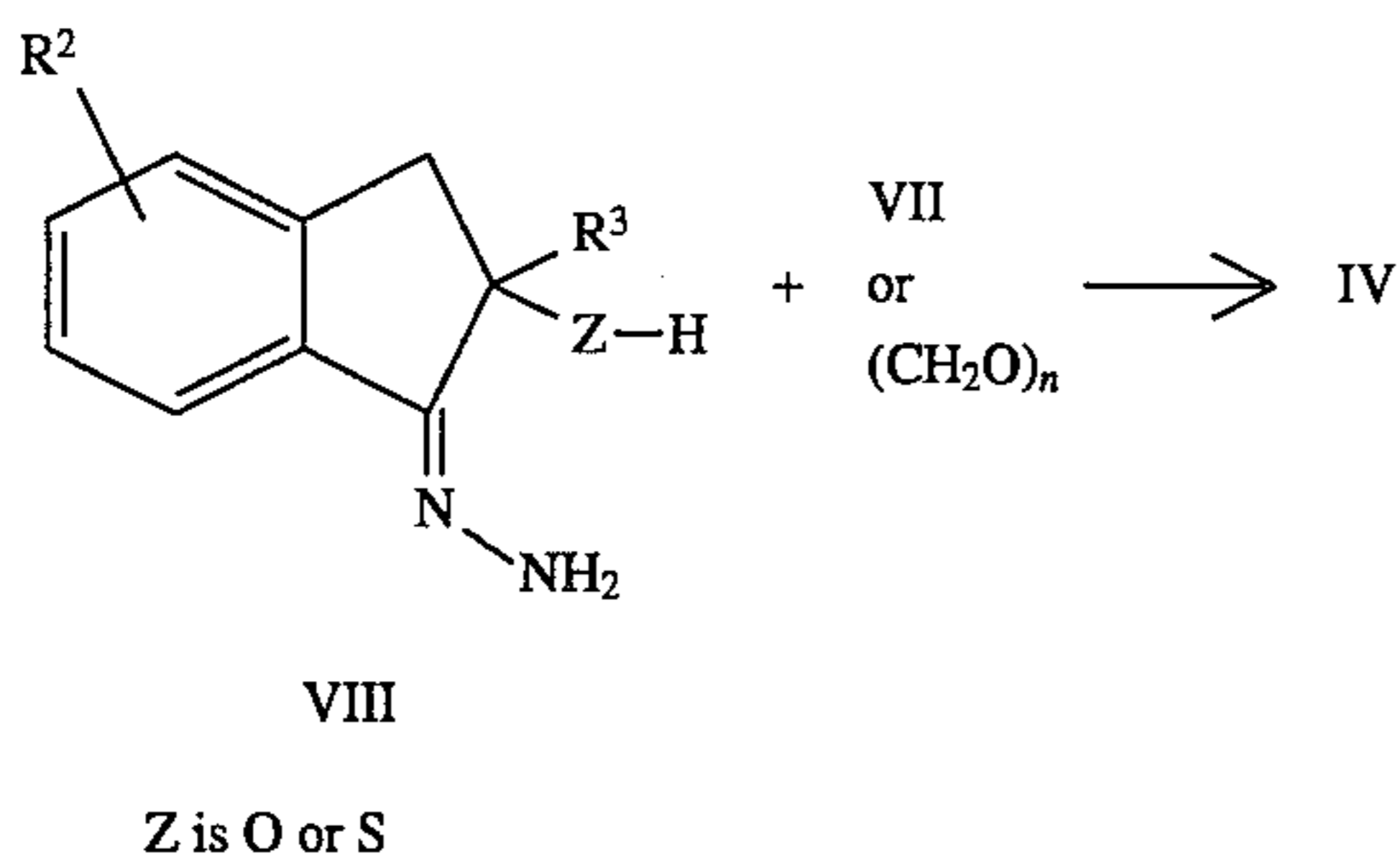
SCHEME 7
