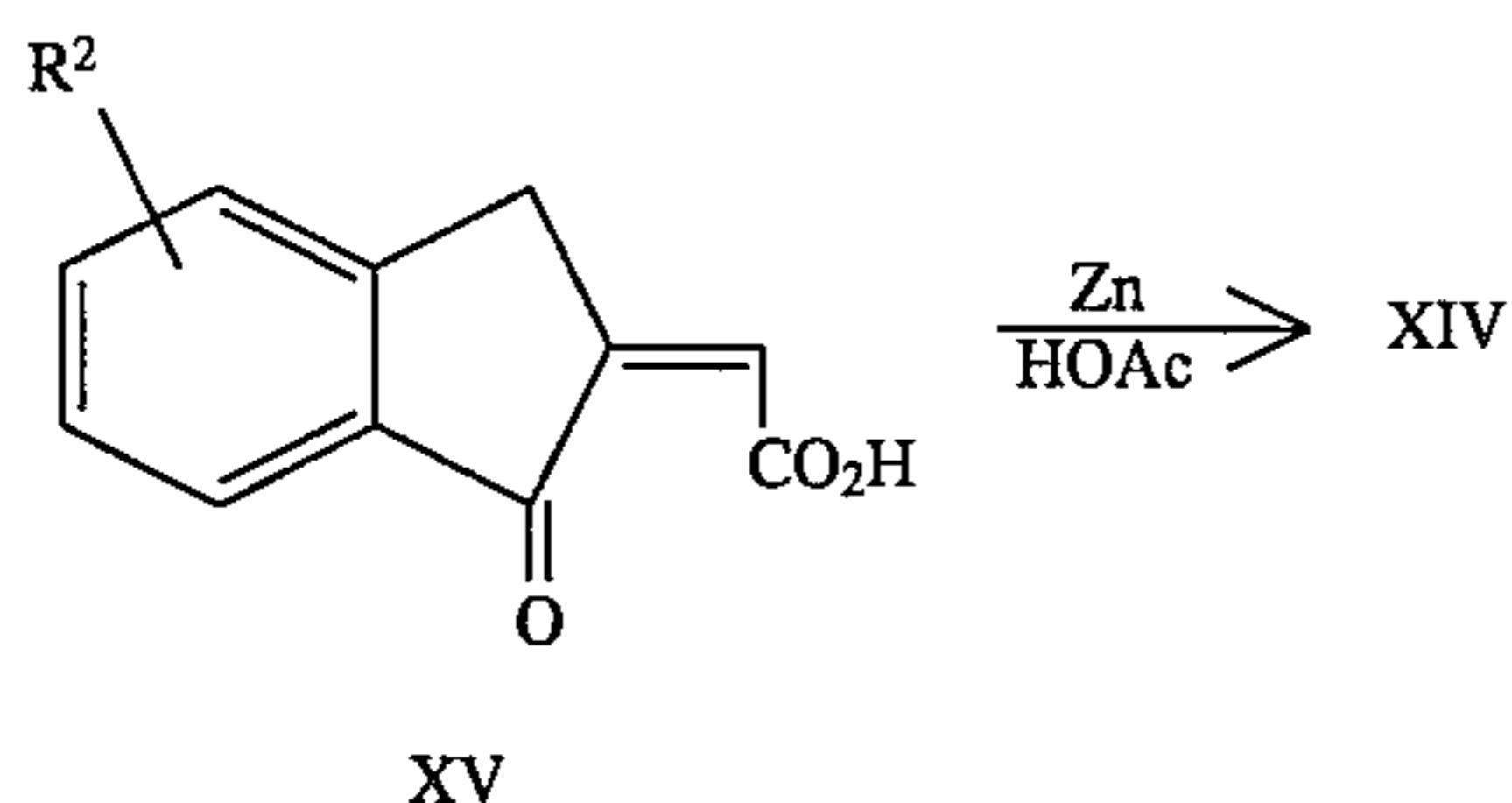
SCHEME 16
