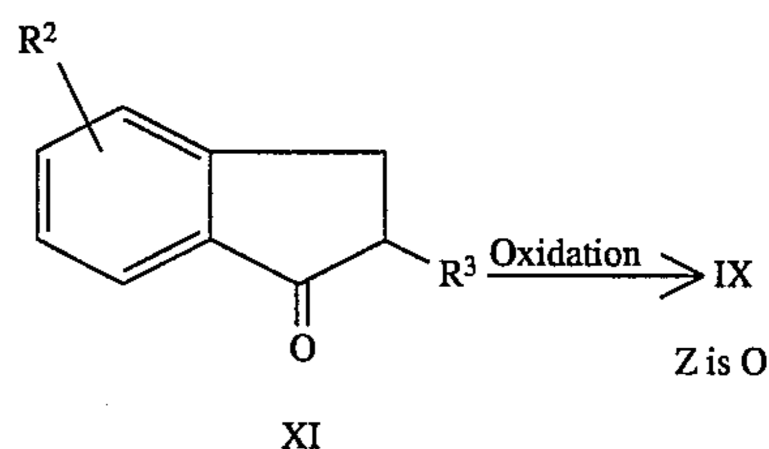
SCHEME 11
