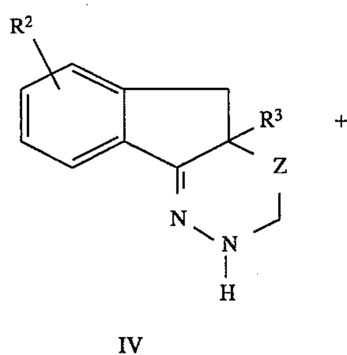
SCHEME 4
