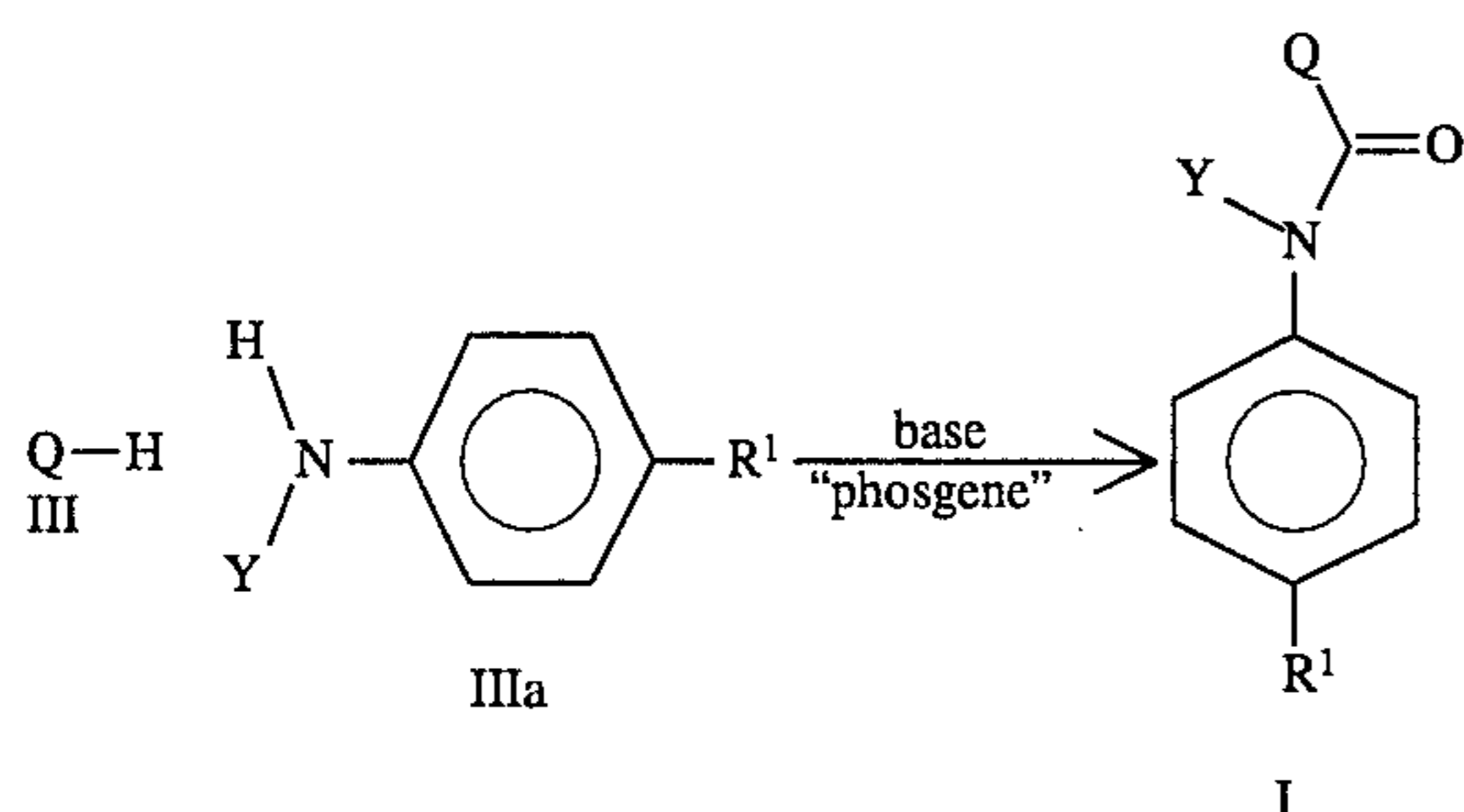
SCHEME 3
