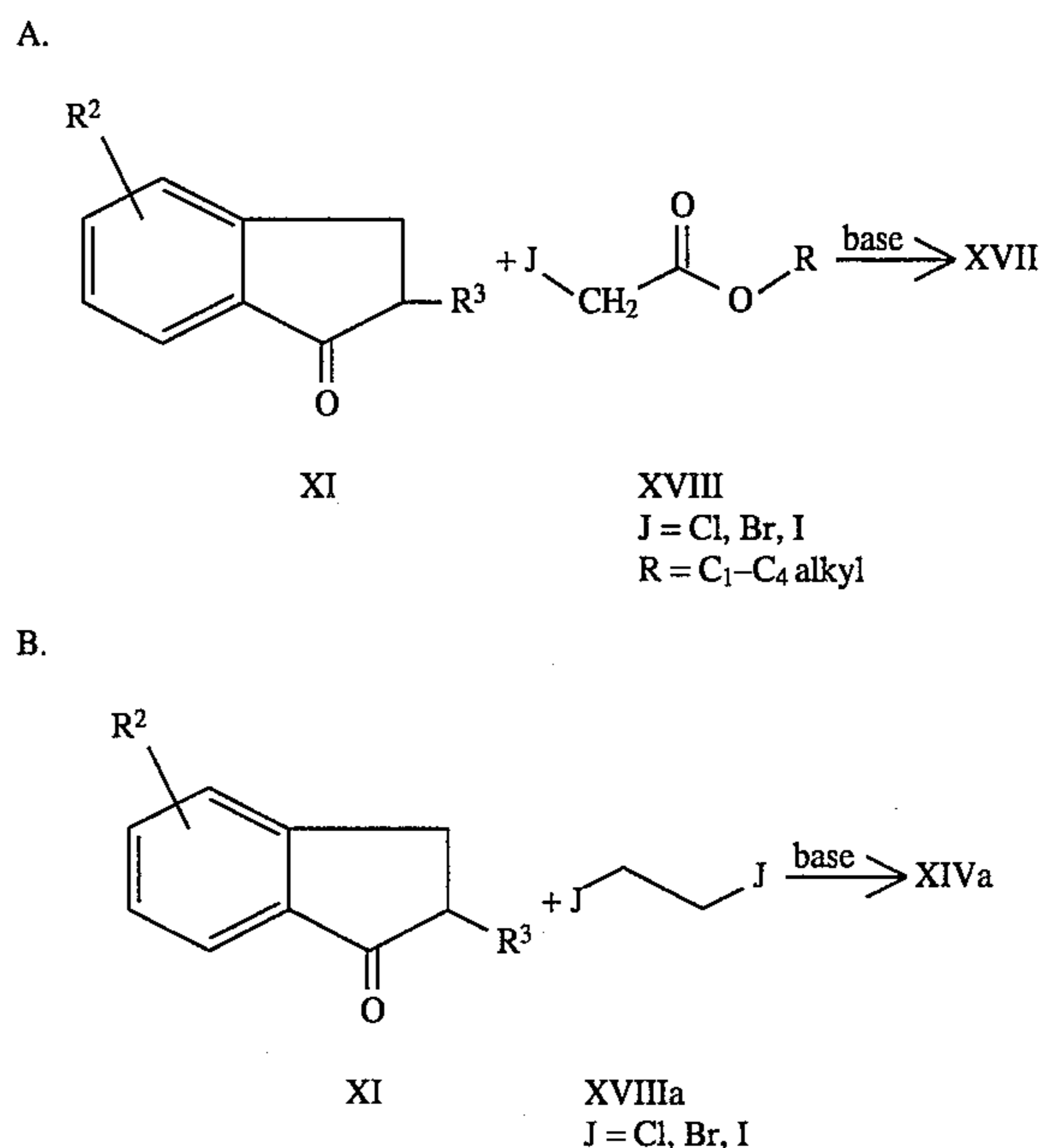
SCHEME 19
