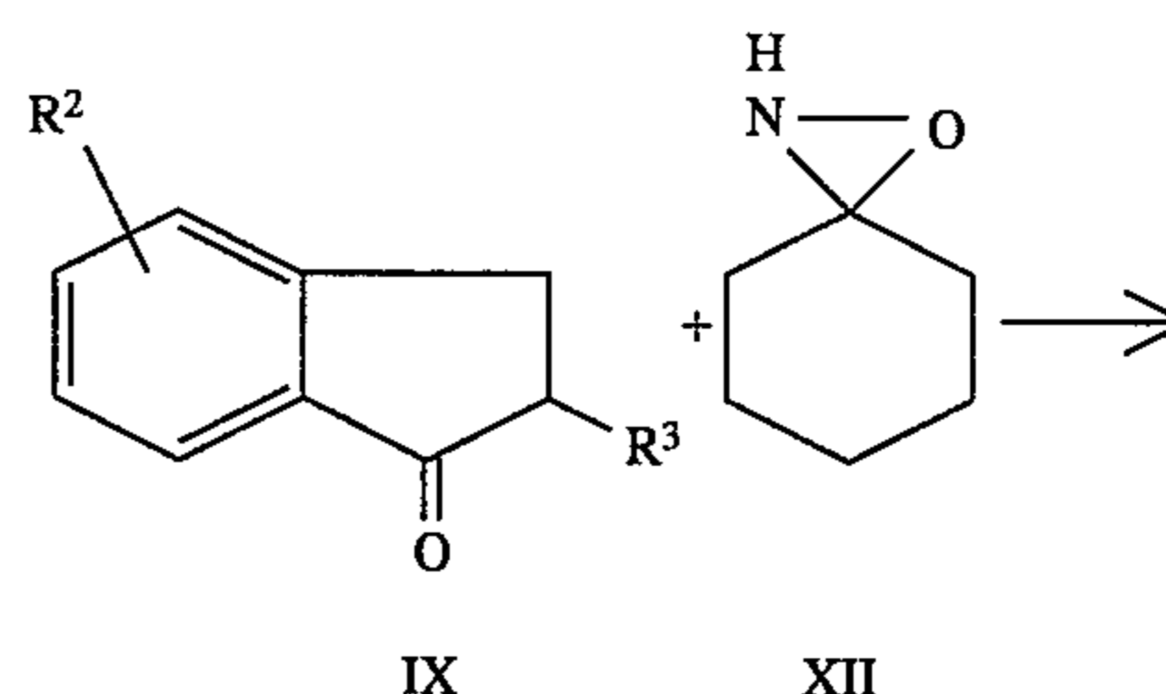
SCHEME 12
