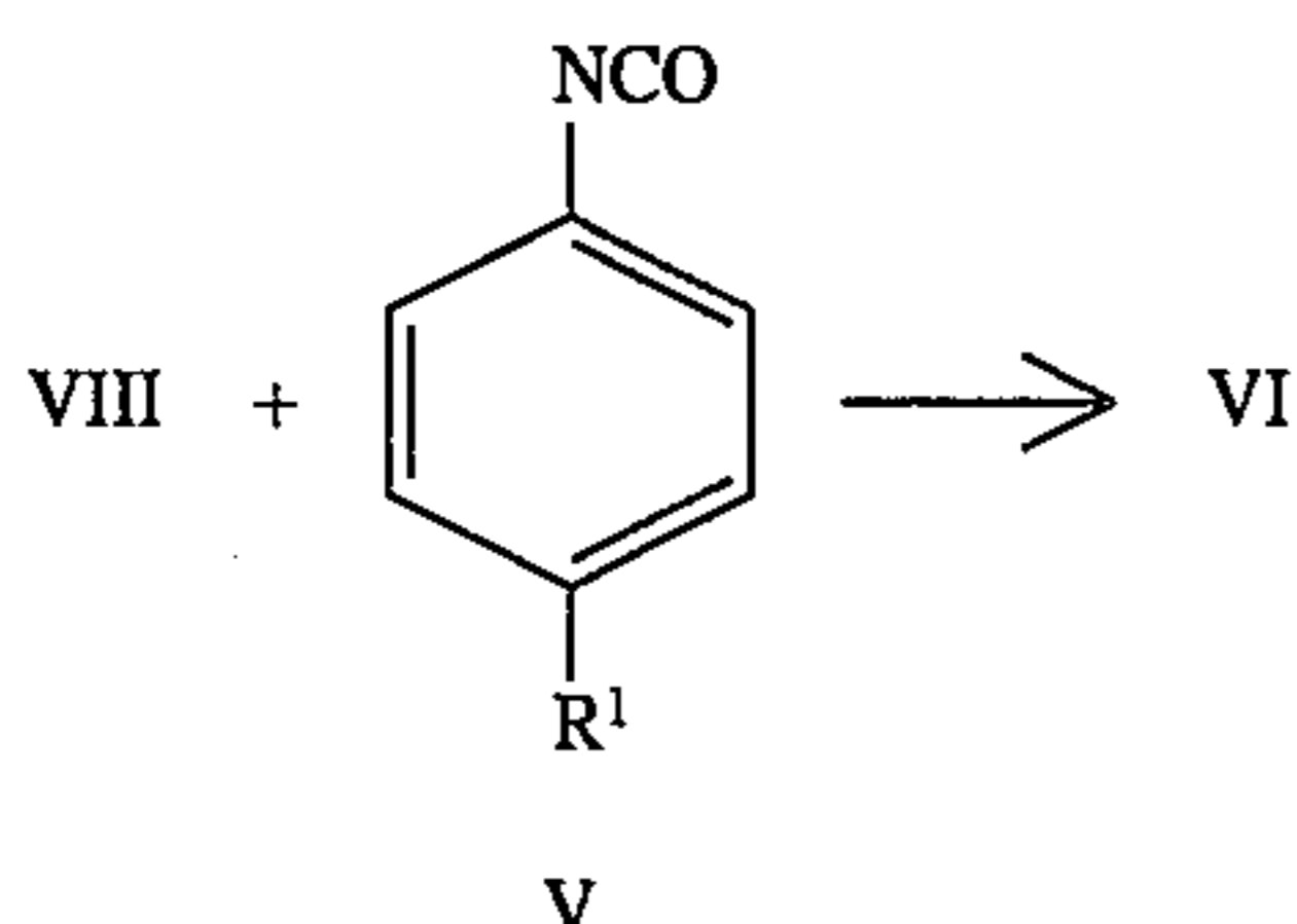
SCHEME 8
