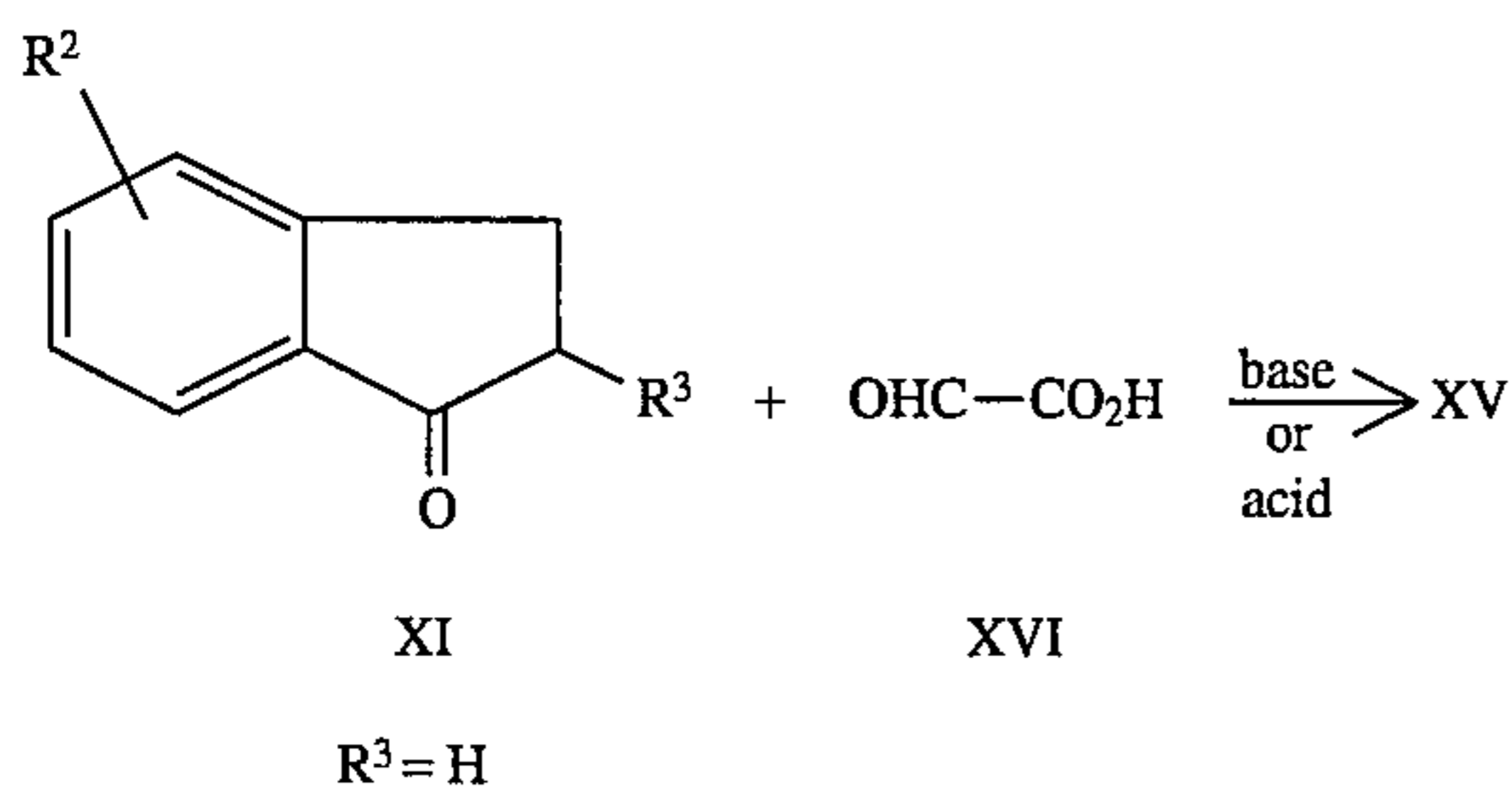
SCHEME 17
