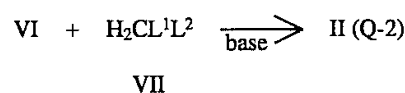
SCHEME 6
