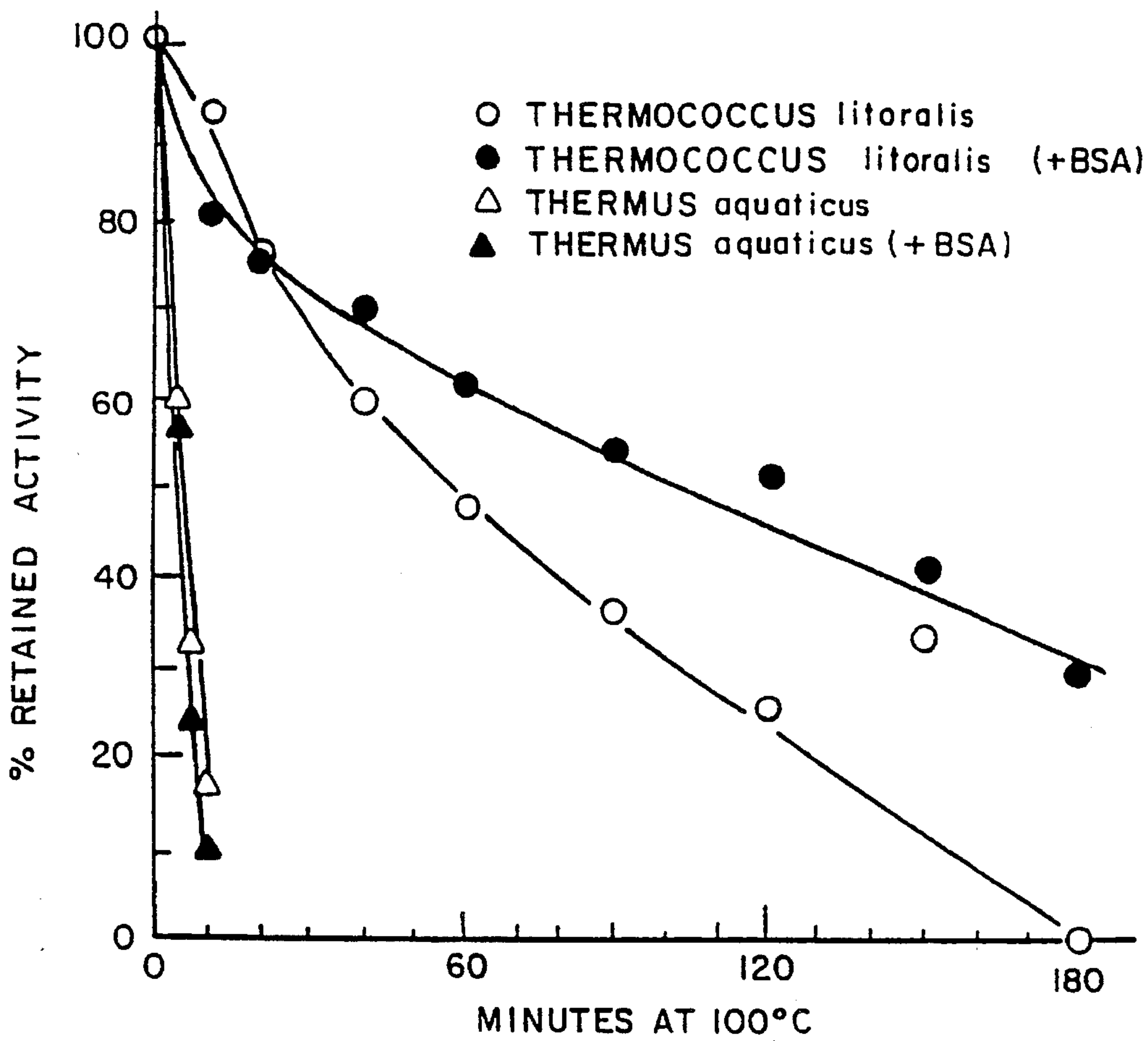
THERMAL STABILITIES OF DNA POLYMERASES
