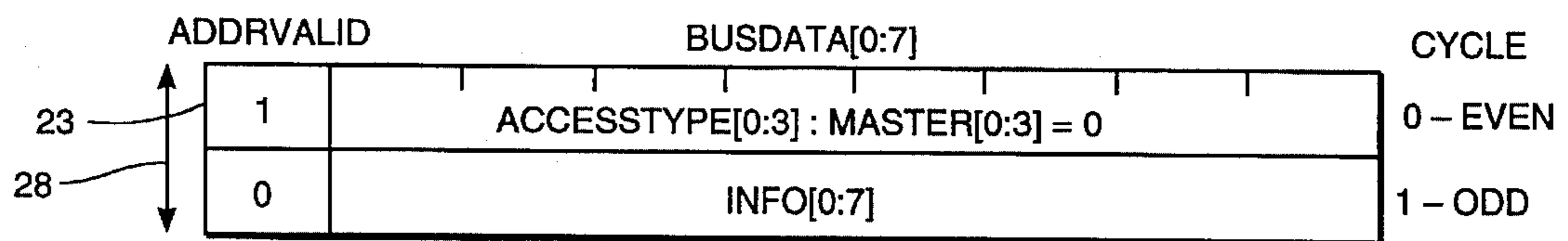
FIG 5 REJECT (NACK) CONTROL PACKET
