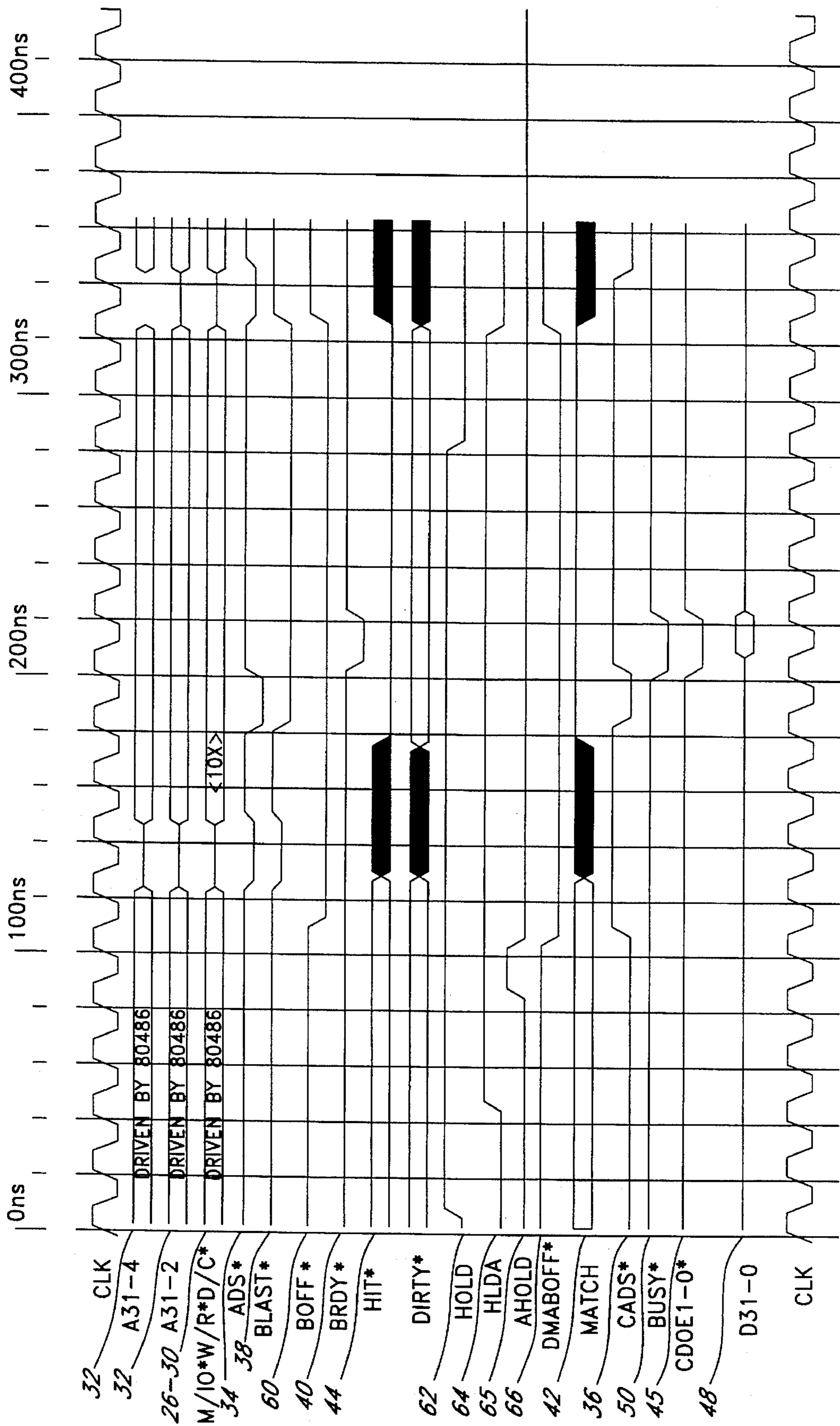
FIG. 6 DMA READ HIT
