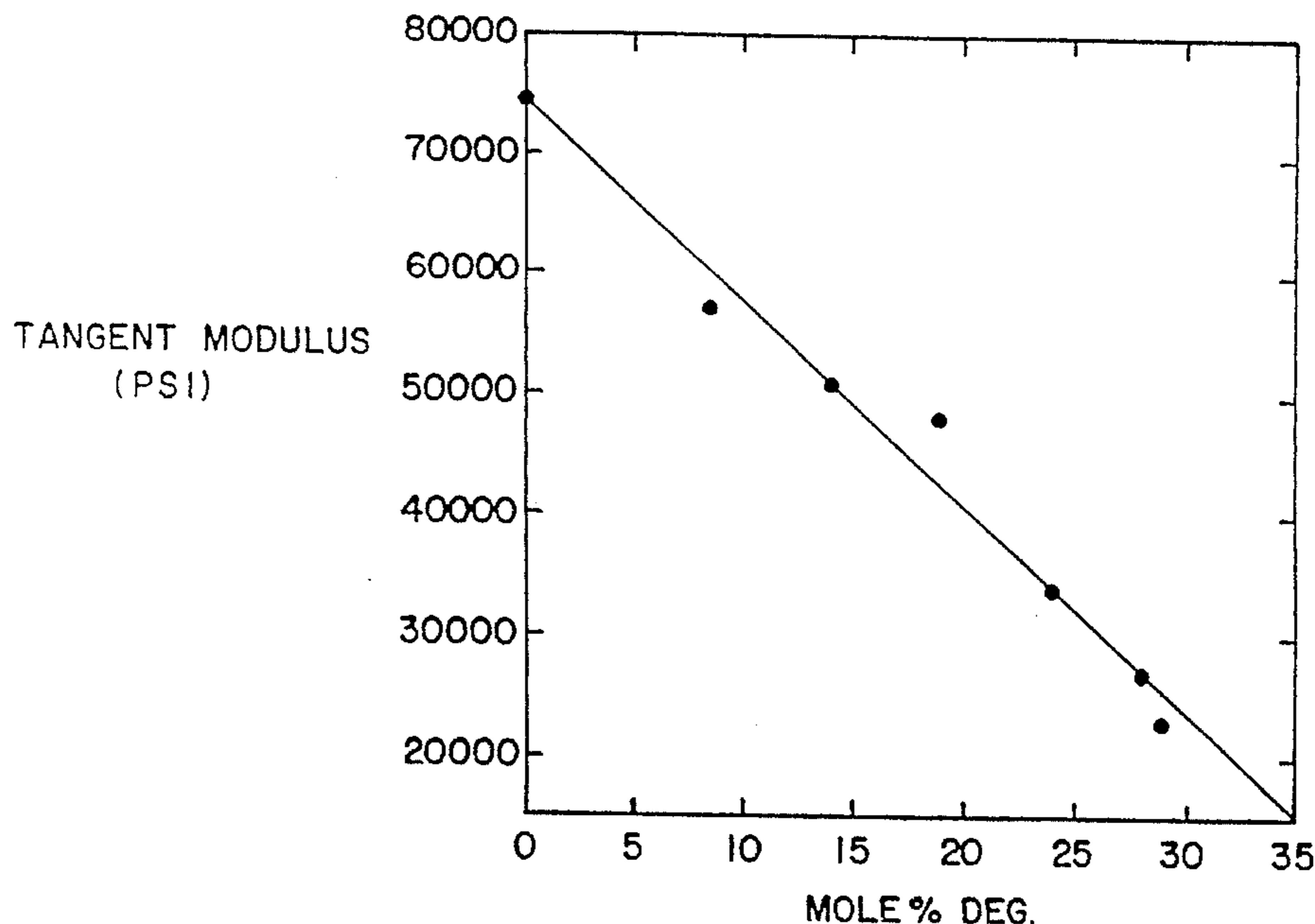
EFFECT OF MOLE % DEG ON THE TANGENT MODULUS OF SUCCINATE COPOLYESTERS
