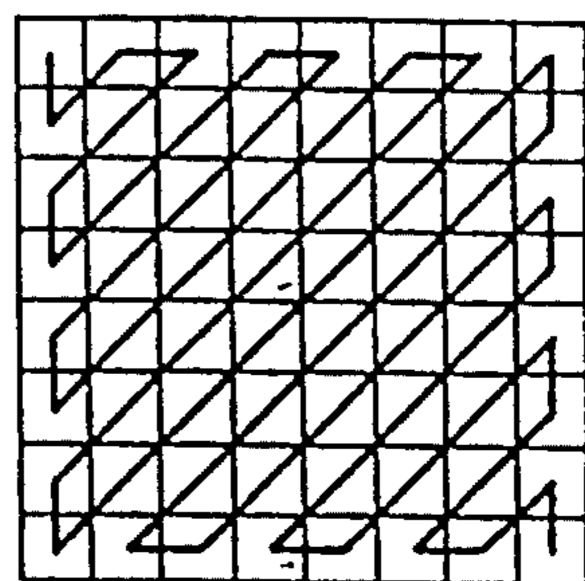
[RUN-LEVEL] CODING WITH ZIGZAG SCANNING PATTERN
