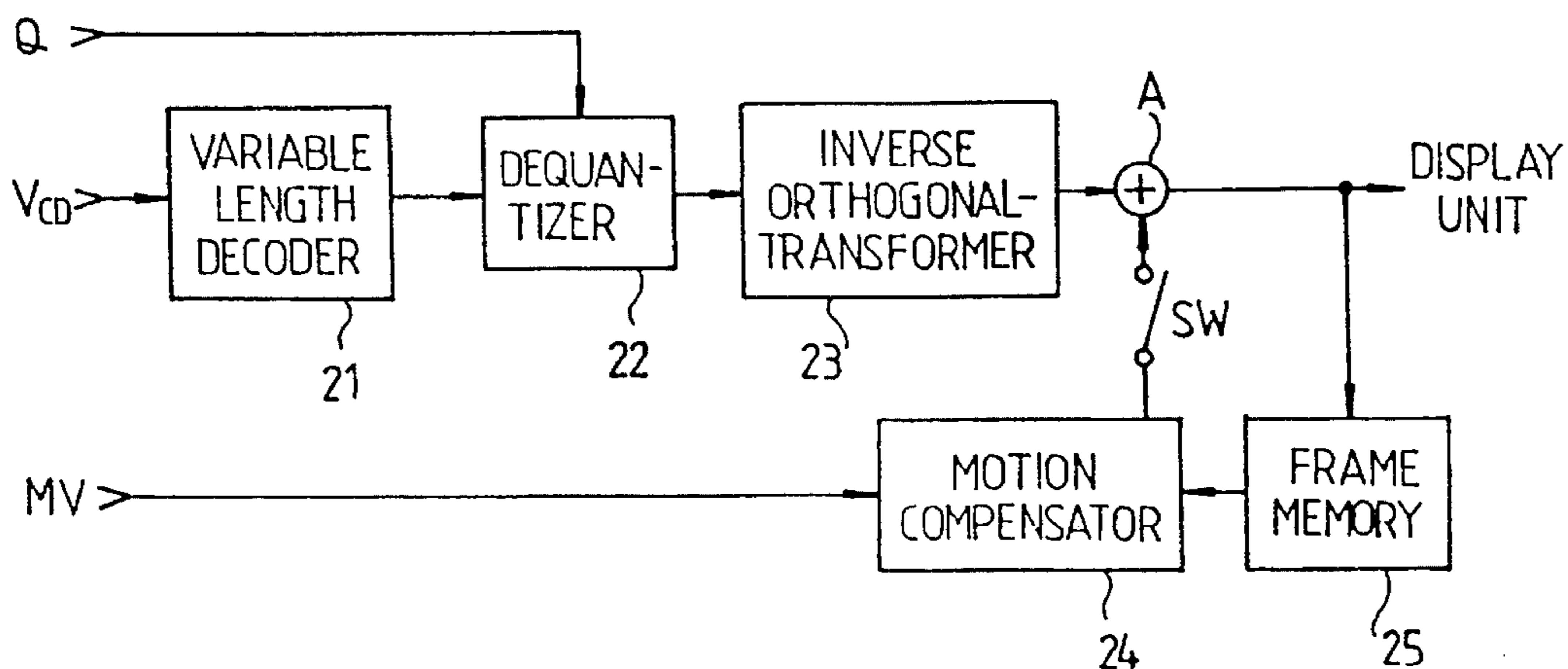
FIG. 2 (PRIOR ART)
