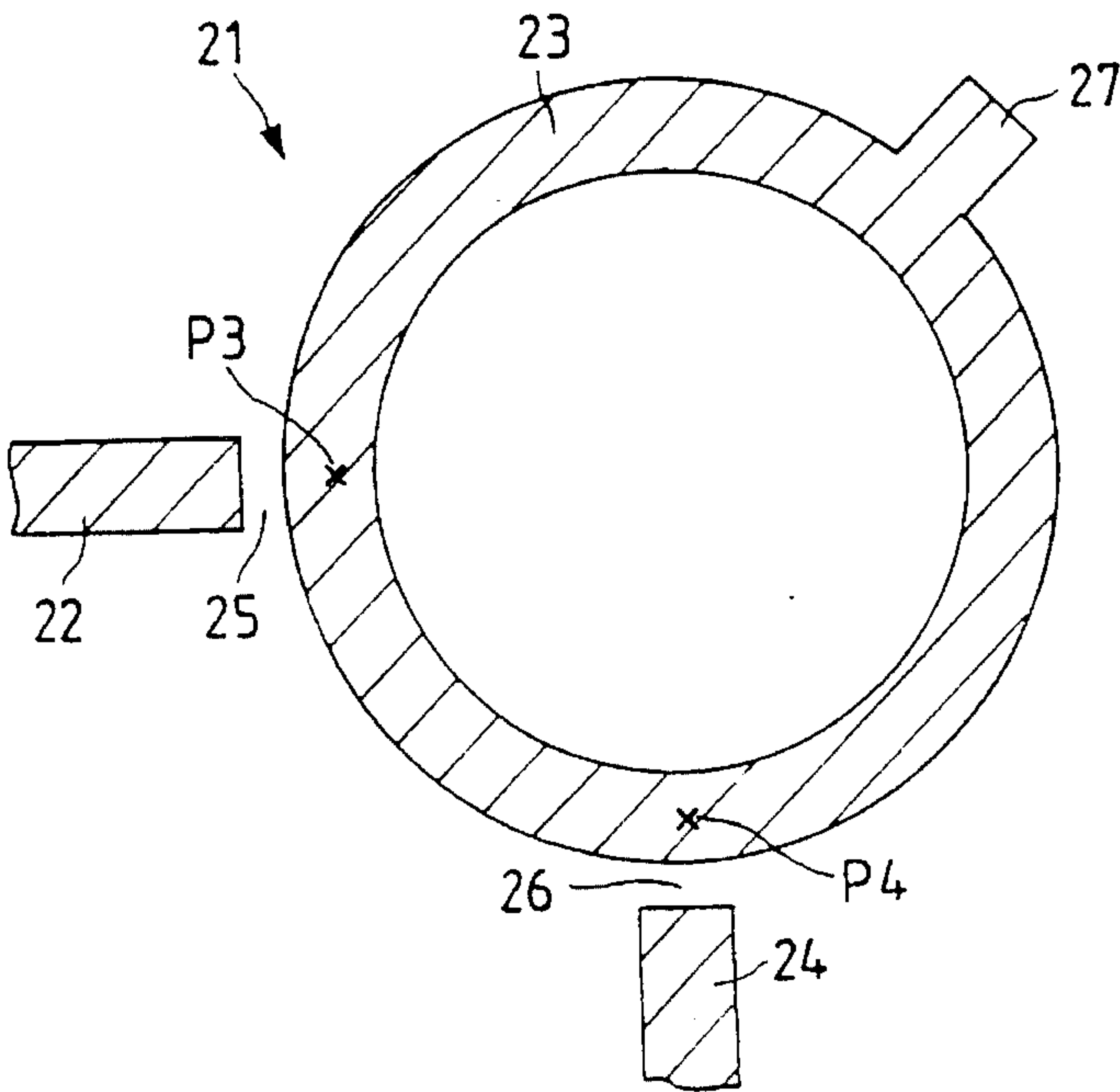
FIG. 2 PRIOR ART
