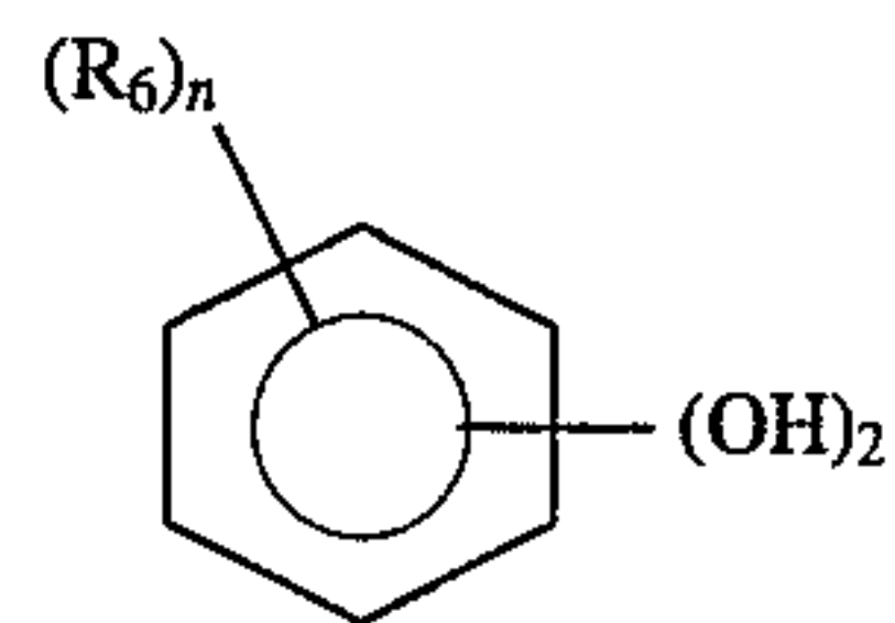
[Compound 4]
