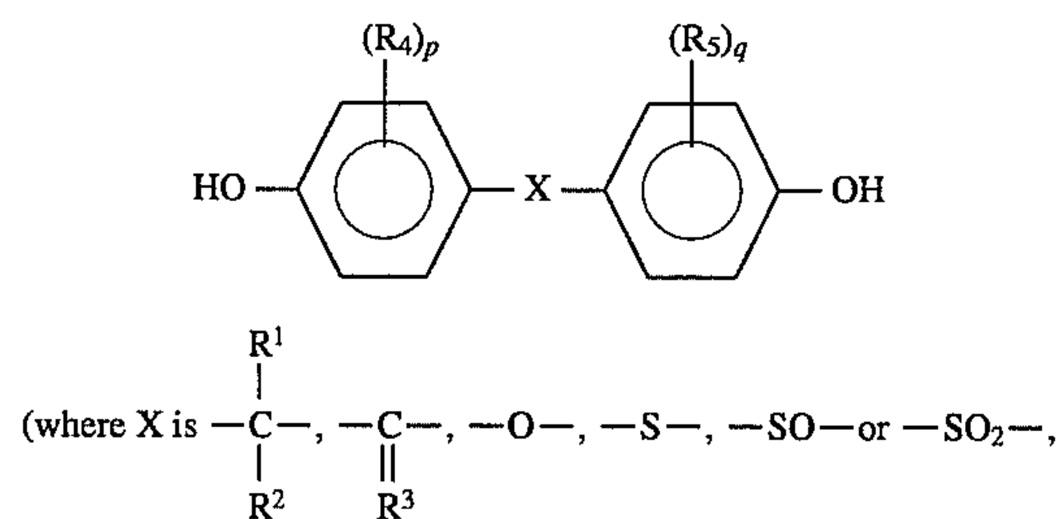
[Compound 3]
