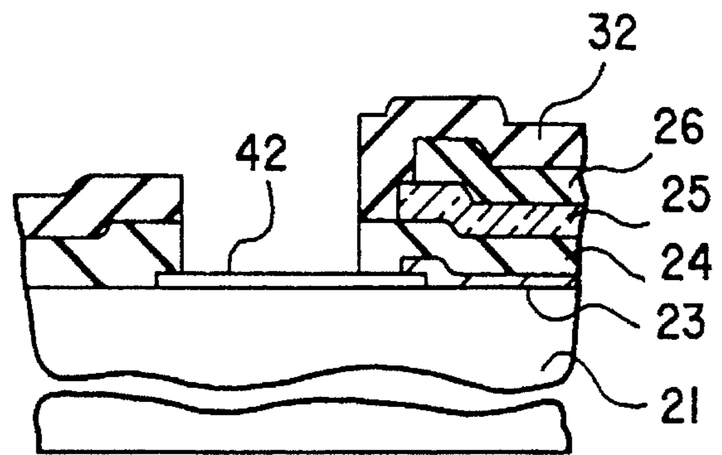
FIG.36B
