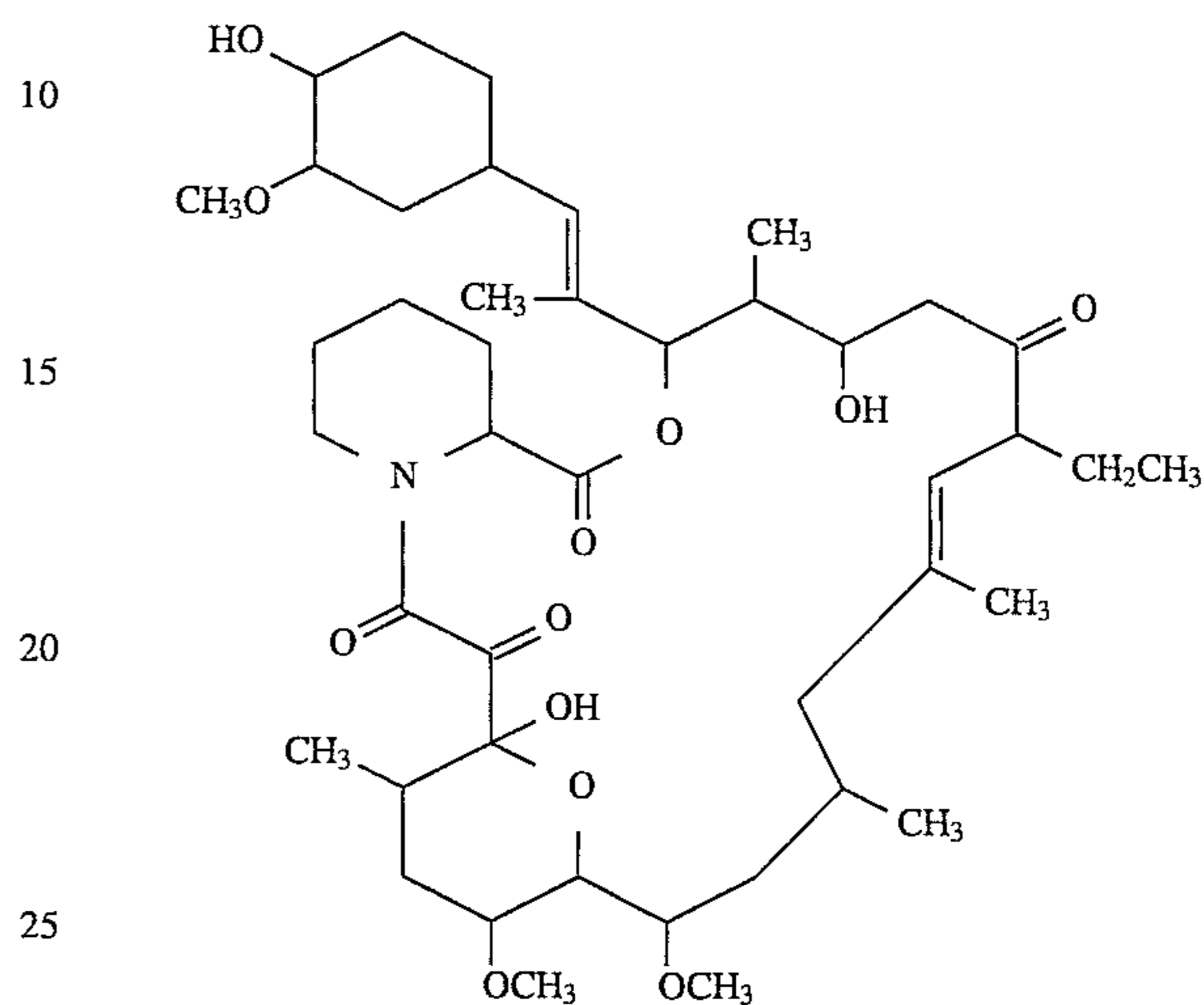
17-Ethyl-1,14-dihydroxy-12-[2-(4-hydroxy-3-methoxycyclohexyl)-1-methylvinyl]-23,25-dimethoxy-13,19,21,27-tetramethyl-11,28-dioxa-4-azatricyclo-[22.3.1.0 4,9 ]octacos-18-ene-2,3,10,16-tetraone FR-900523 Substance
