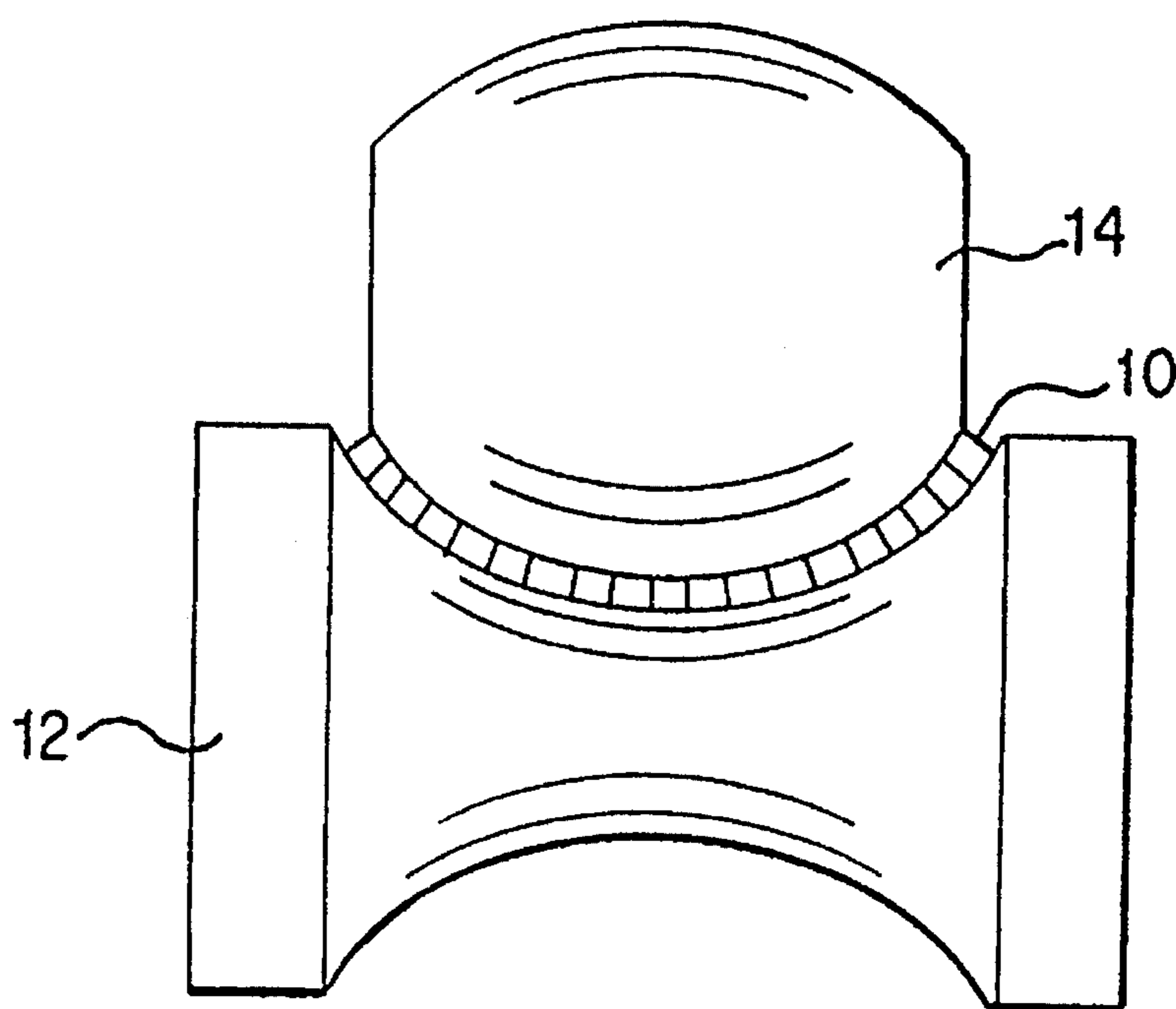
FIG. 2 PRIOR ART
