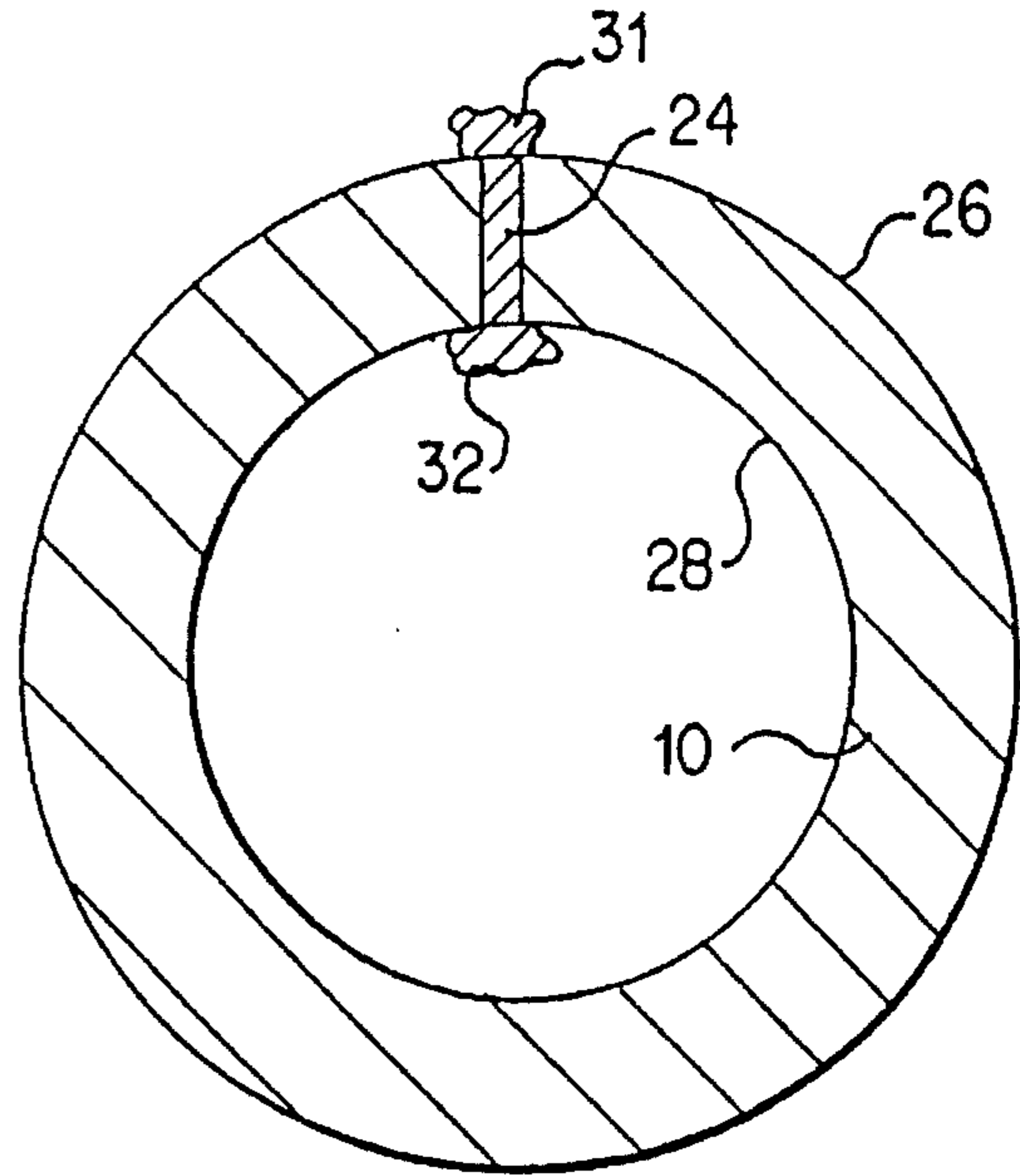
FIG. 6 PRIOR ART
