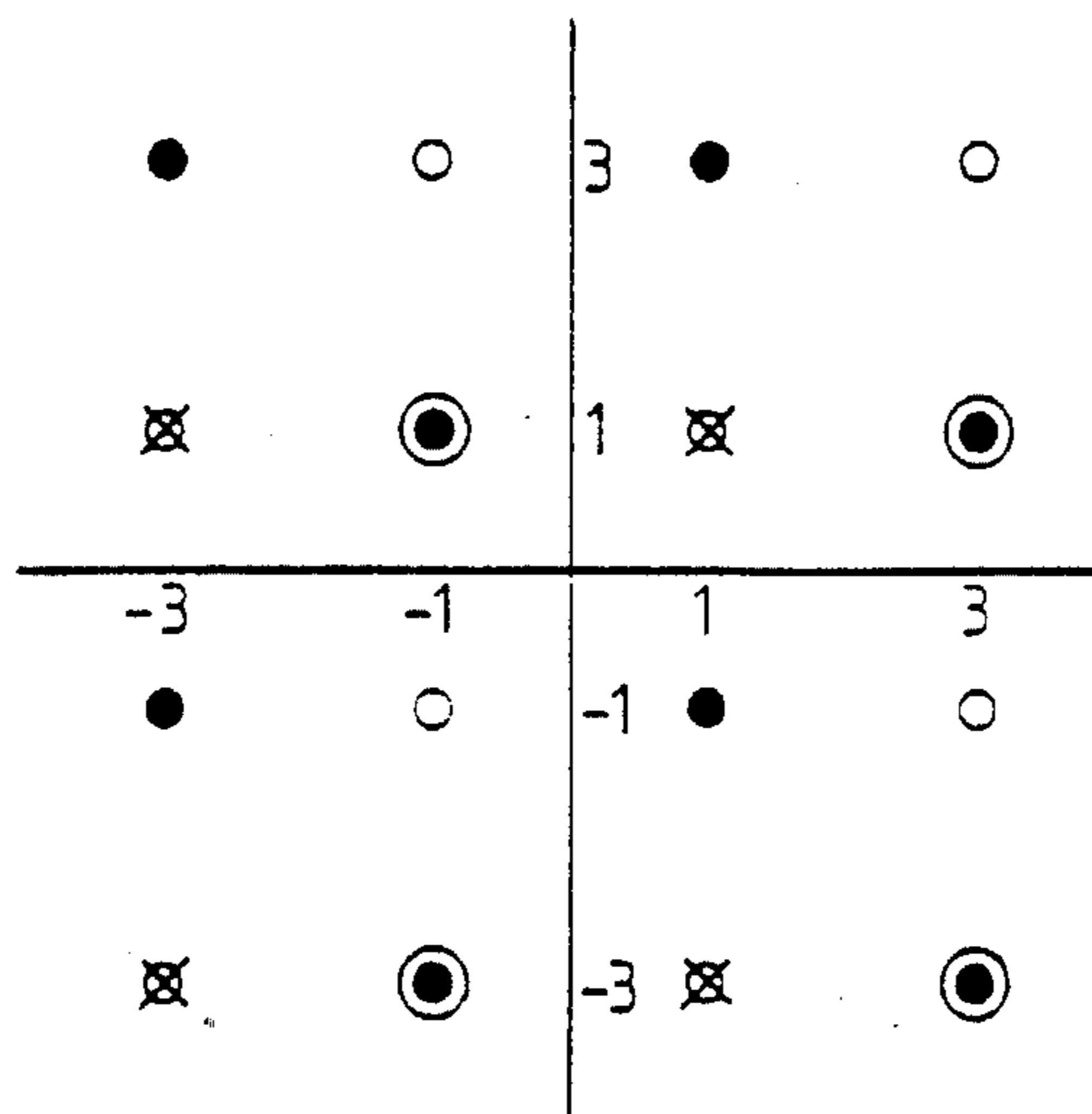
16 POINT SIGNAL CONSTELLATION
