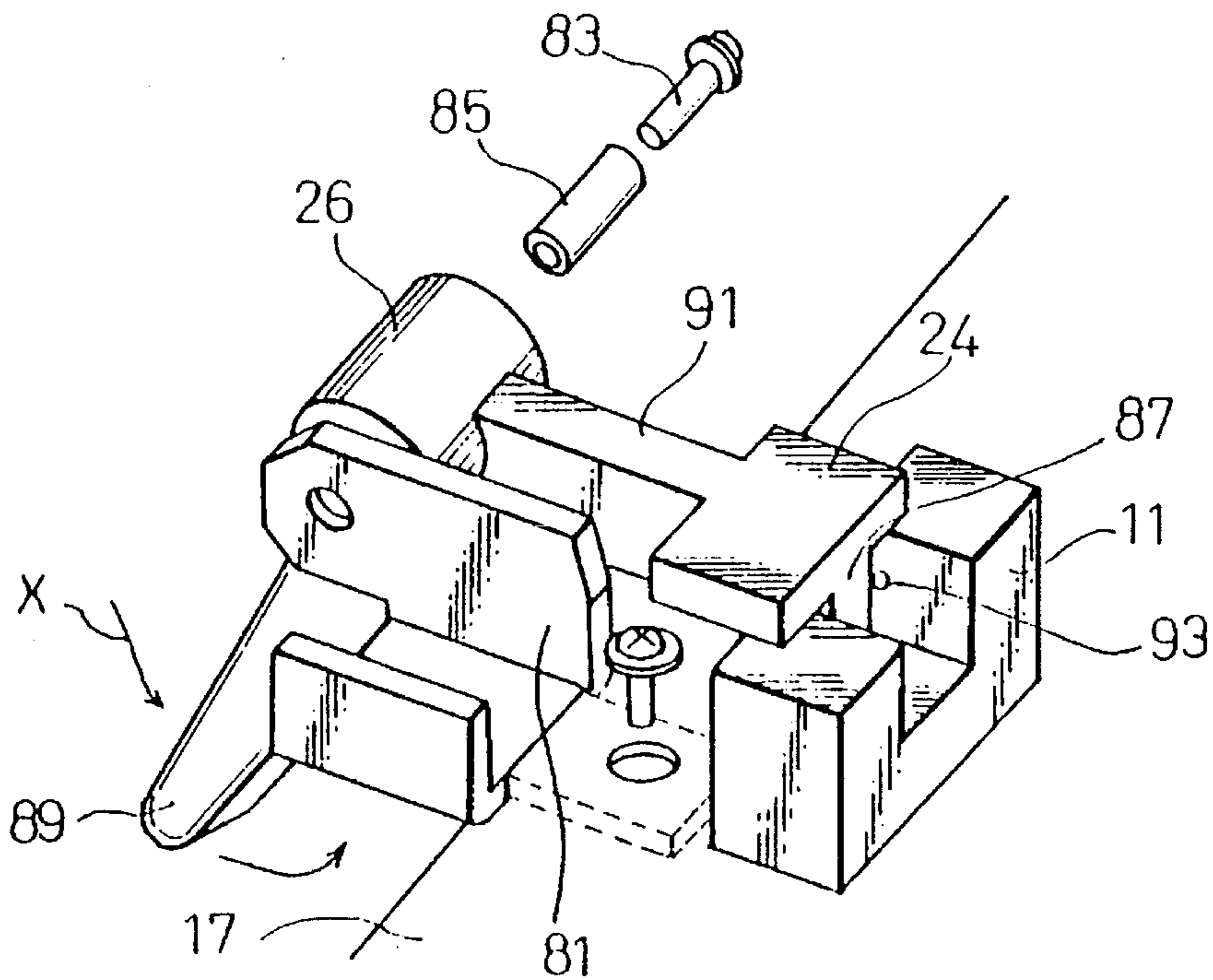
Fig. 46 (PRIOR ART)
