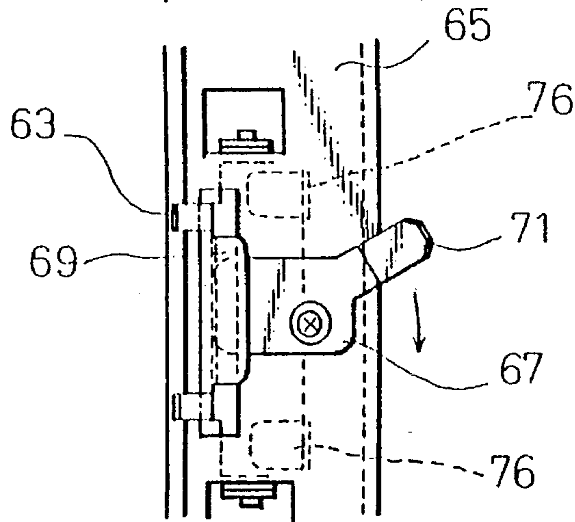
Fig. 45 (PRIOR ART)
