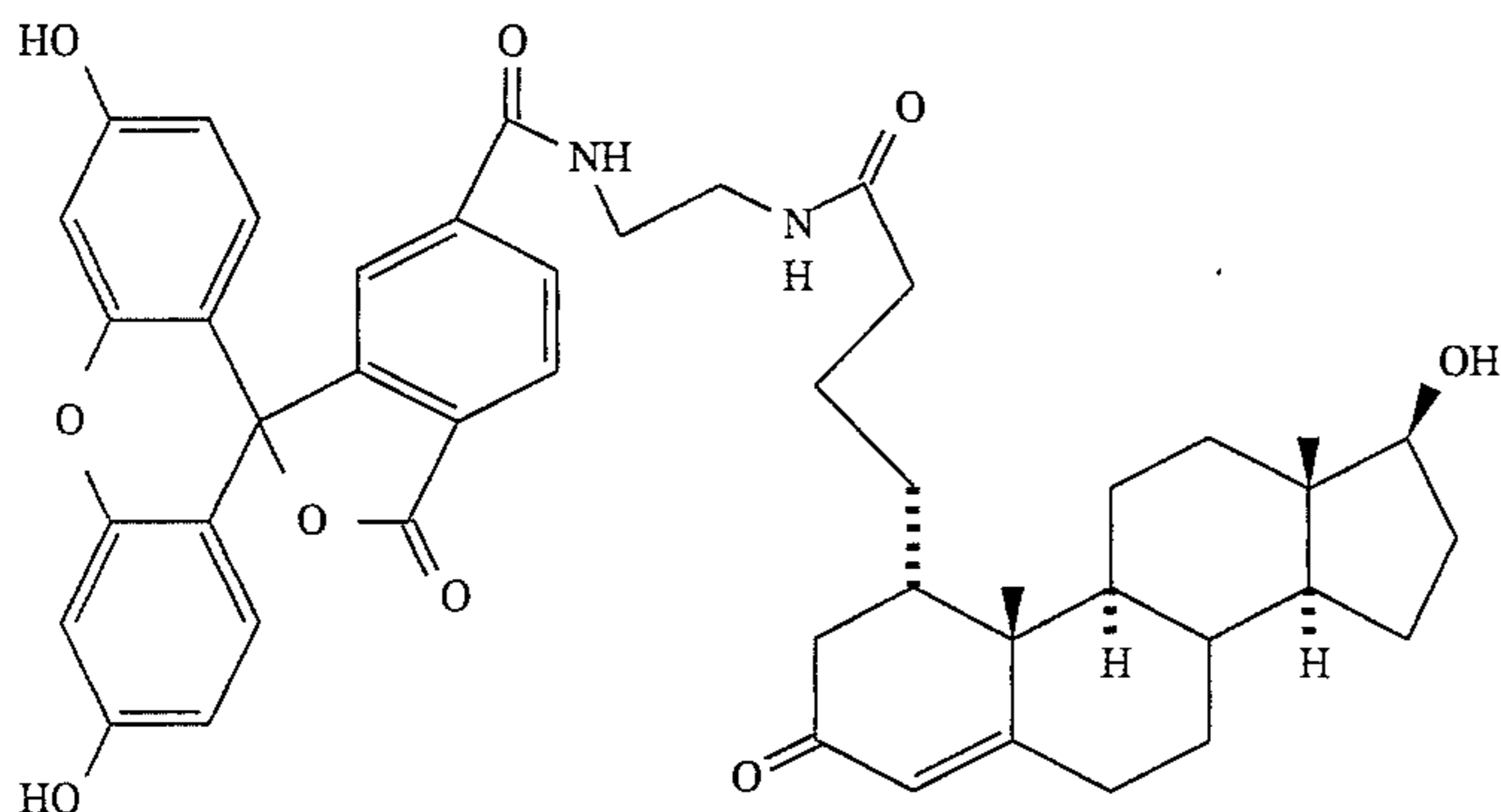
FORMULA 3 STRUCTURE OF THE PREFERRED FLUORESCIN-LABELED TESTOSTERONE REAGENT
