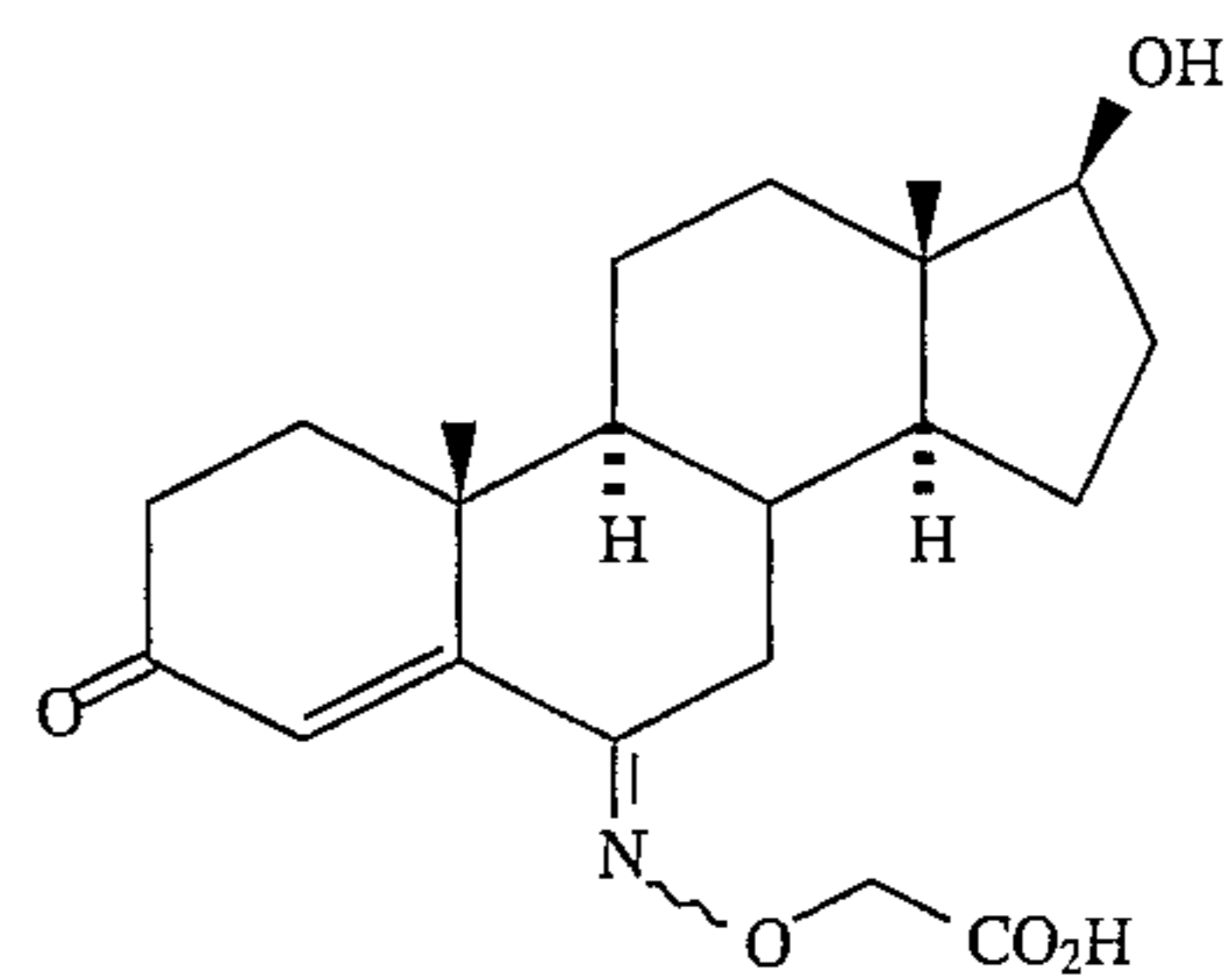
6-(O-carboxymethyl)-oxime testosterone
