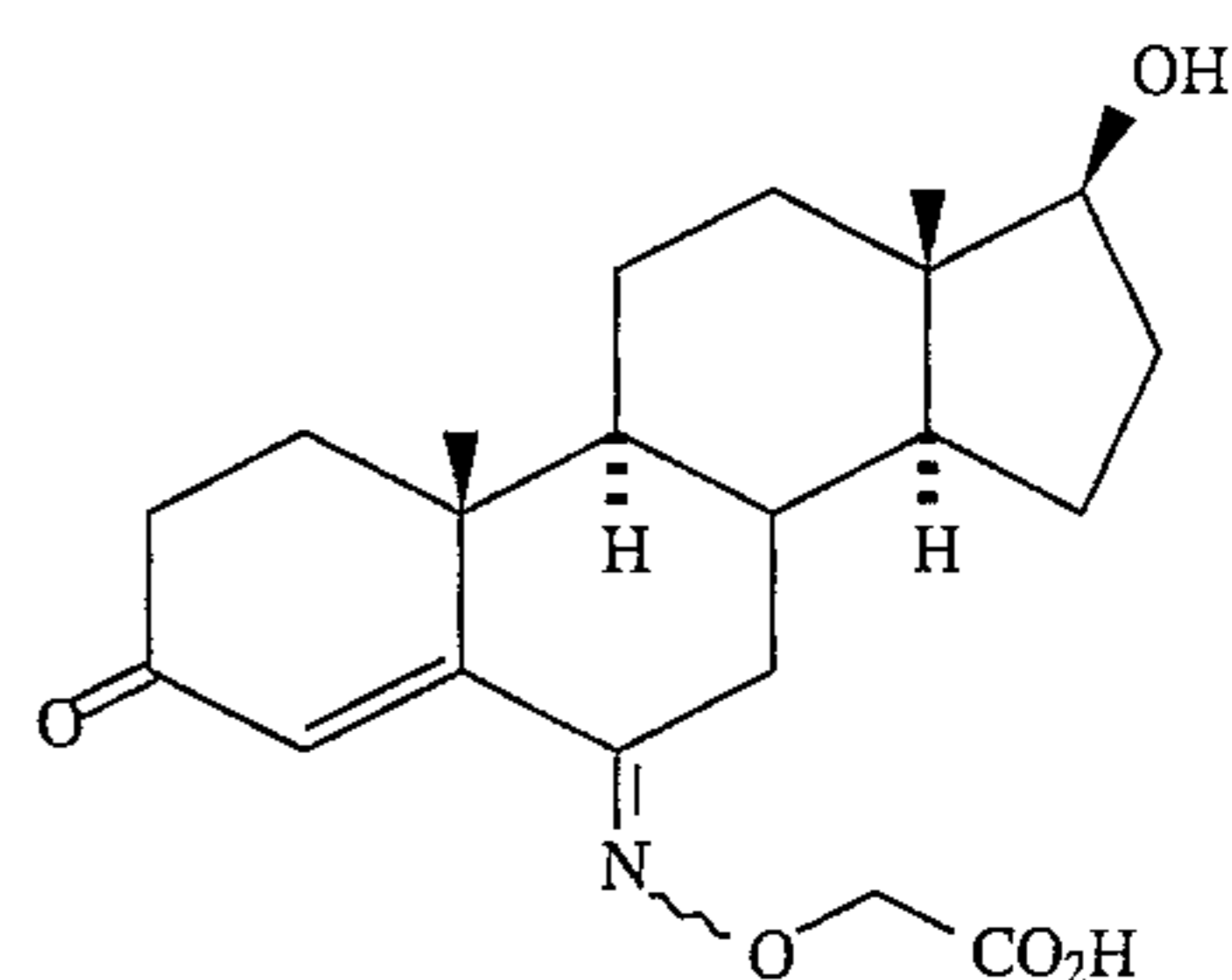
6-(O-carboxymethyl)-oxime testosterone
