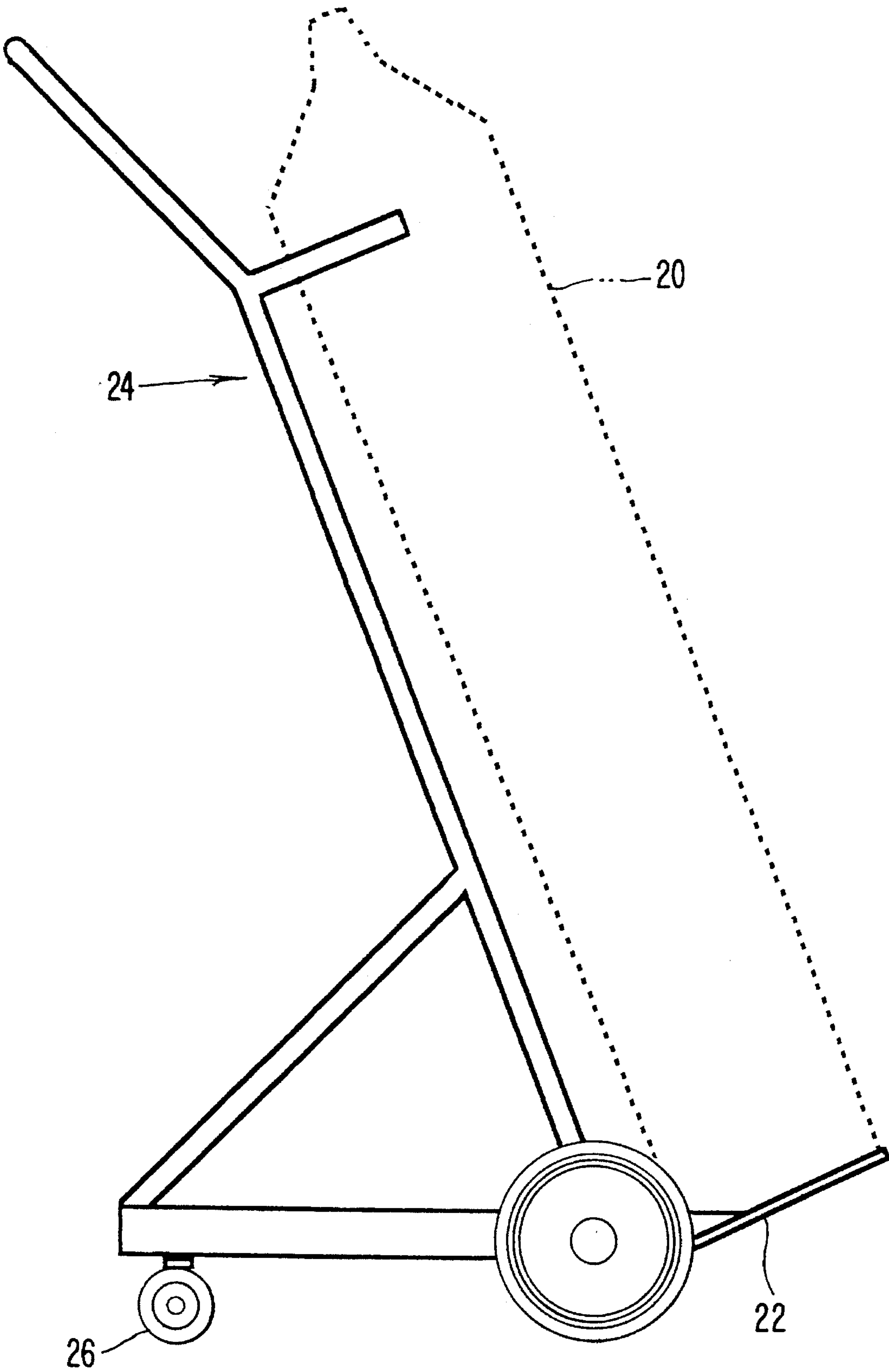
FIG. 2 PRIOR ART
