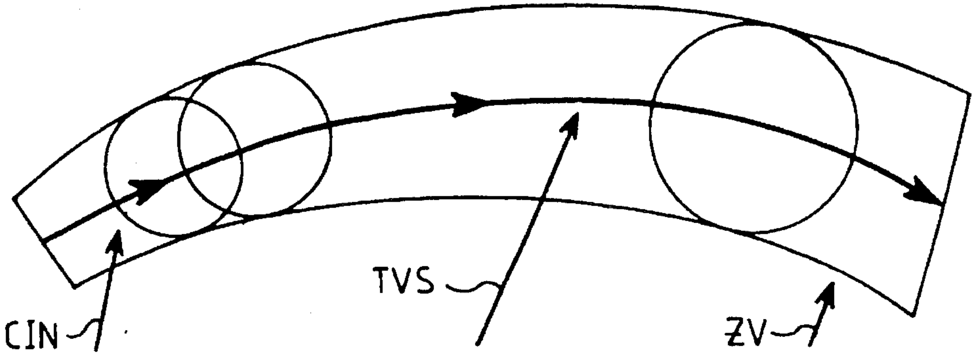
FIG.14 - UNCERTAINTY LINKED TO THE FLIGHT PATH OF THE AIRCRAFT (PROJECTION IN THE HORIZONTAL PLANE)
