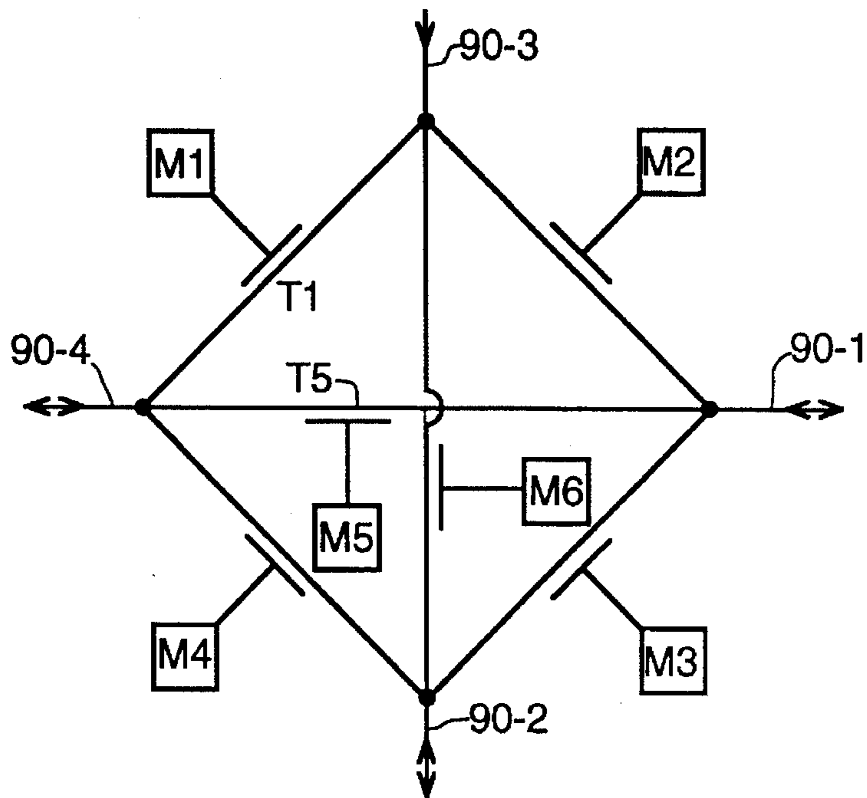
FIG. 2c (PRIOR ART)
