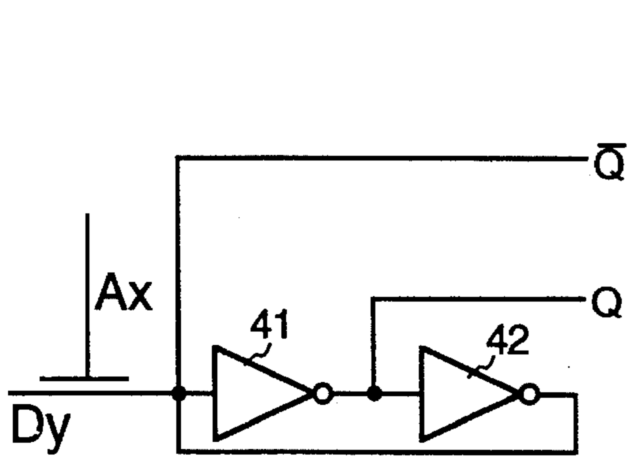
FIG. 4 (PRIOR ART)
