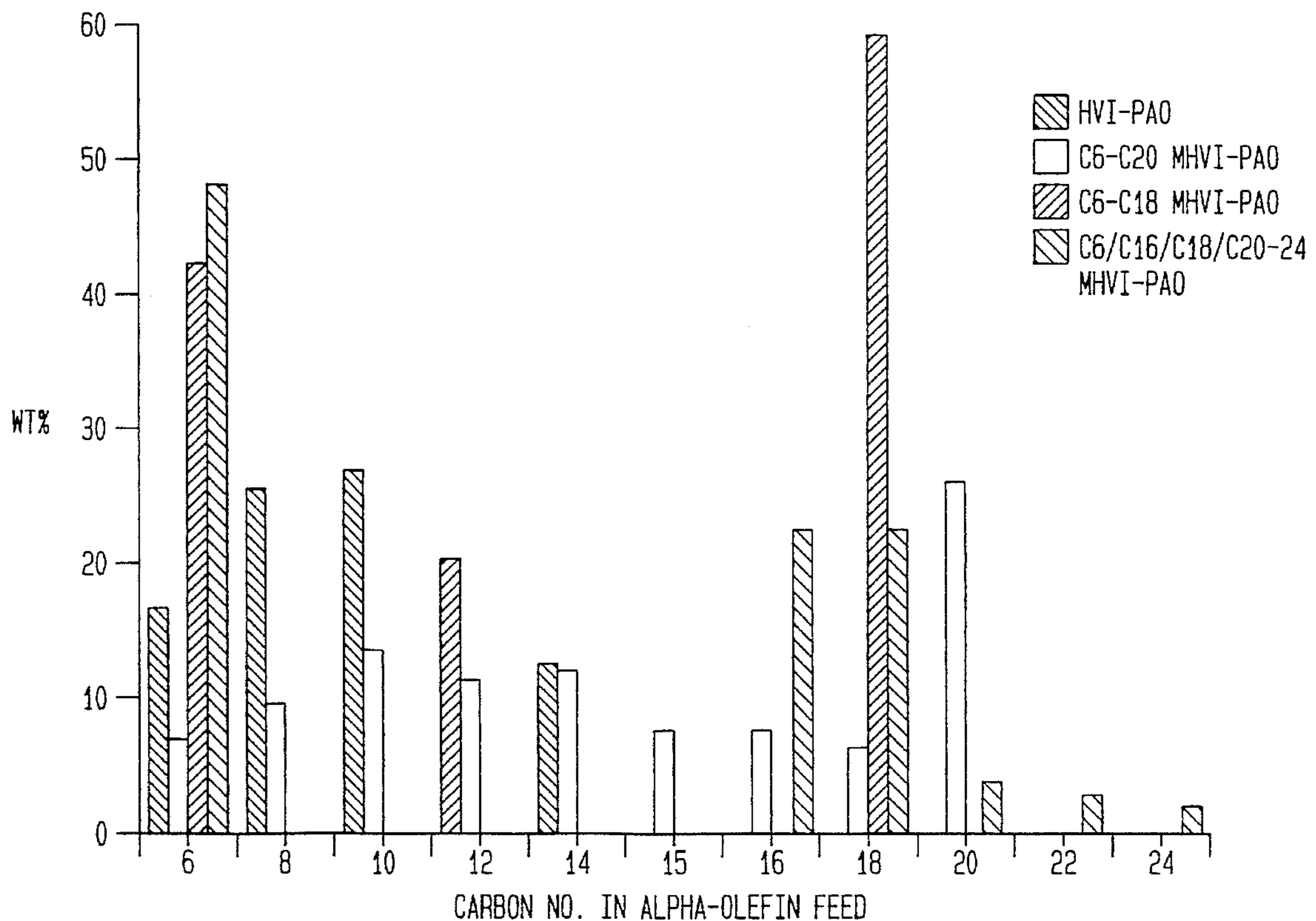
FEED COMPOSITIONS FOR HVI-PAO VS. MIXED HVI-PAO
