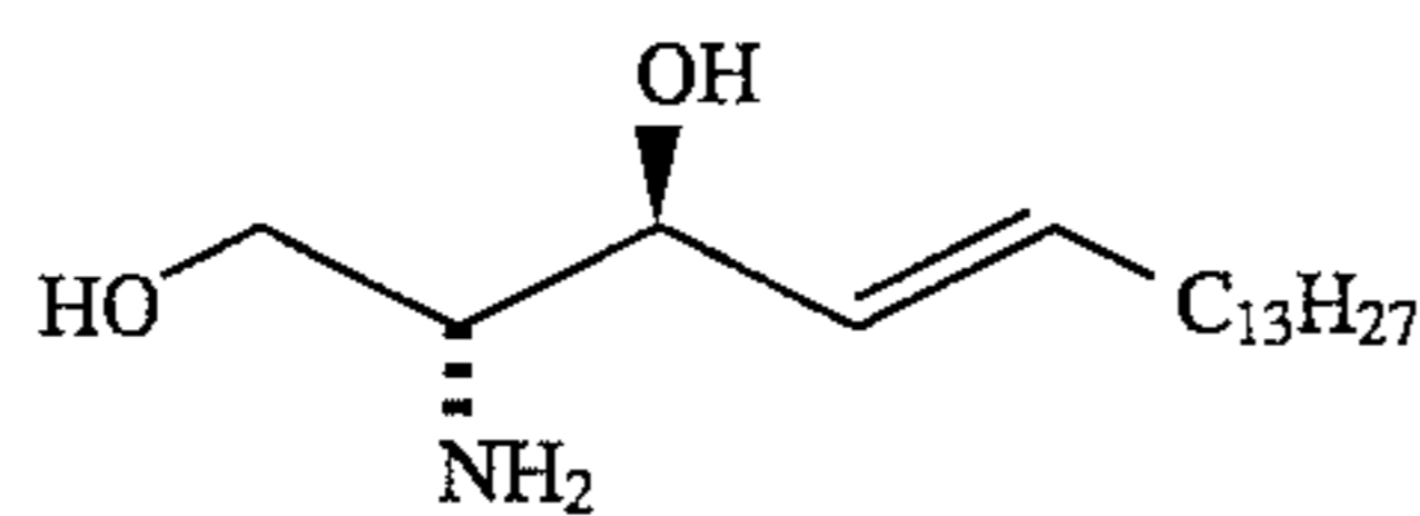
L-erythro-sphingosine (3)
