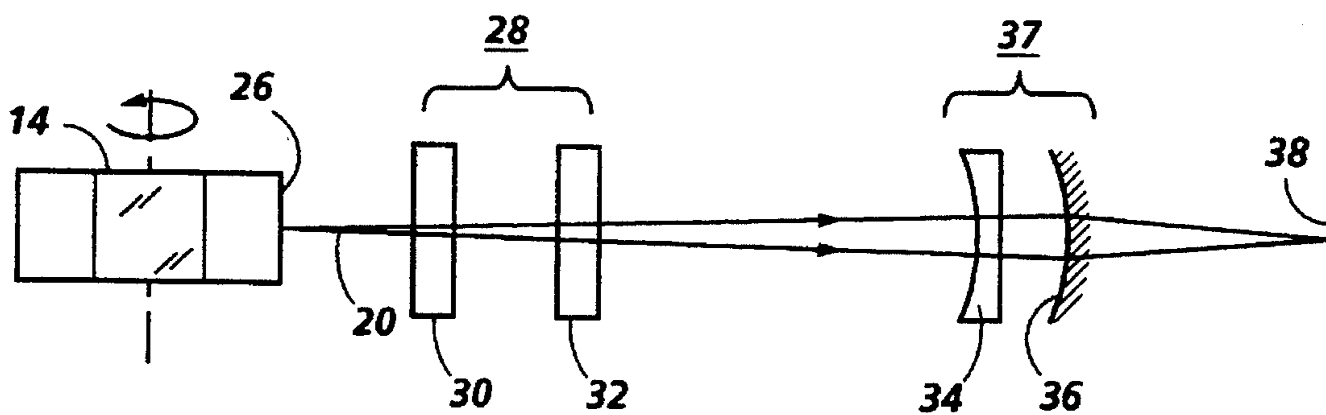
FIG. 3 PRIOR ART
