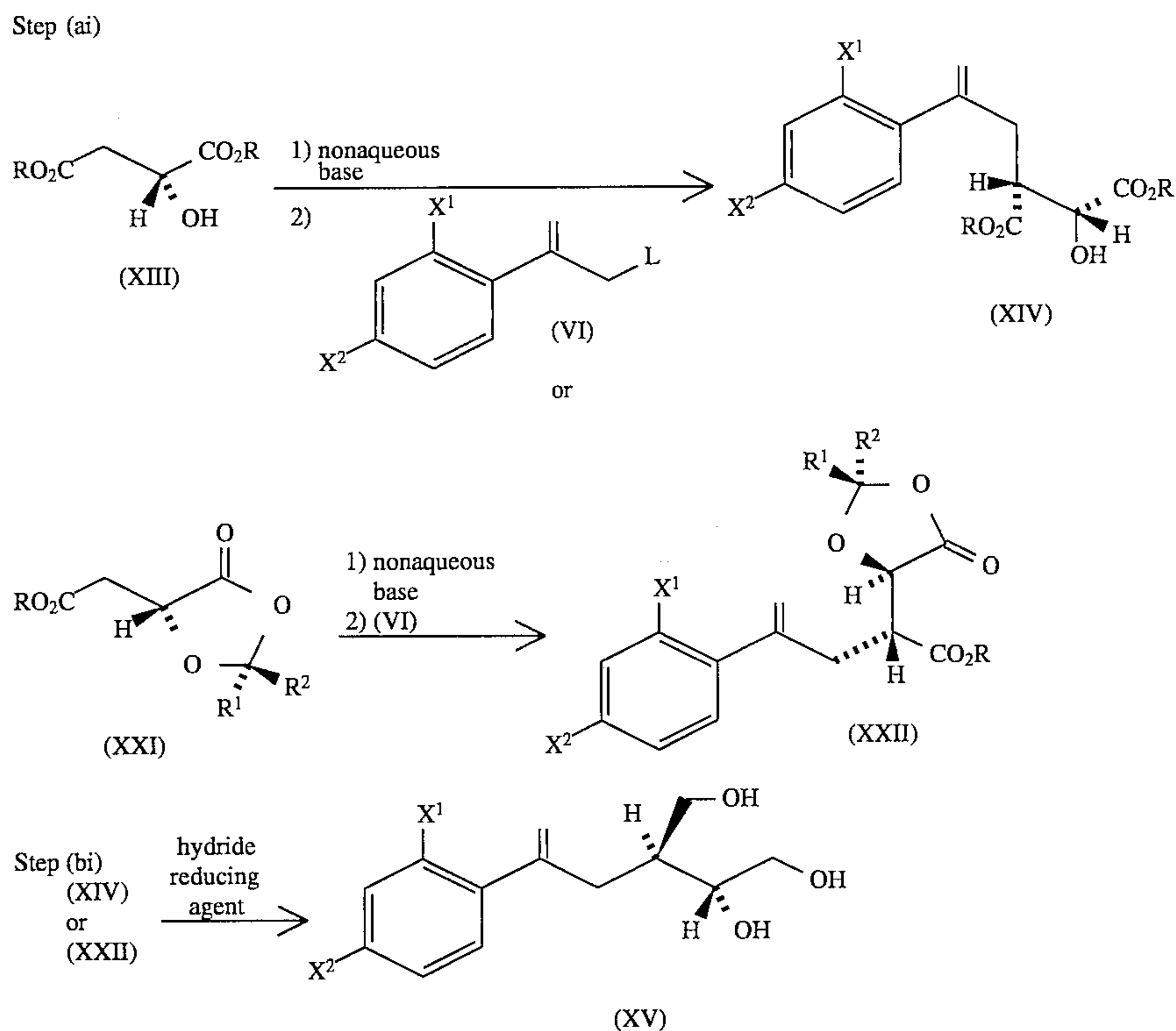
Reaction Scheme 2
