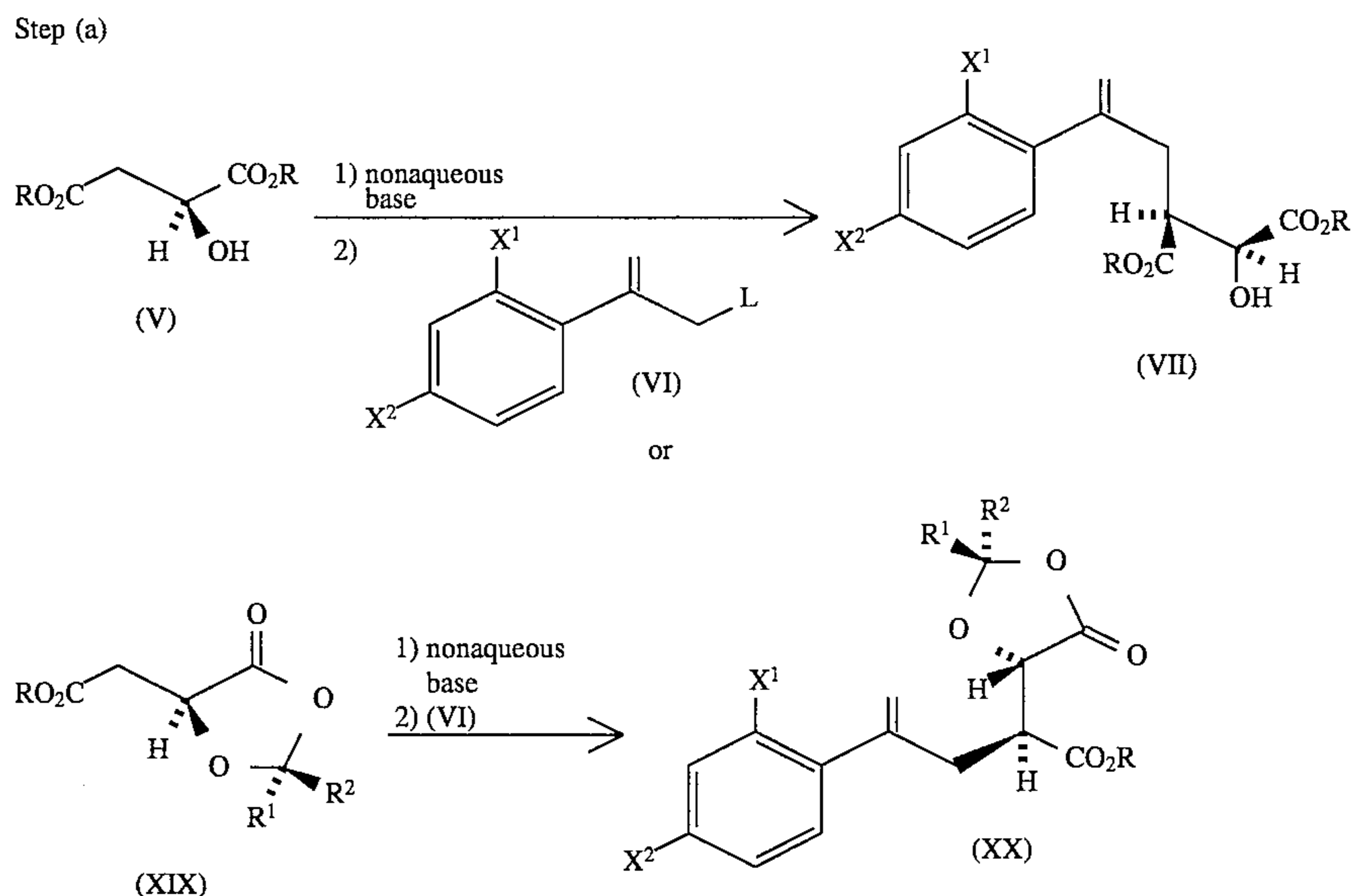
Reaction Scheme 1
