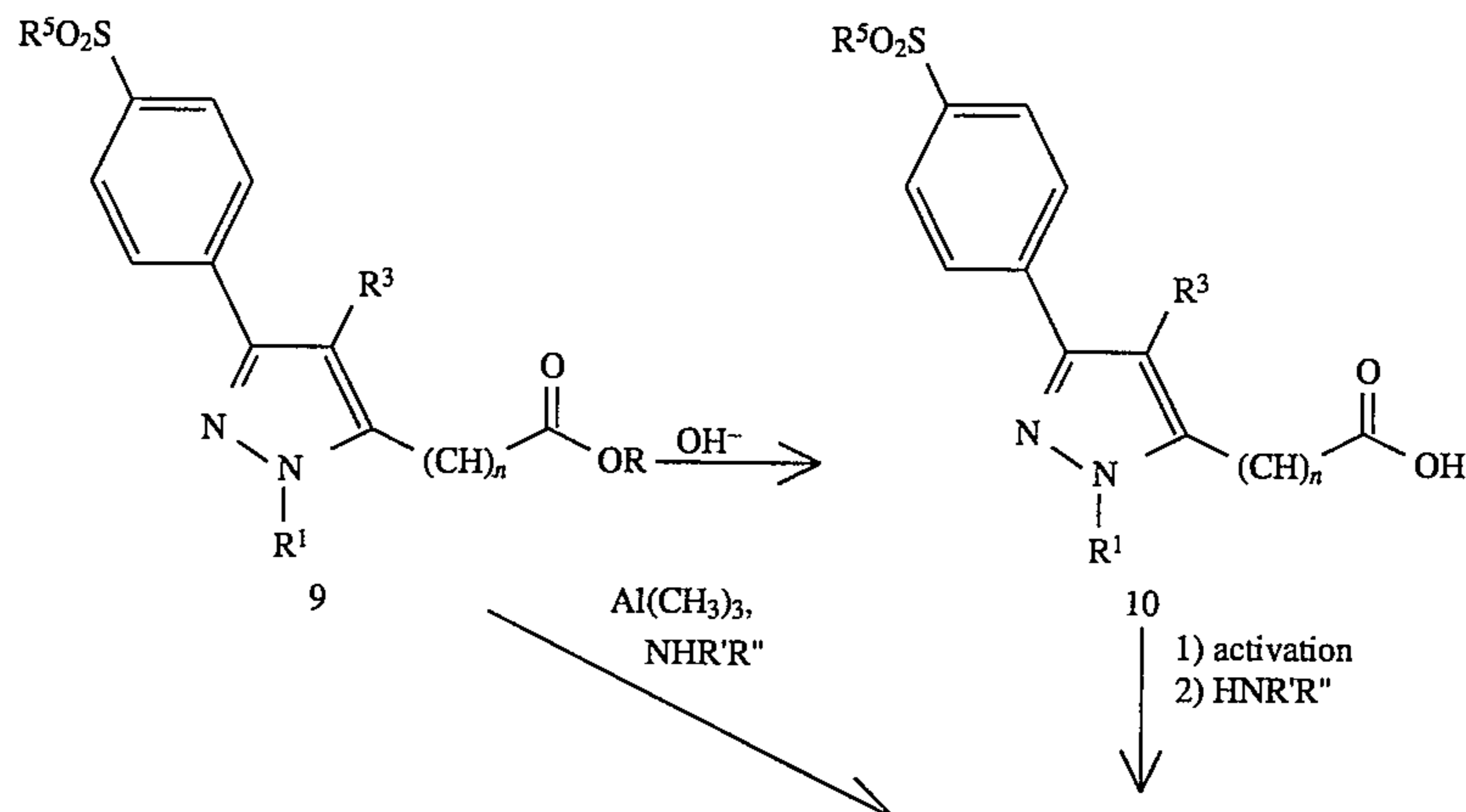
Scheme V
