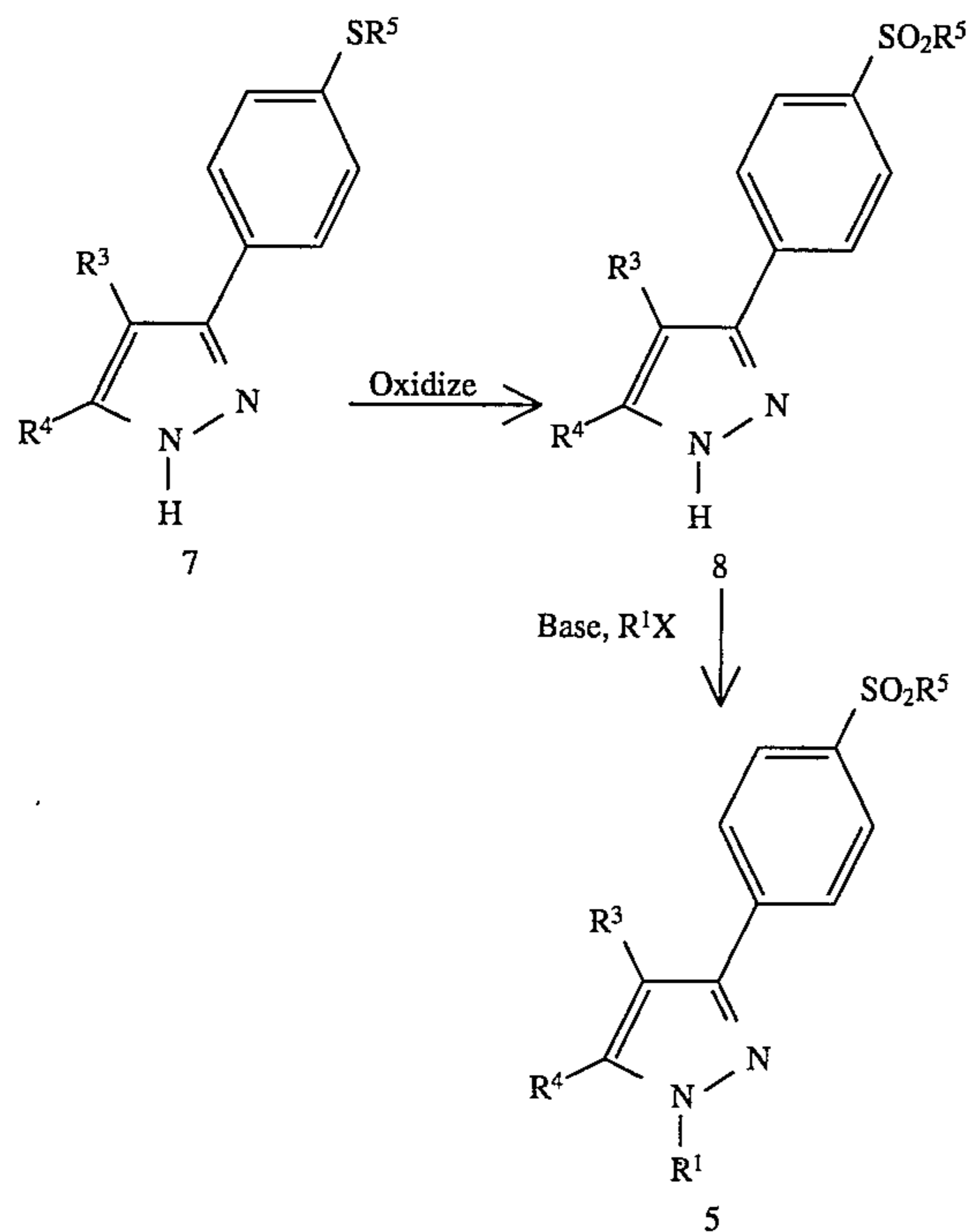
Scheme IV
