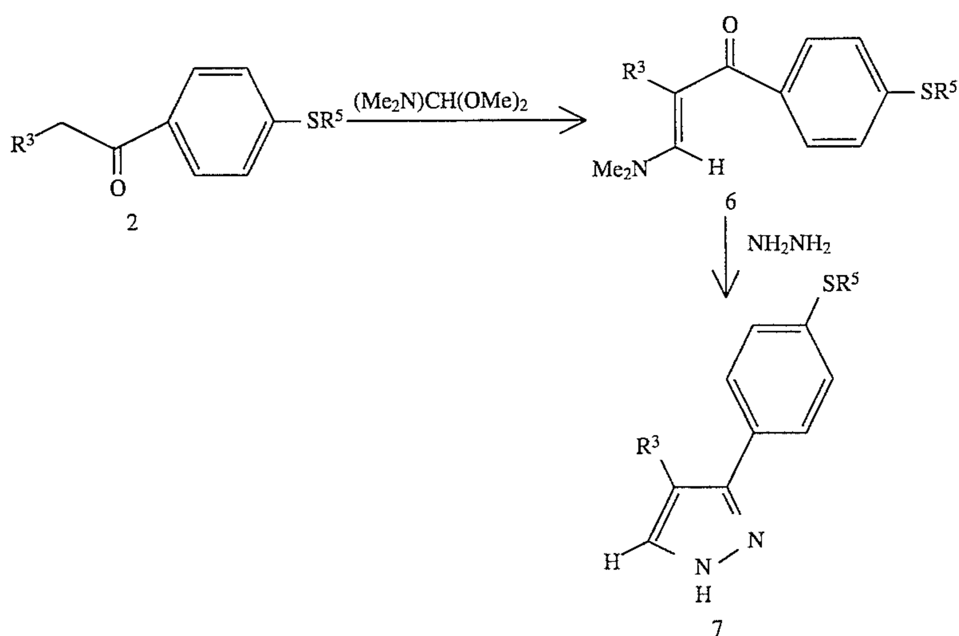
Scheme III
