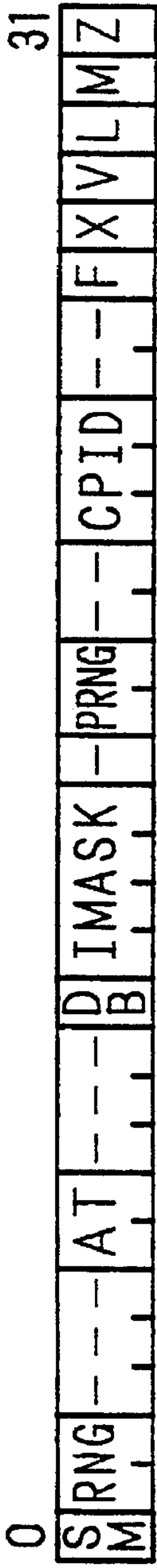
Fig. 45(a) PSW( processor status word)
