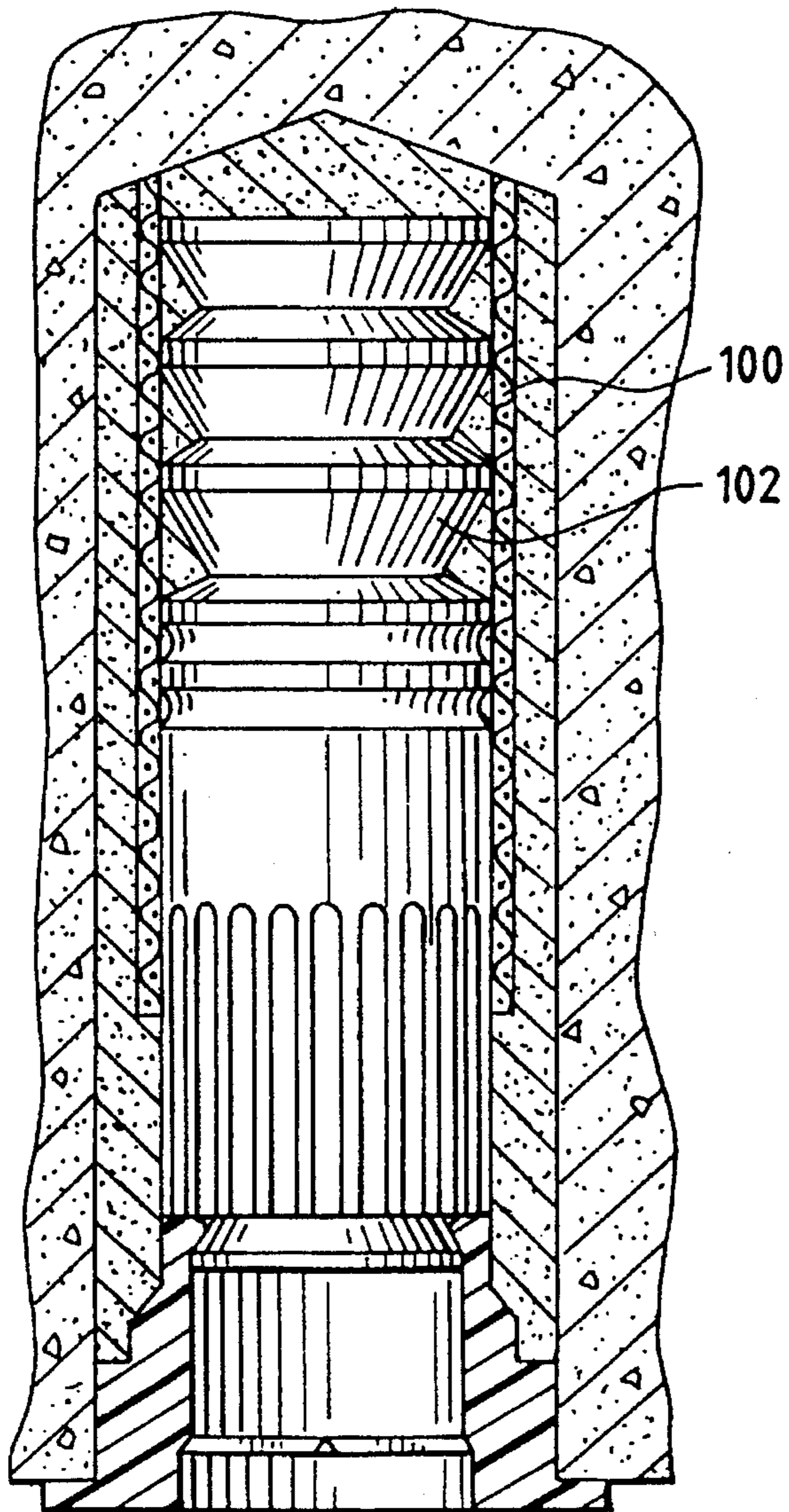
FIG. 6 PRIOR ART
