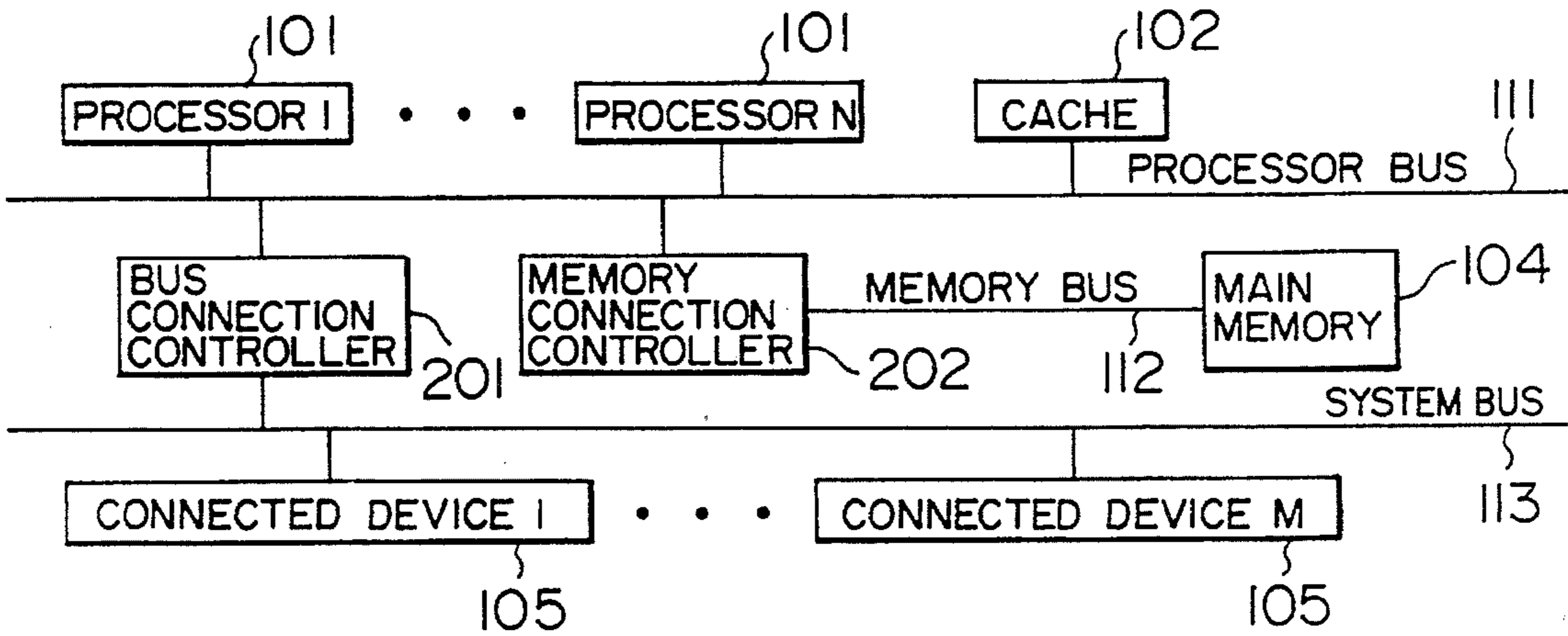
FIG. 3 PRIOR ART
