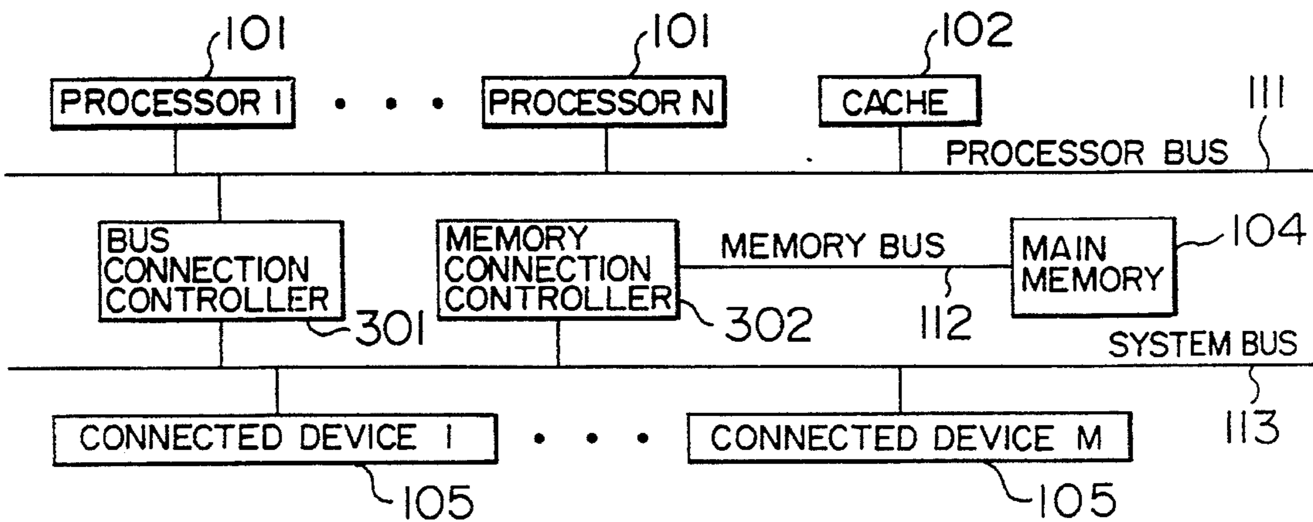
FIG. 3 PRIOR ART
