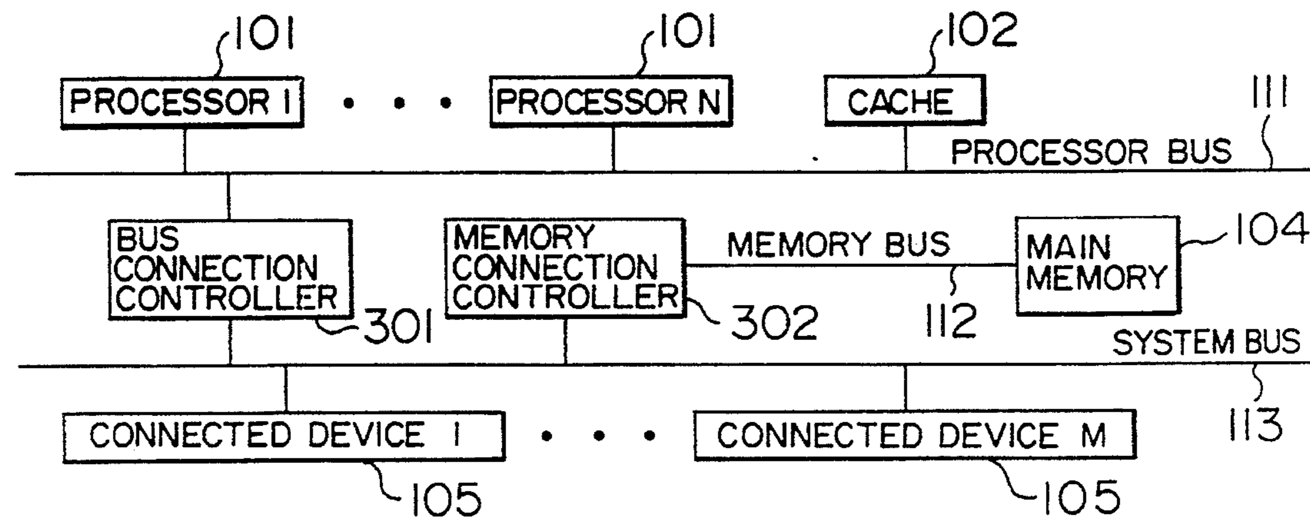
FIG. 3 PRIOR ART
