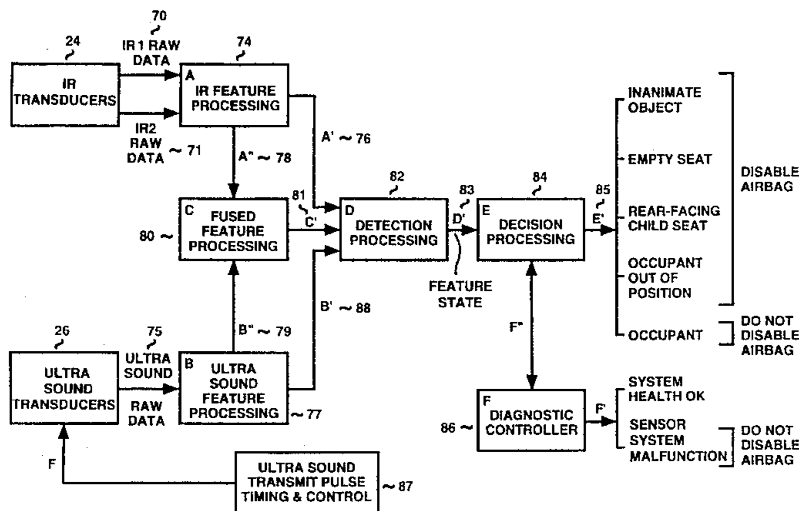
SIGNAL PROCESSOR FUNCTIONAL BLOCK DIAGRAM
