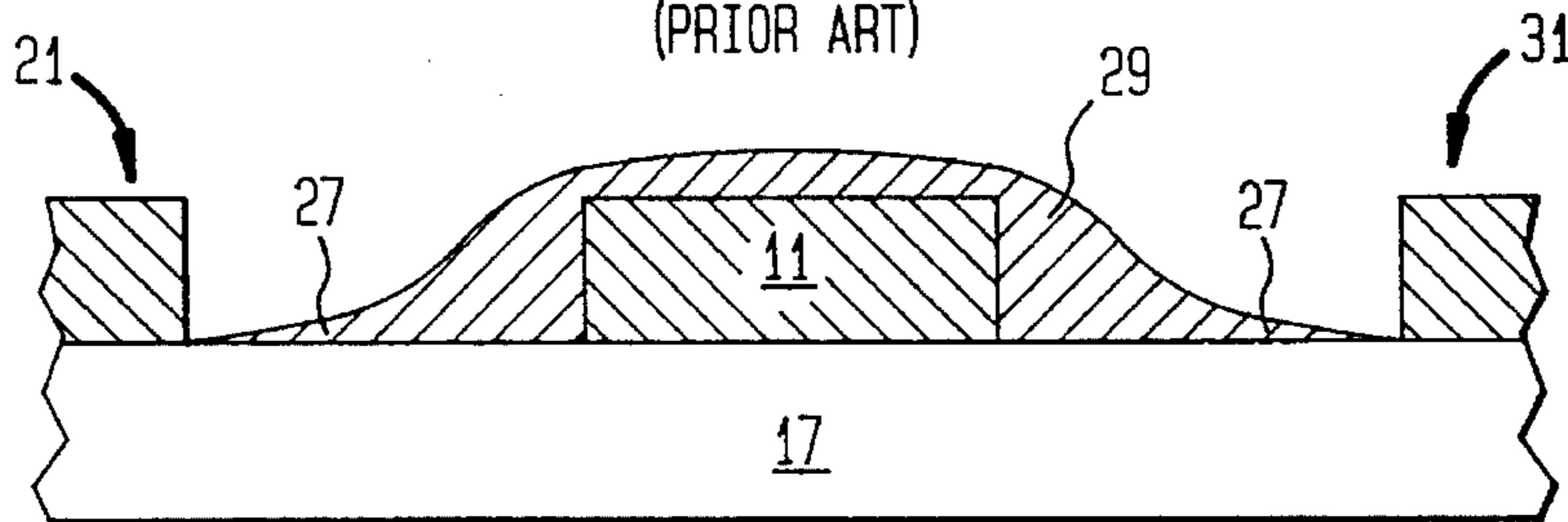
FIG. 2C (PRIOR ART)
