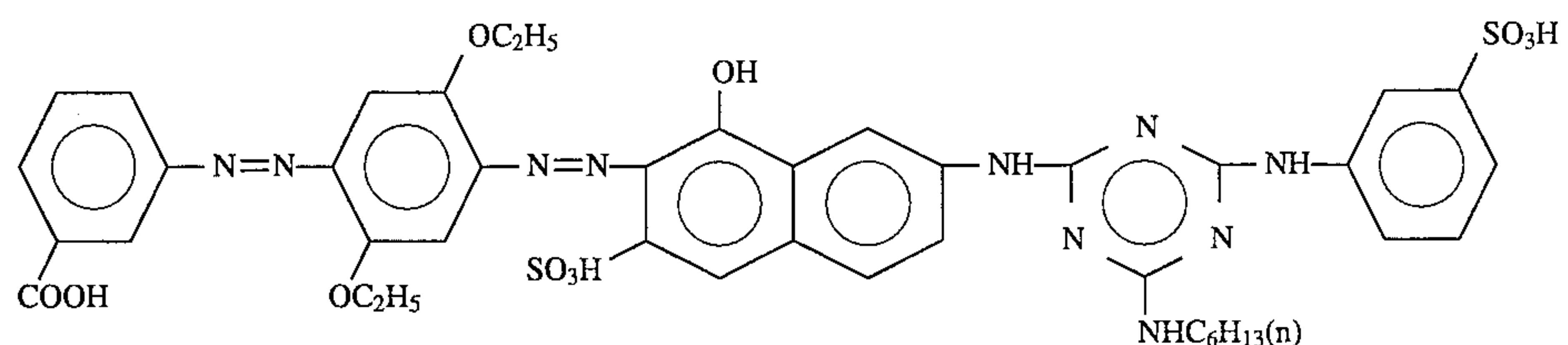
Structural Formula (3):
