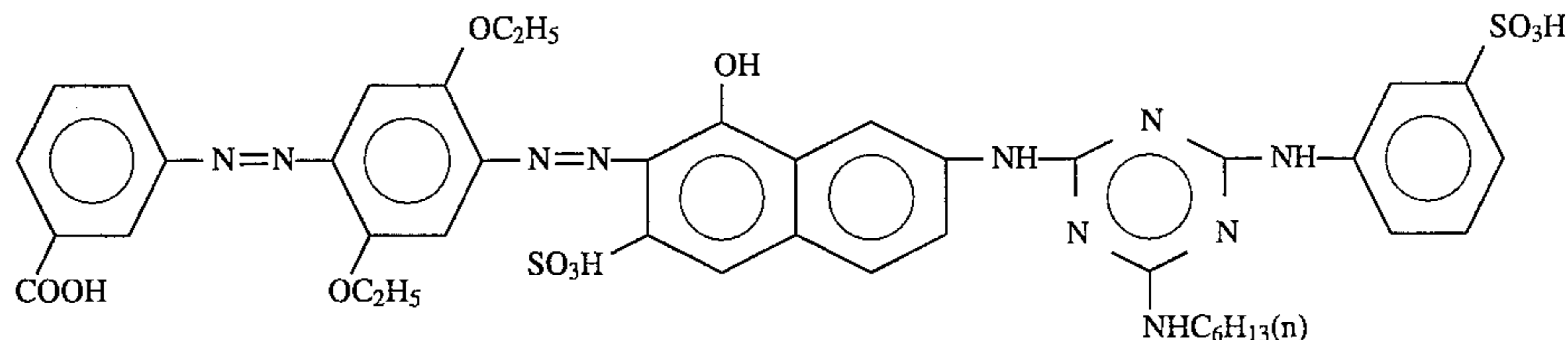
Structural Formula (3):
