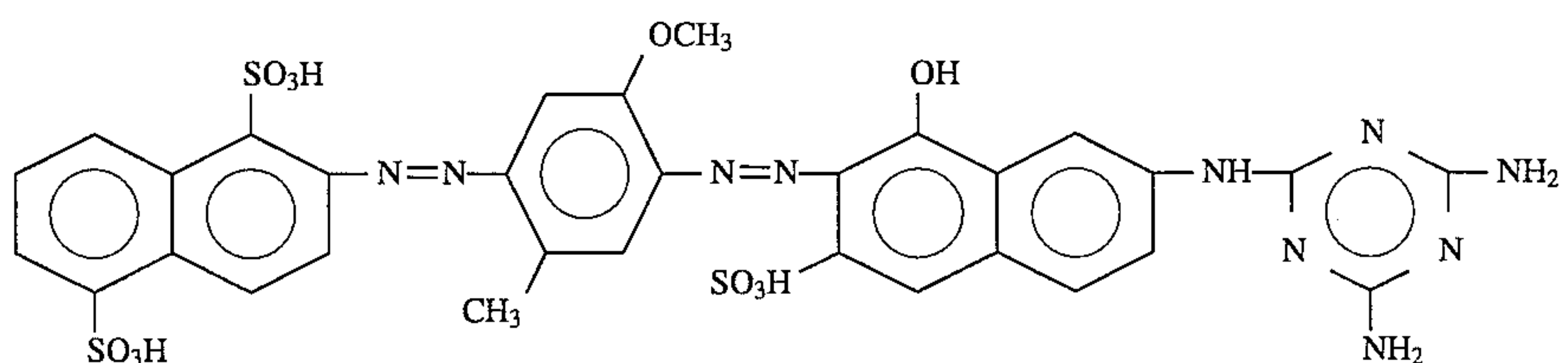
Structural Formula (2):
