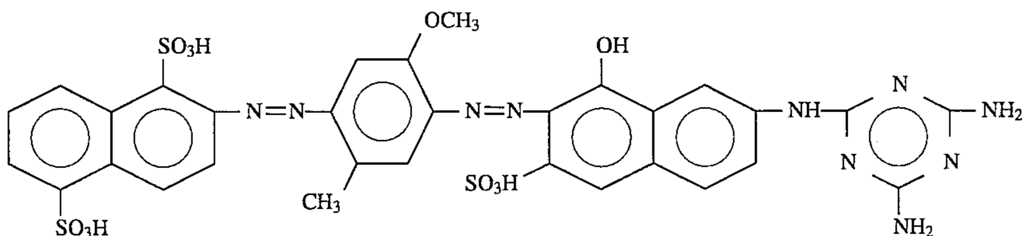
Structural Formula (2):
