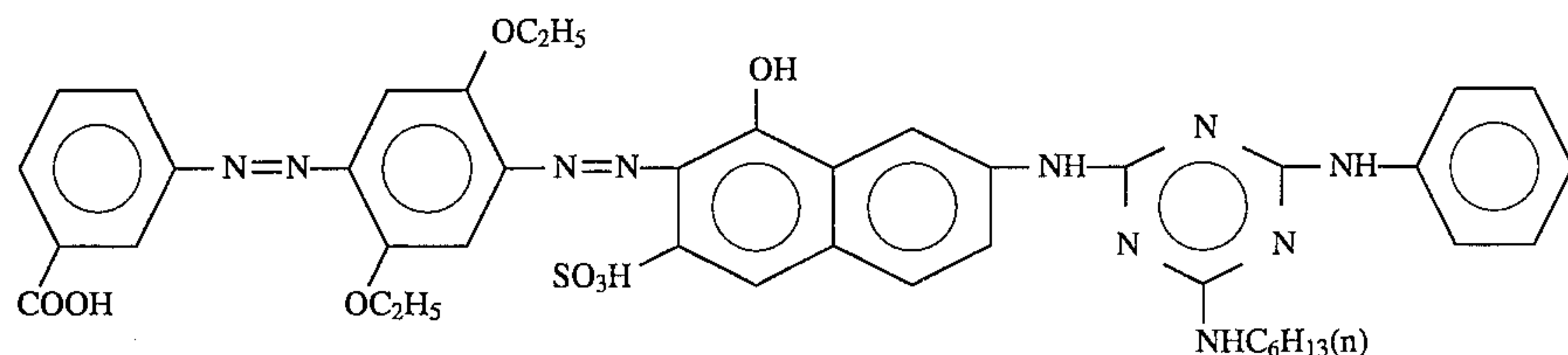
Structural Formula (3):
