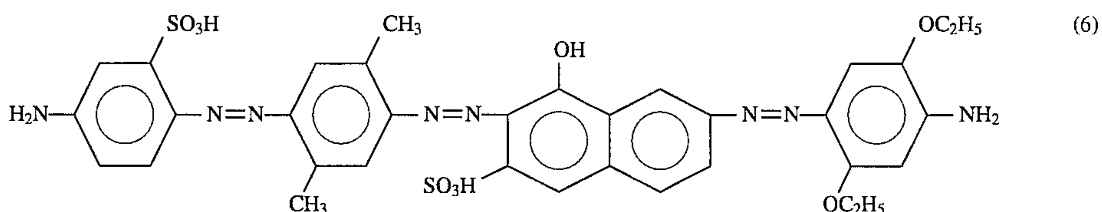
Structural Formula (6):
