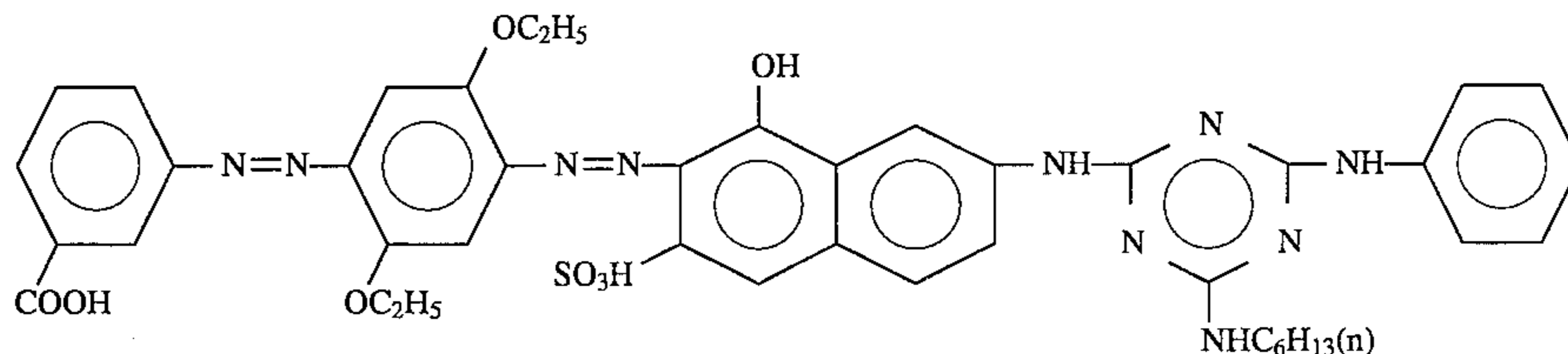
Structural Formula (3):
