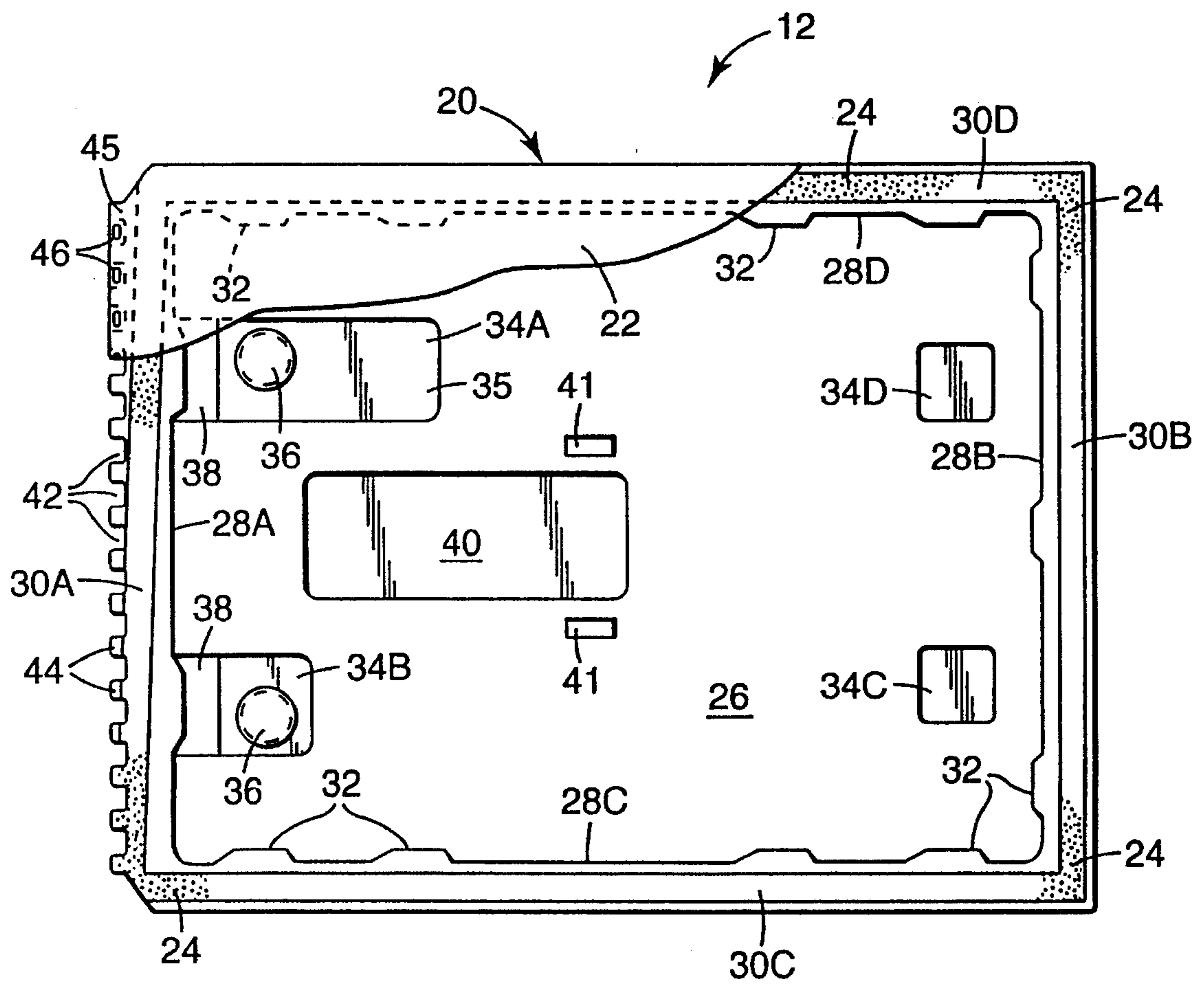
Fig. 3 PRIOR ART
