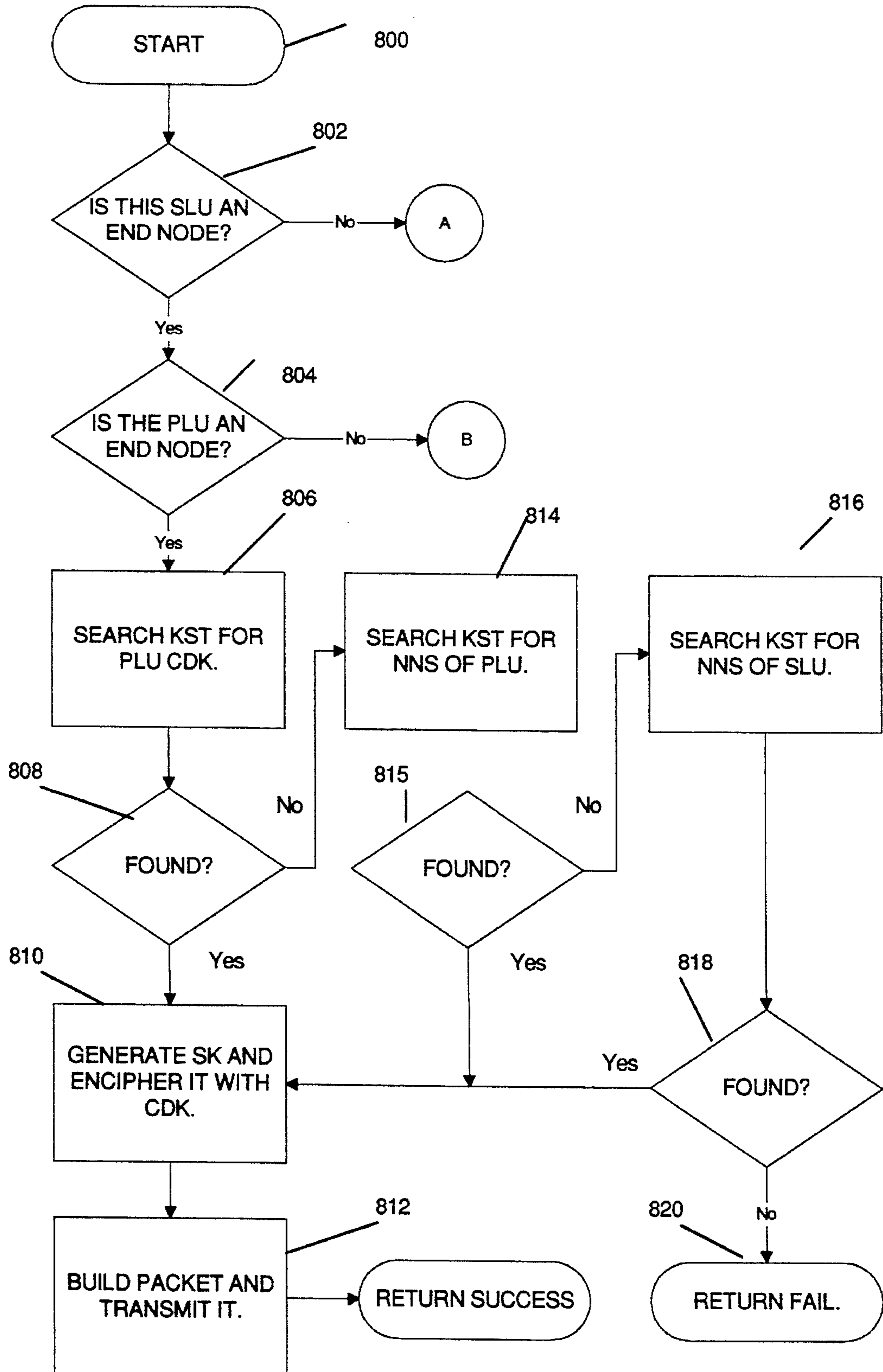
FIG. 8 - APPN SELECT KEY ALGORITHM (EXECUTED AT A SLU DESTINATION)
