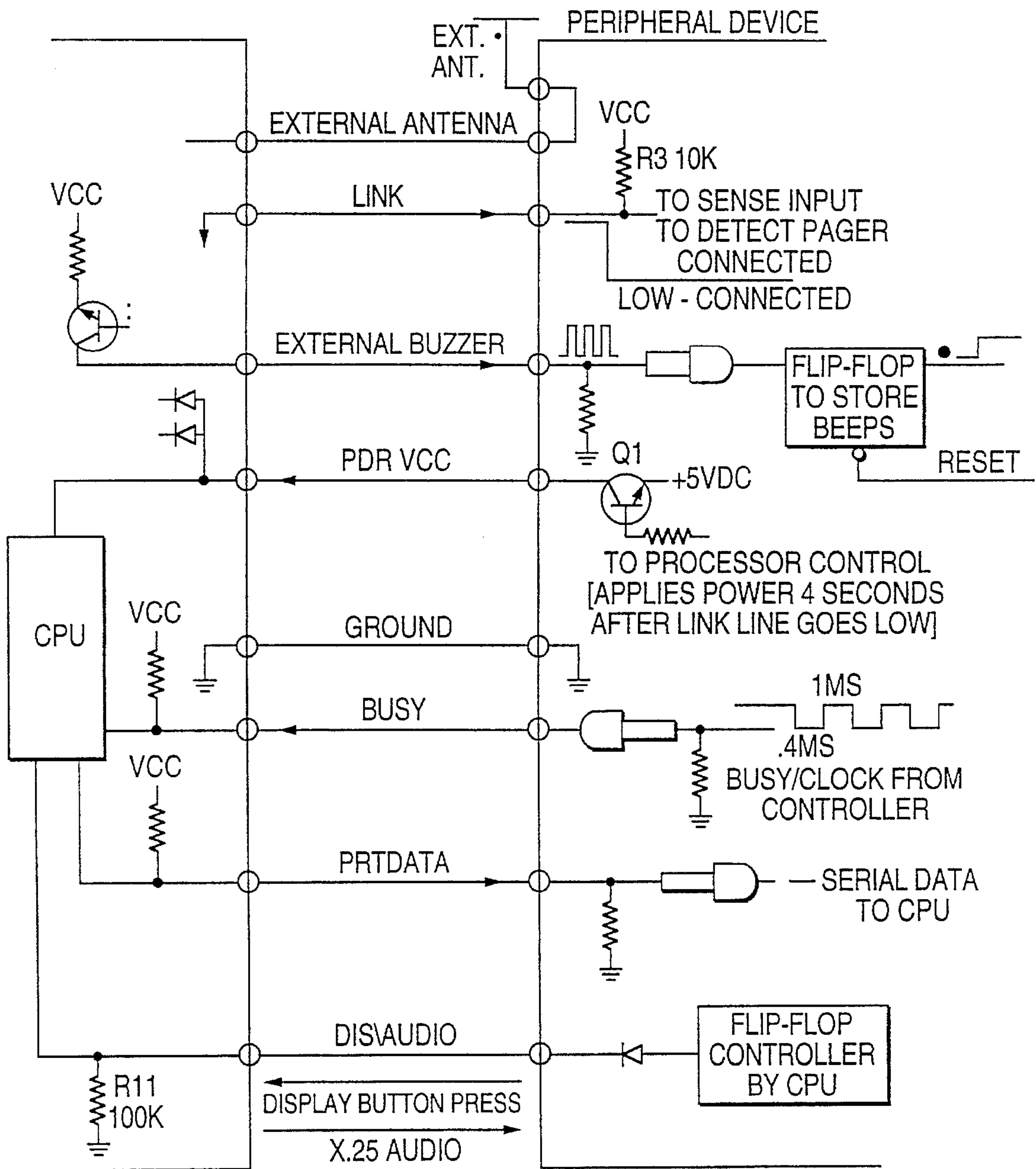
FIG. 7 PRIOR ART
