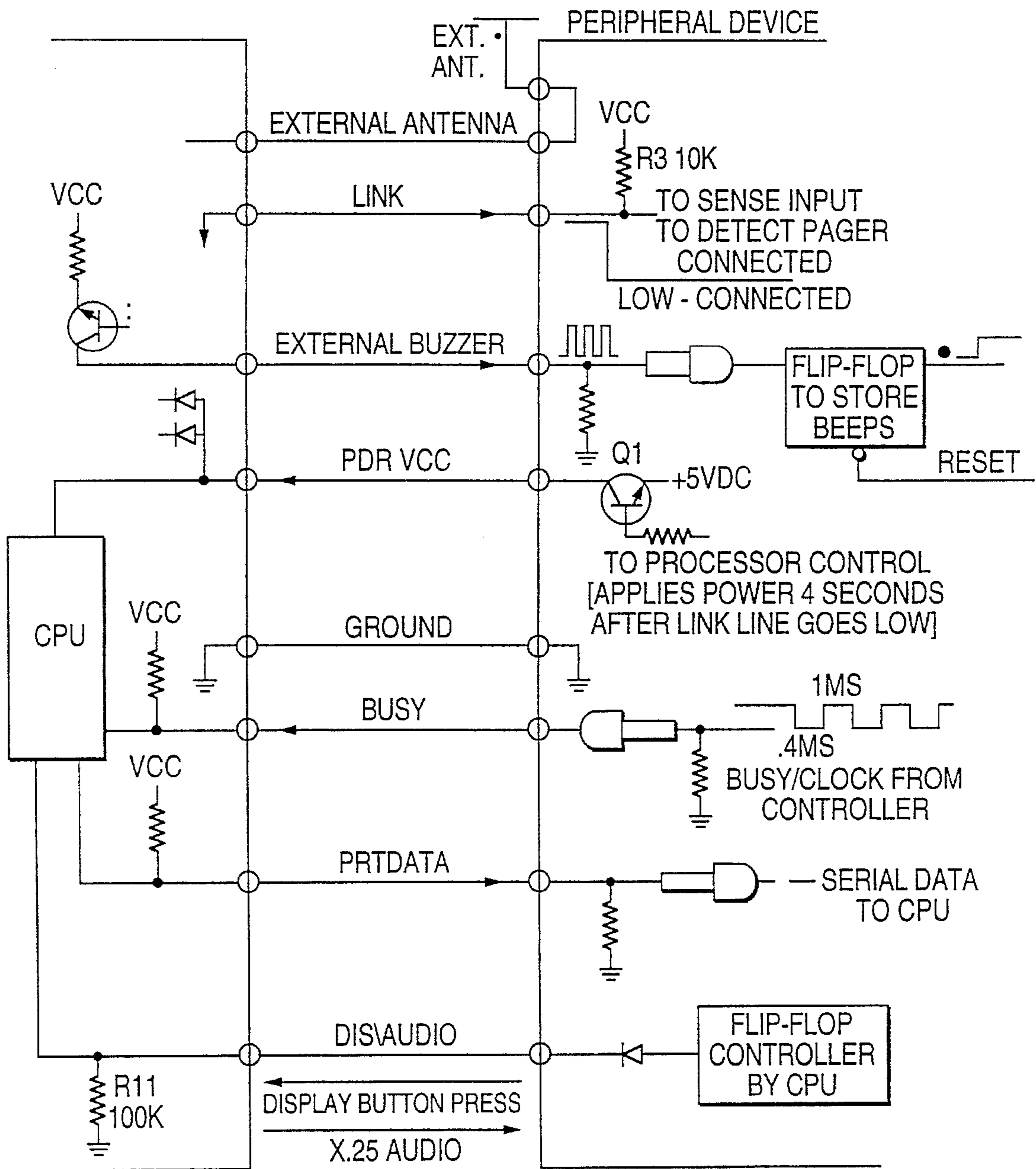
FIG. 7 PRIOR ART
