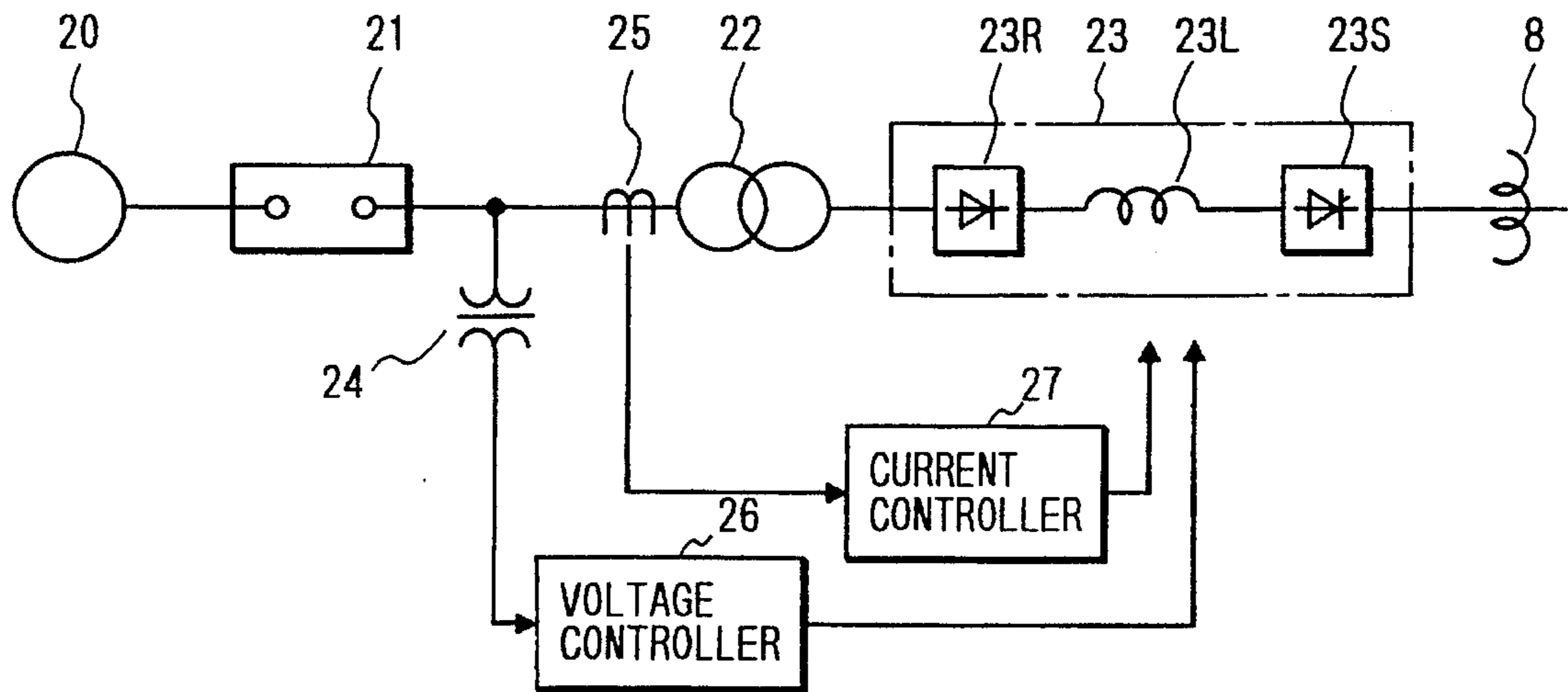
FIG. 15 (PRIOR ART)
