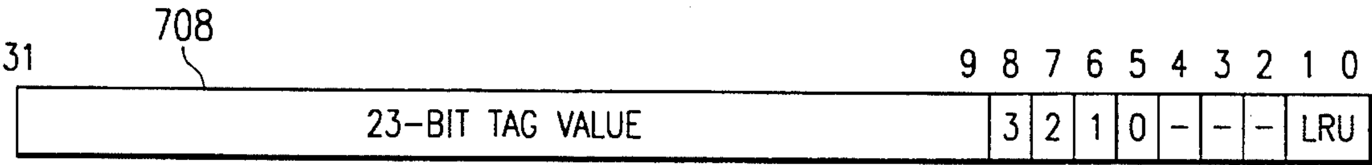
FIG. 35 SUB-BLOCK PRESENT BITS
