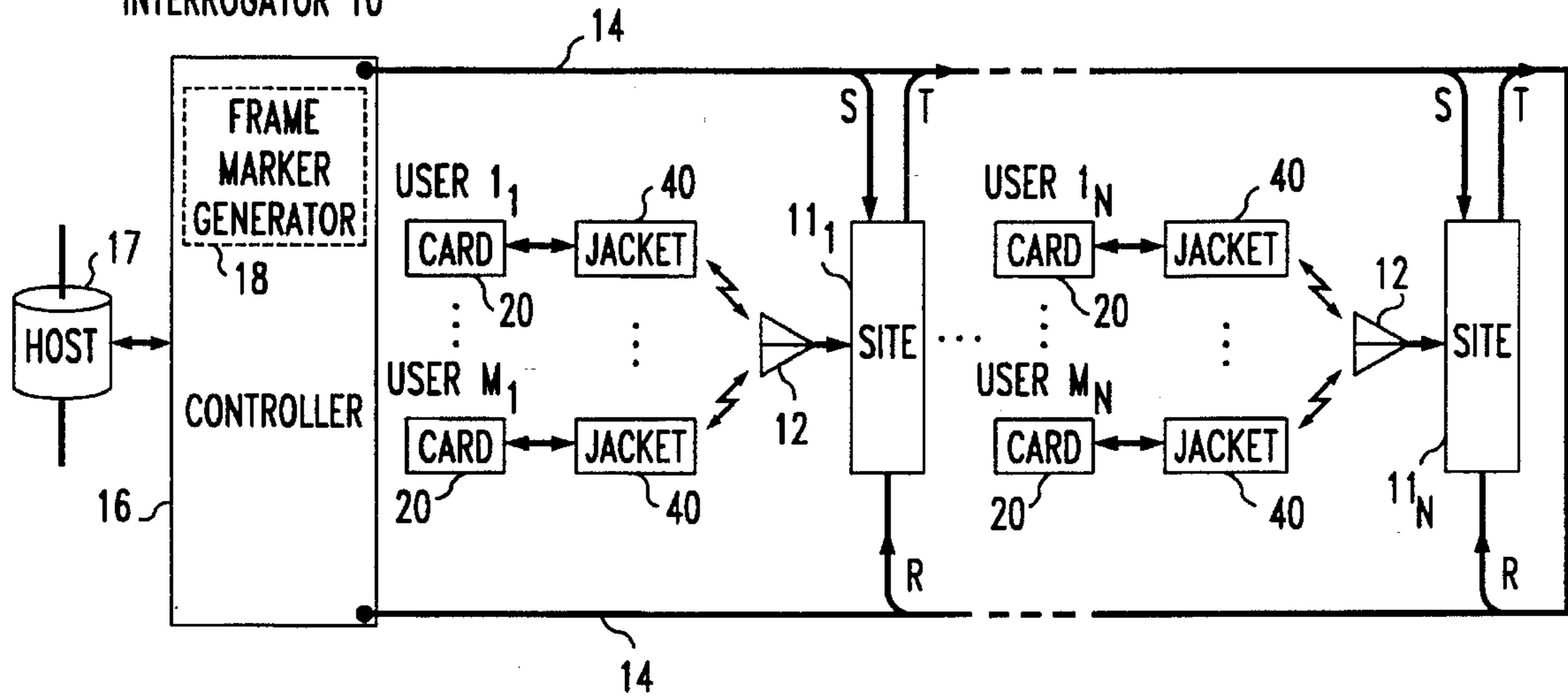
FIG. 1 INTERROGATOR 10
