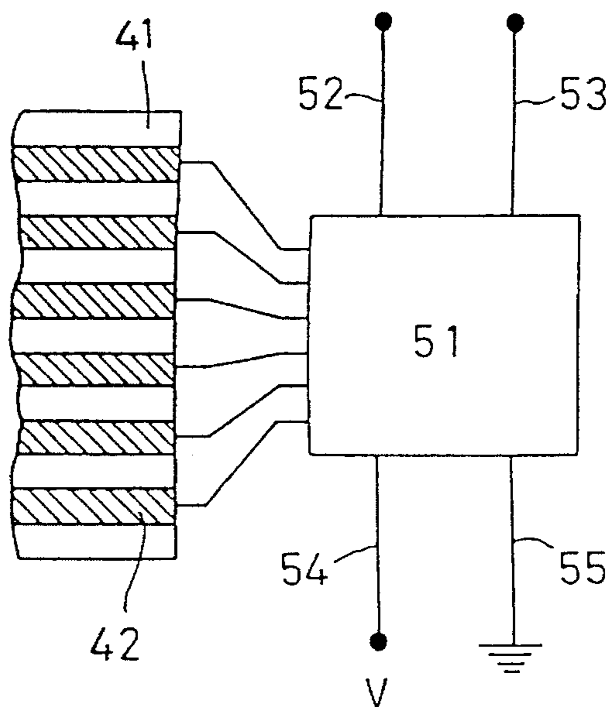
Fig.8 RELATED ART
