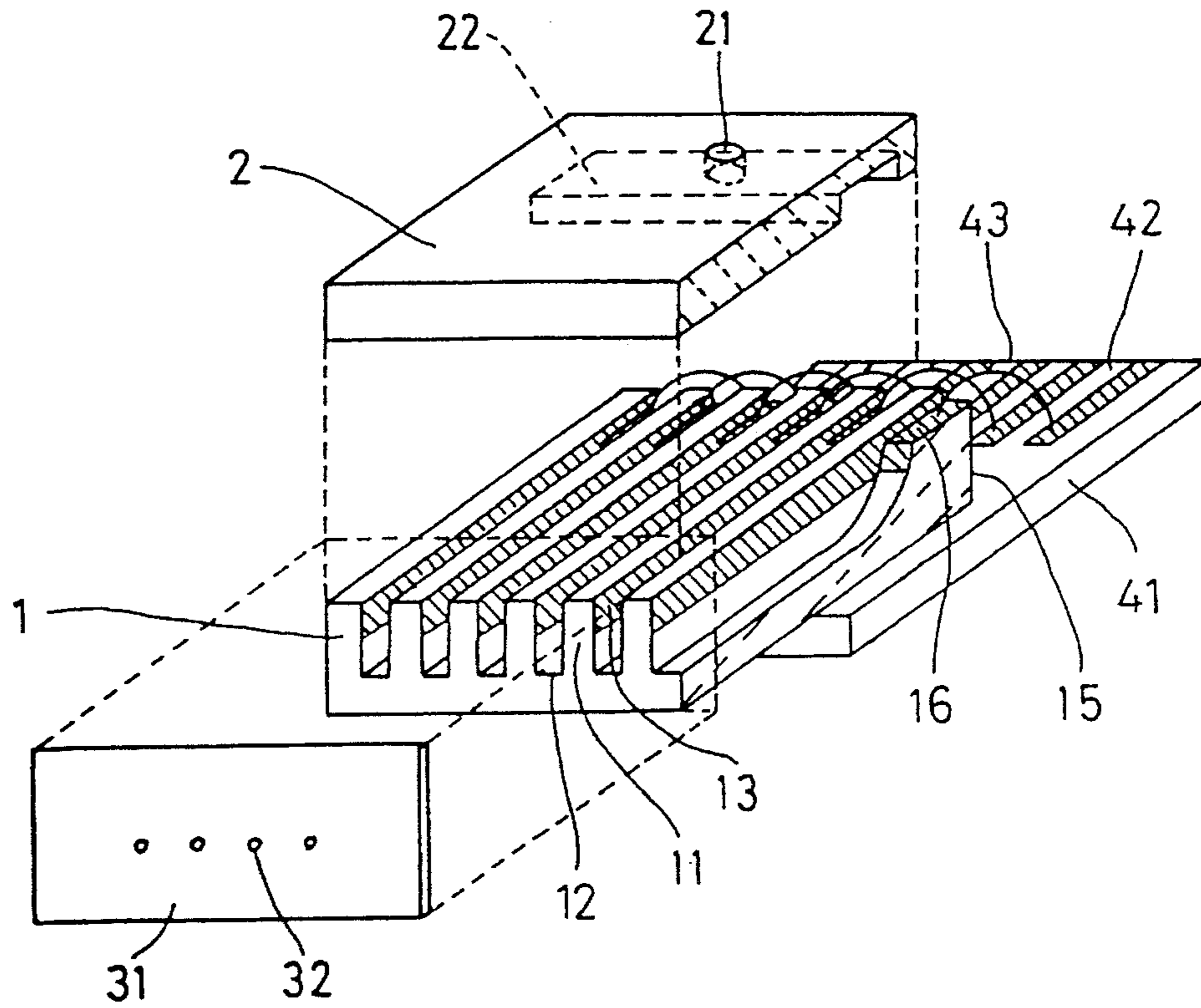
Fig.8 RELATED ART
