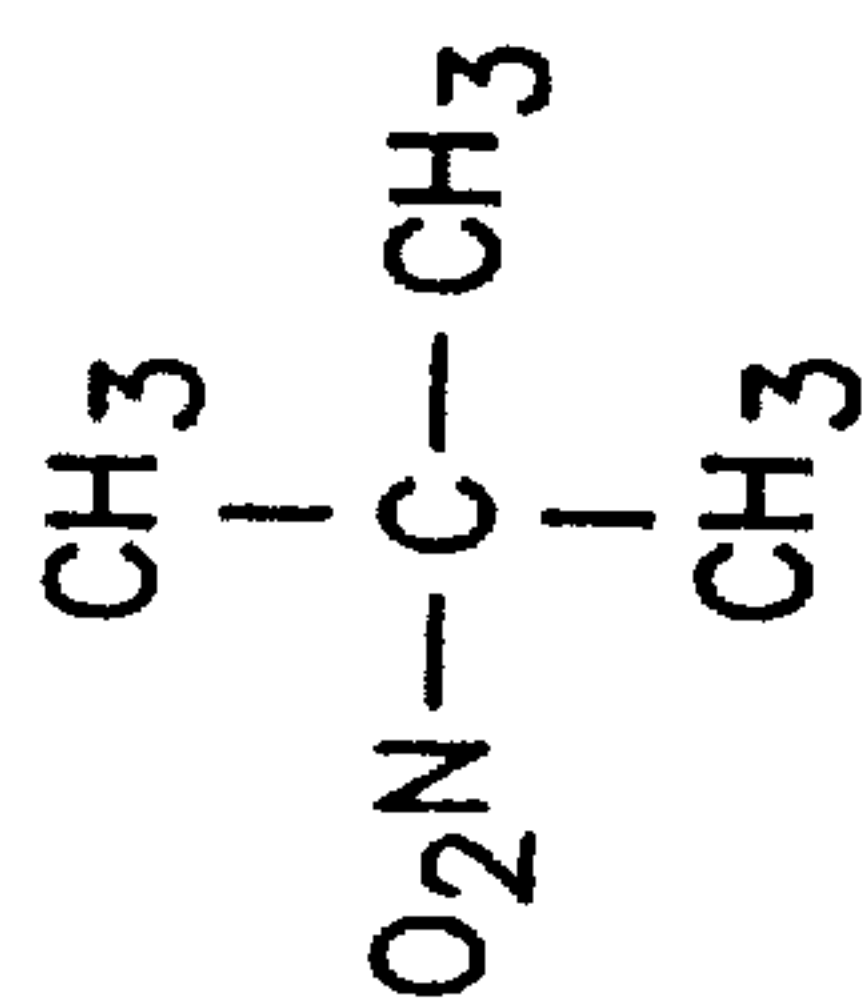
2-Methyl-2-nitropropane
