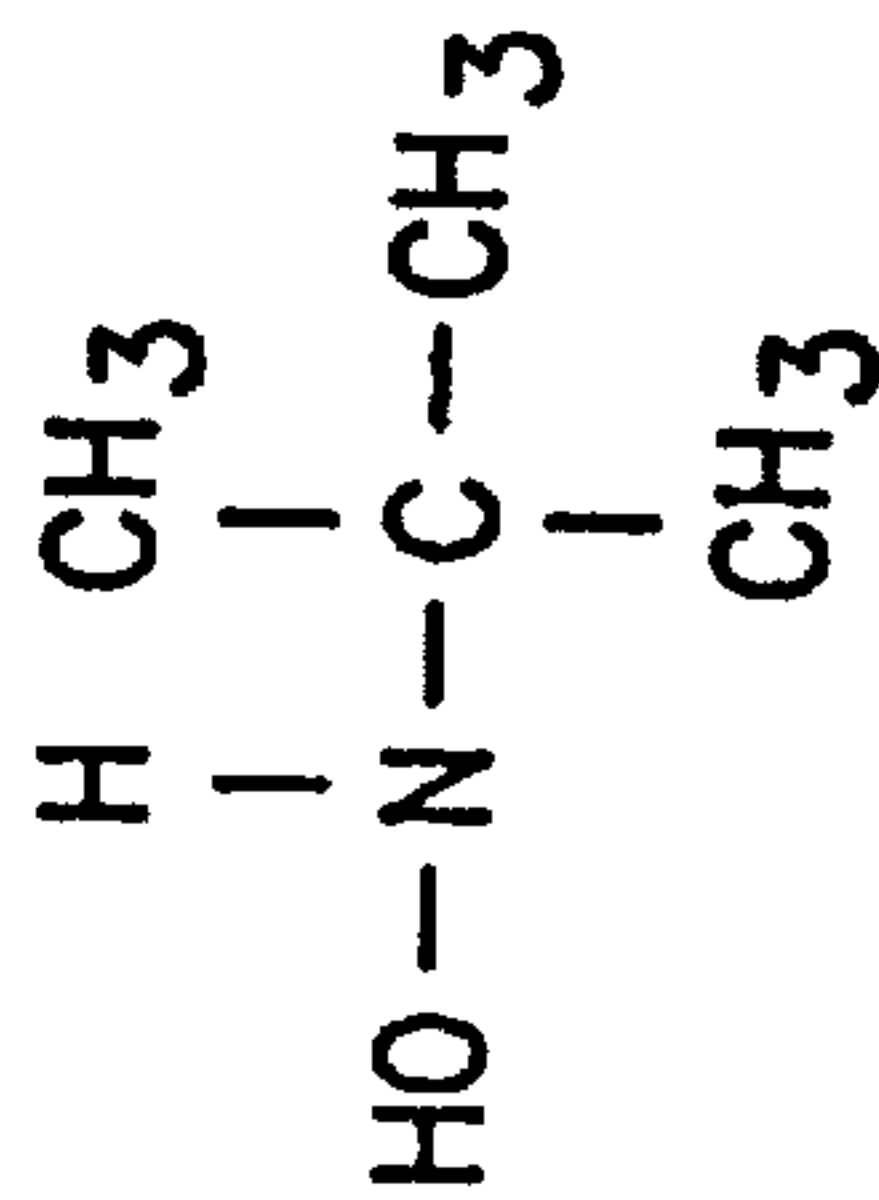
t -Butylhydroxylamine
