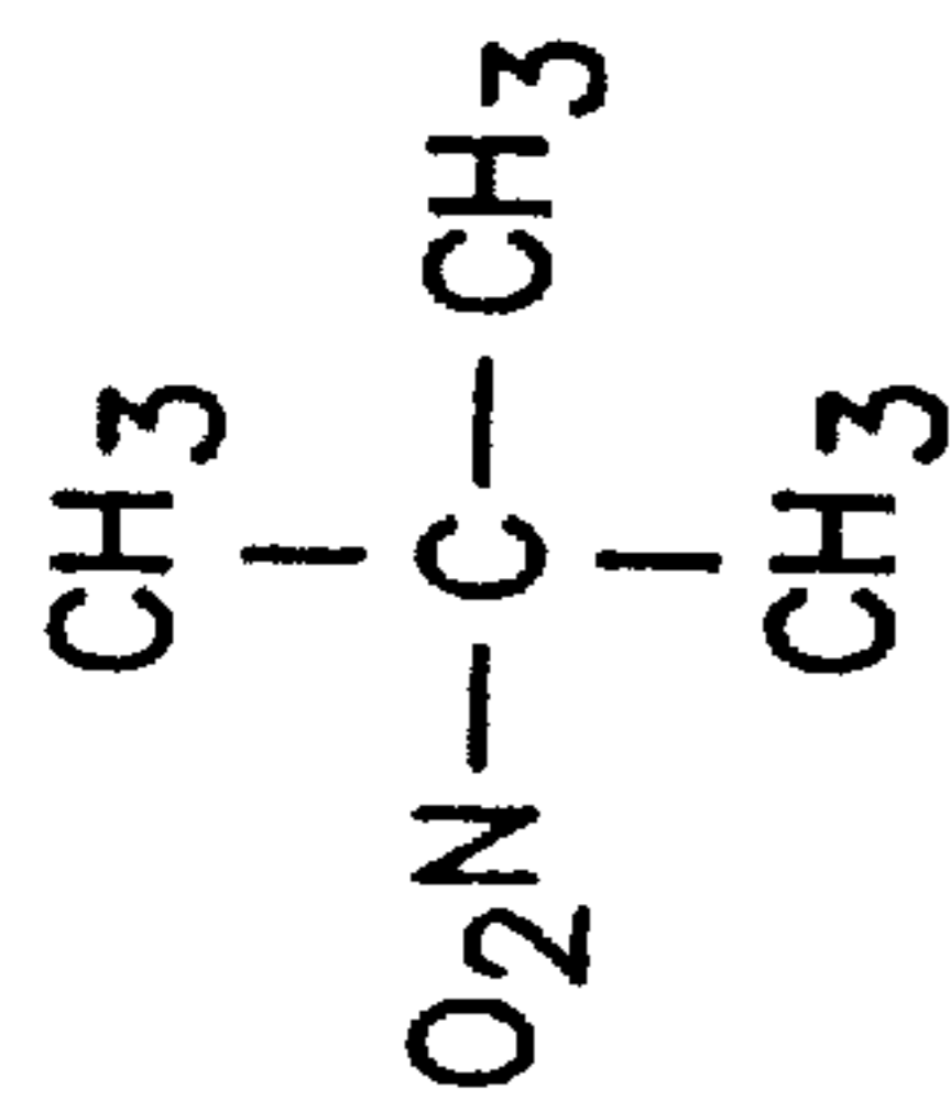
2-Methyl-2-nitropropane
