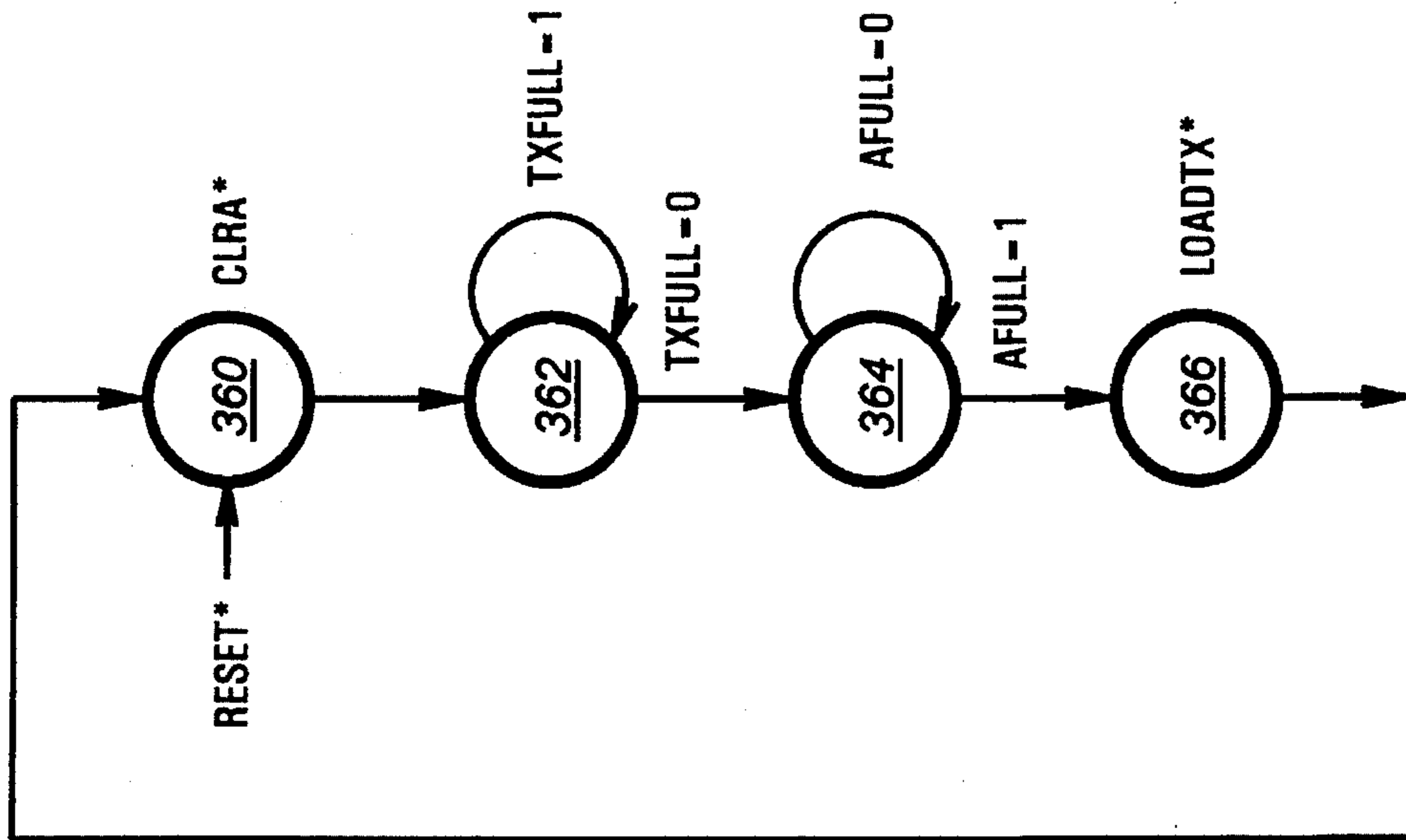
TRANSMITTER BUFFER CONTROLLER STATE MACHINE
