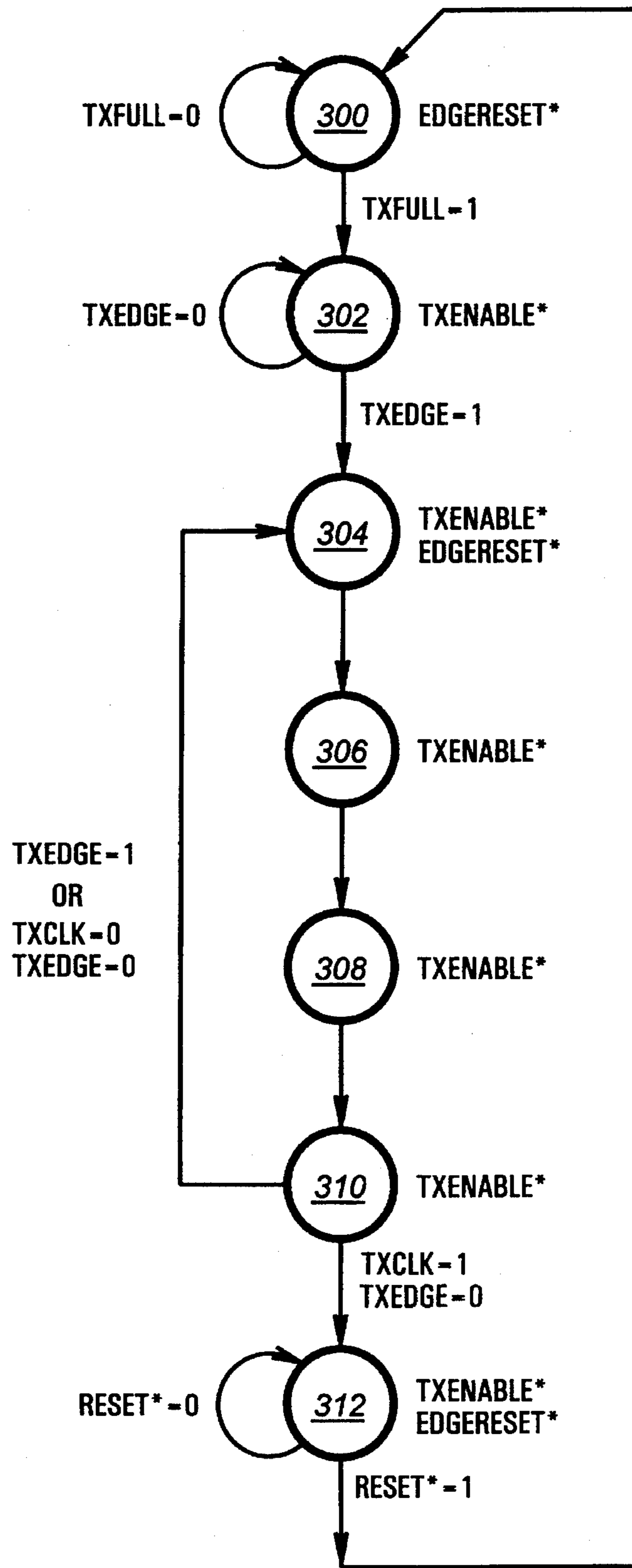
TRANSMITTER STATE MACHINE
