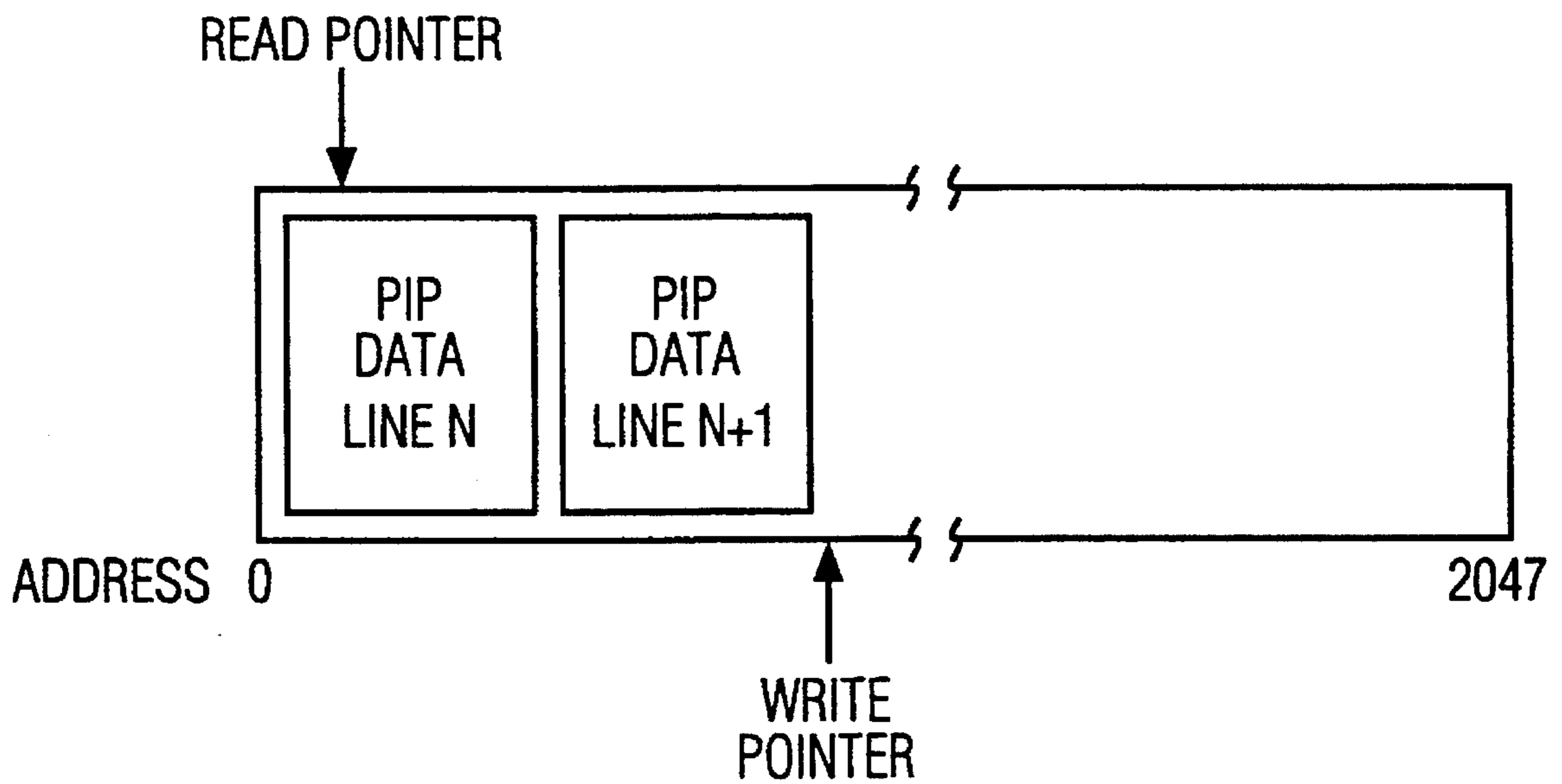
FIG. 18 AUX FIFO MEMORY STORAGE
