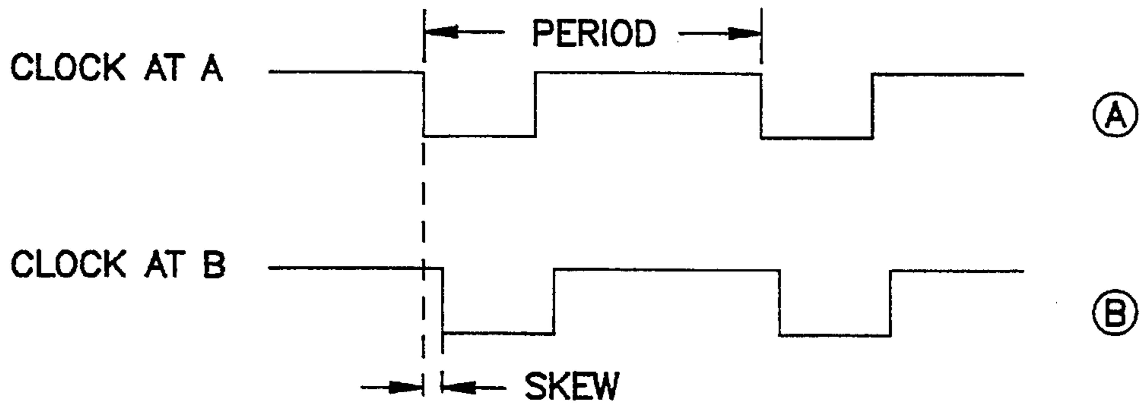
FIG. 2 PRIOR ART
