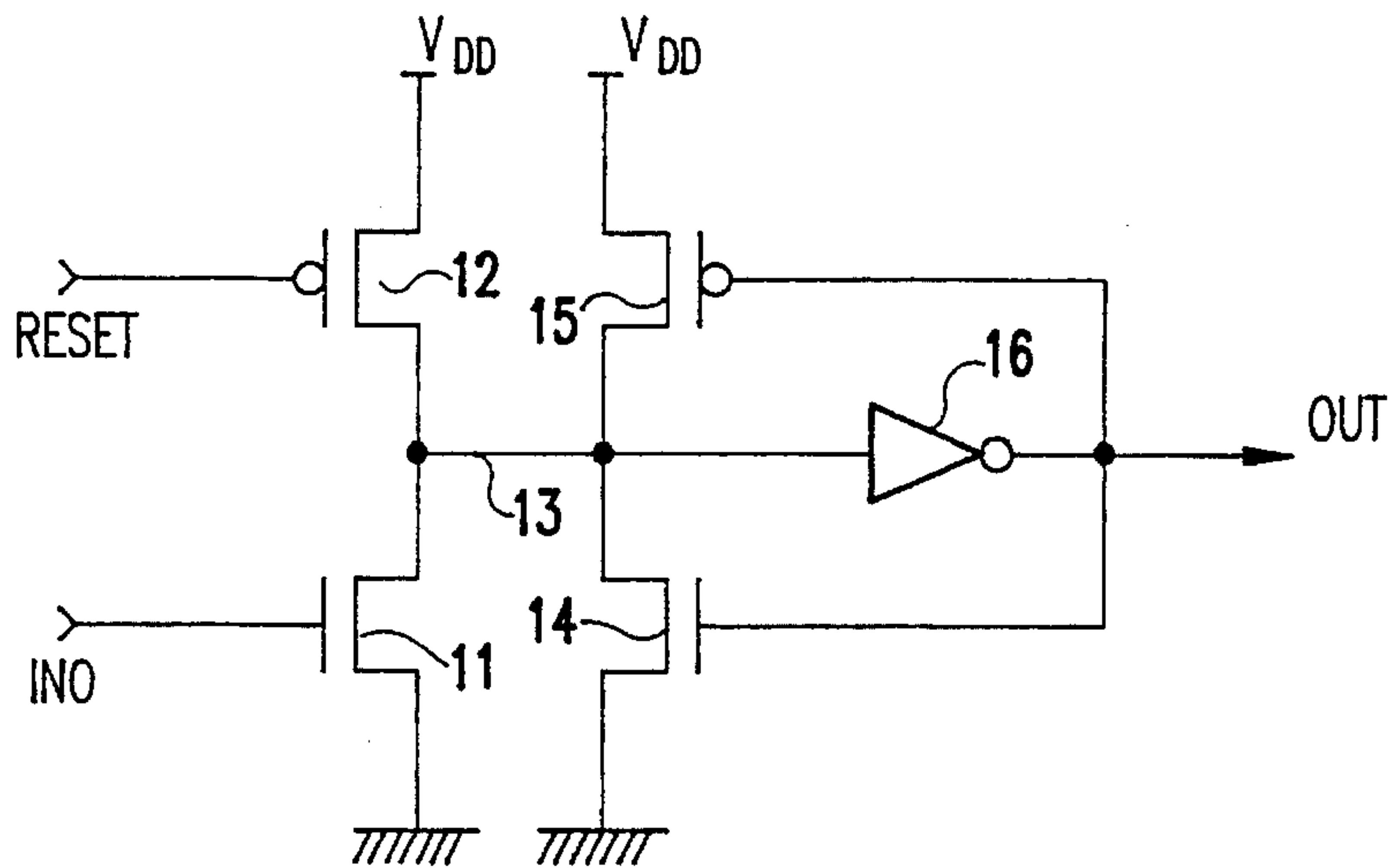
FIG. 1 PRIOR ART
