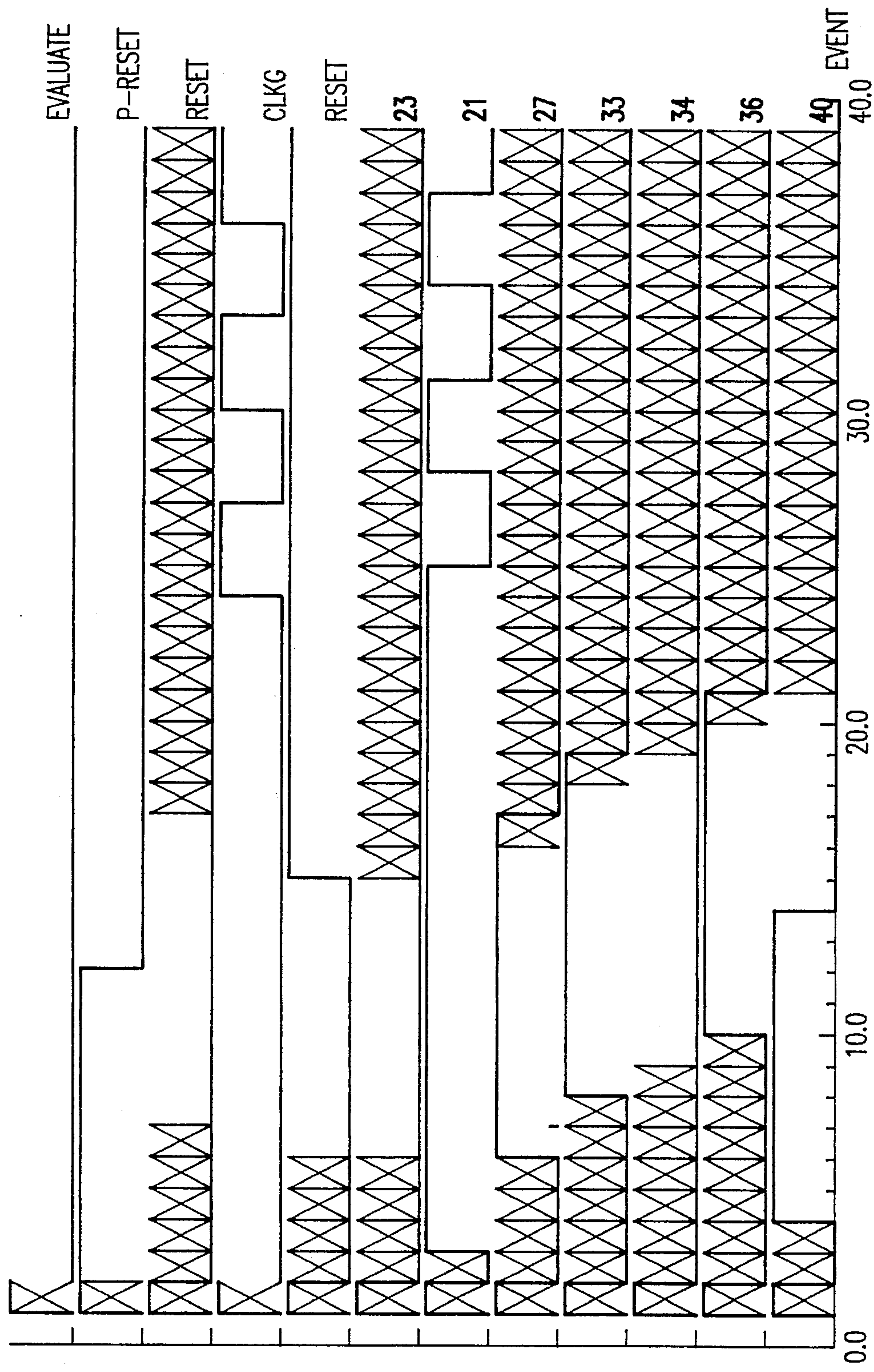
FIG. 3 PRIOR ART
