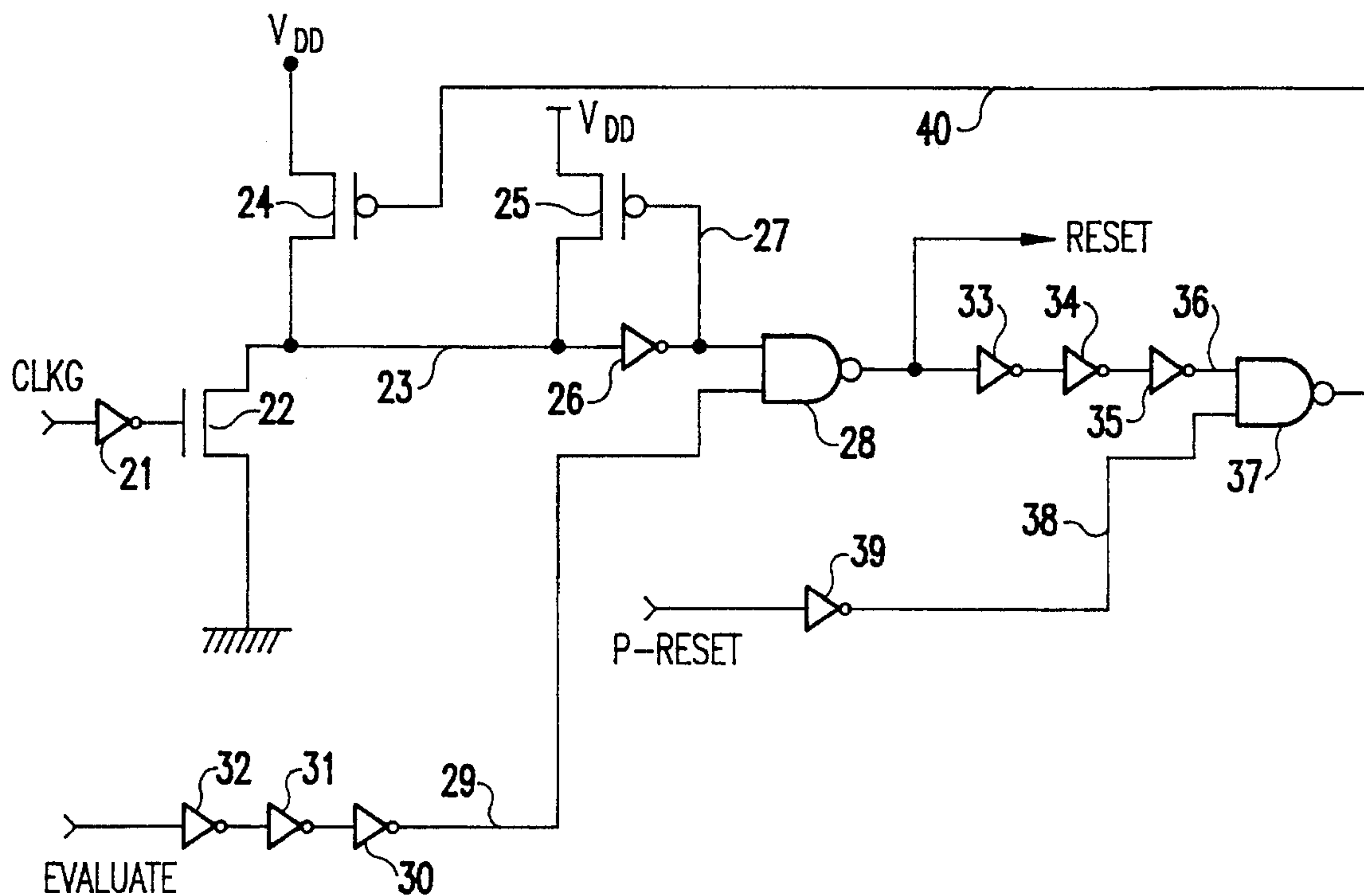
FIG. 2 PRIOR ART
