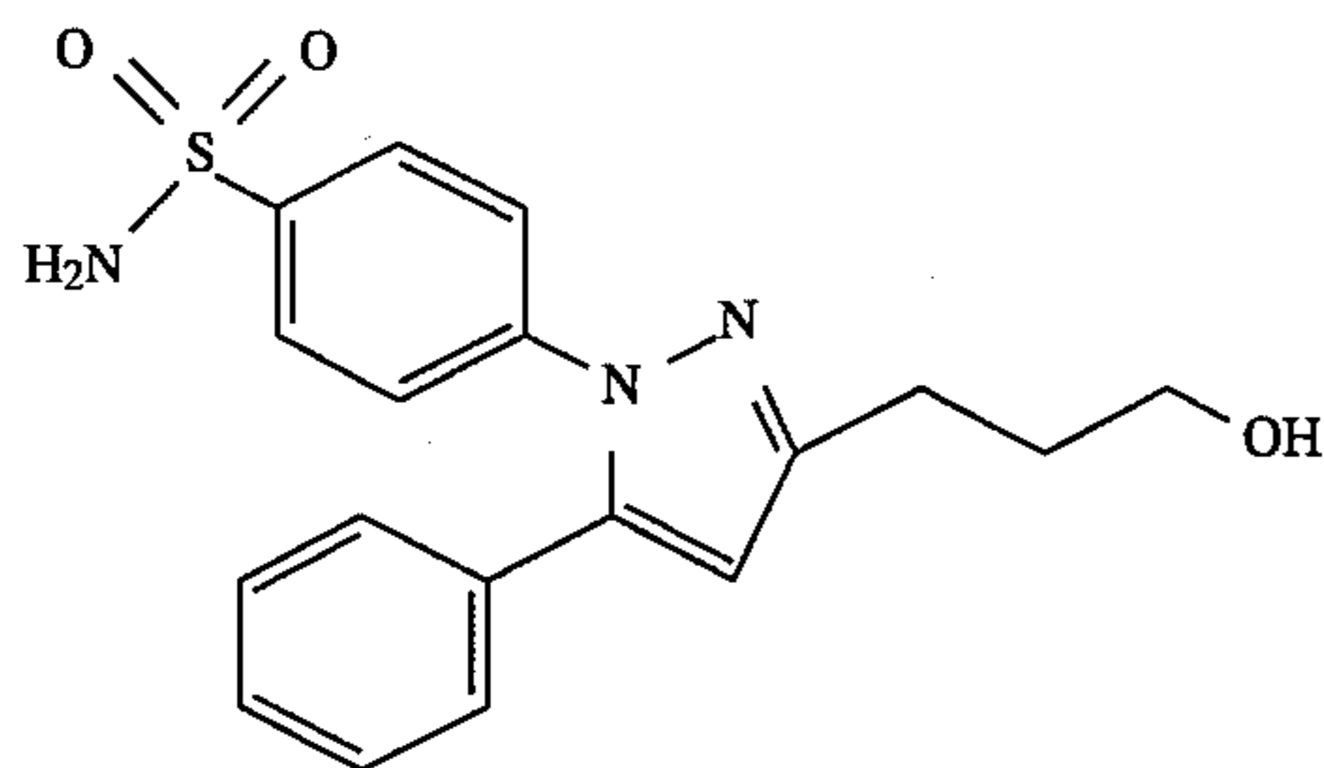
4-[5-Phenyl-3-(3-hydroxypropyl)-1H-pyrazol-1-yl]benzenesulfonamide
