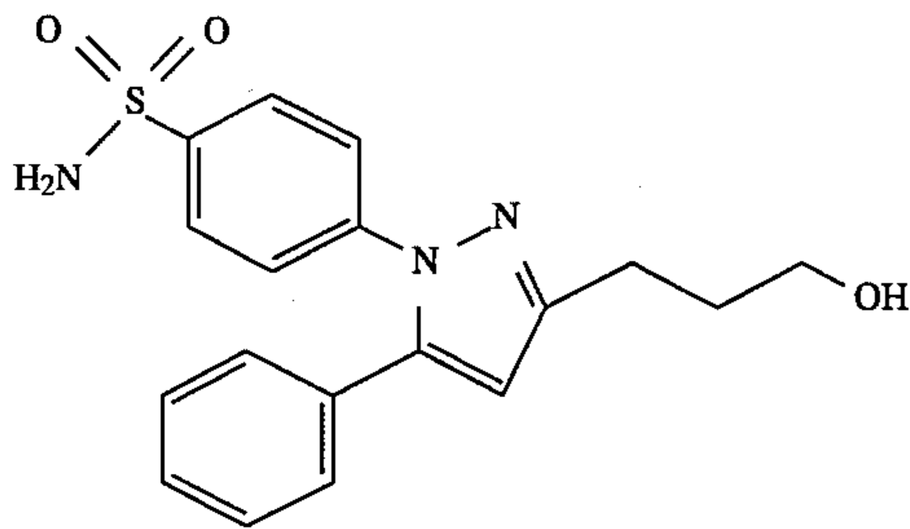
4-[5-Phenyl-3-(3-hydroxypropyl)-1H-pyrazol-1-yl]benzenesulfonamide
