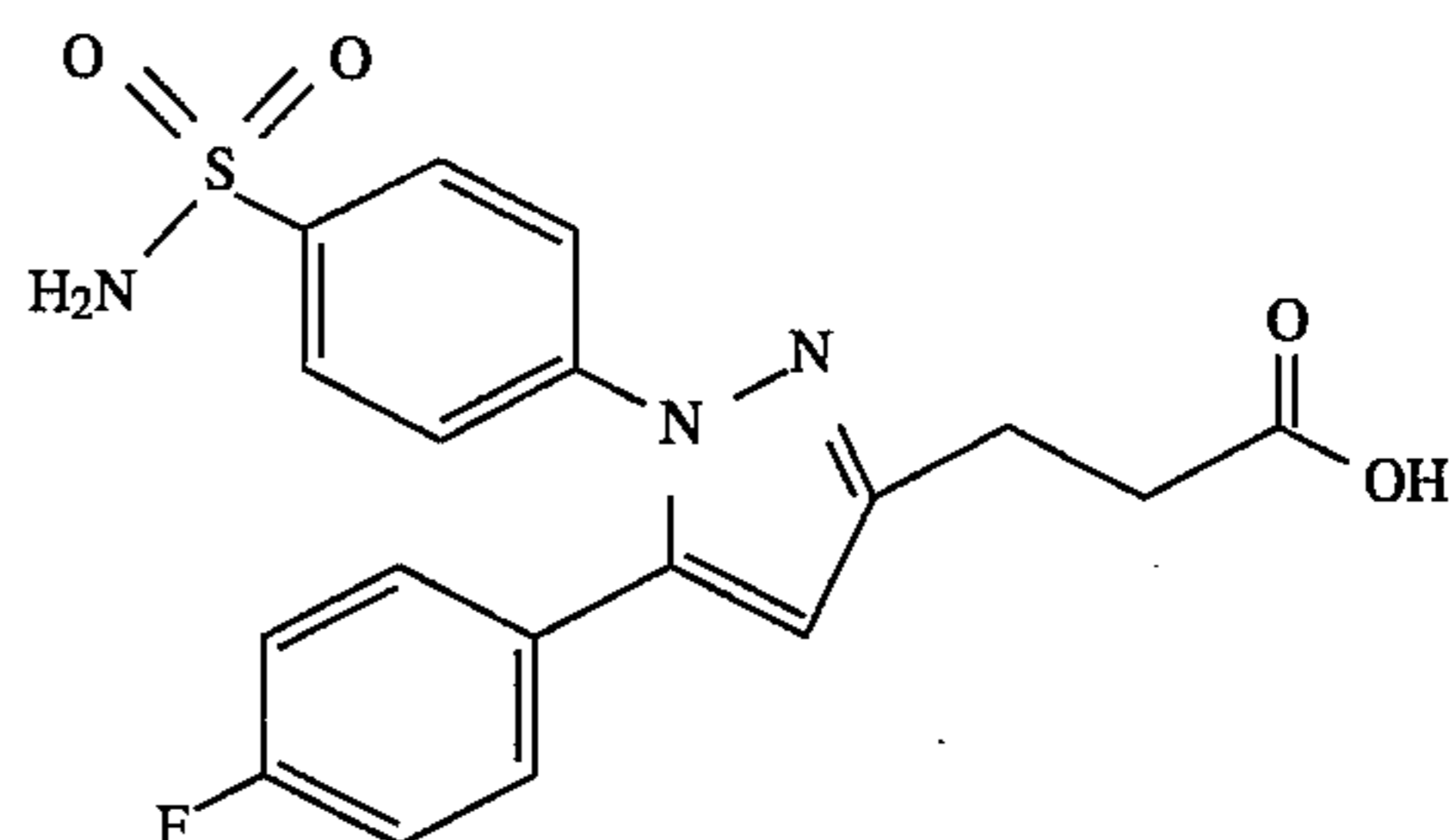
4-[4-(Aminosulfonyl)phenyl]-5-(4-fluorophenyl)-1H-pyrazole-3-propanoic acid
