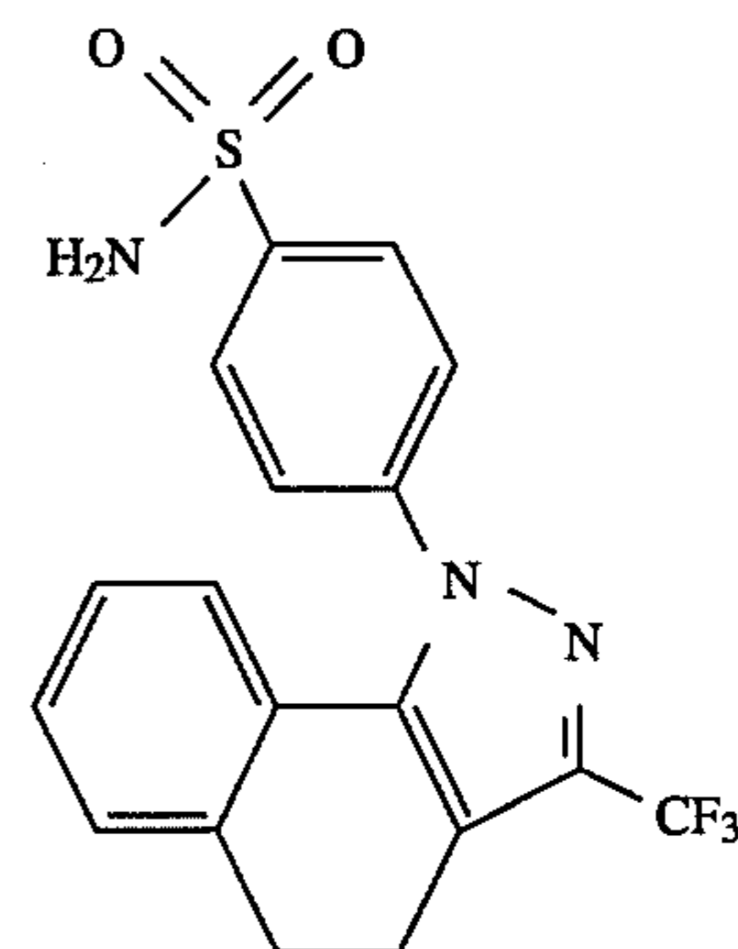
4,5-Dihydro-4-[3-trifluoromethyl]-1H-benz[g]indazol-1-yl]benzenesulfonamide
