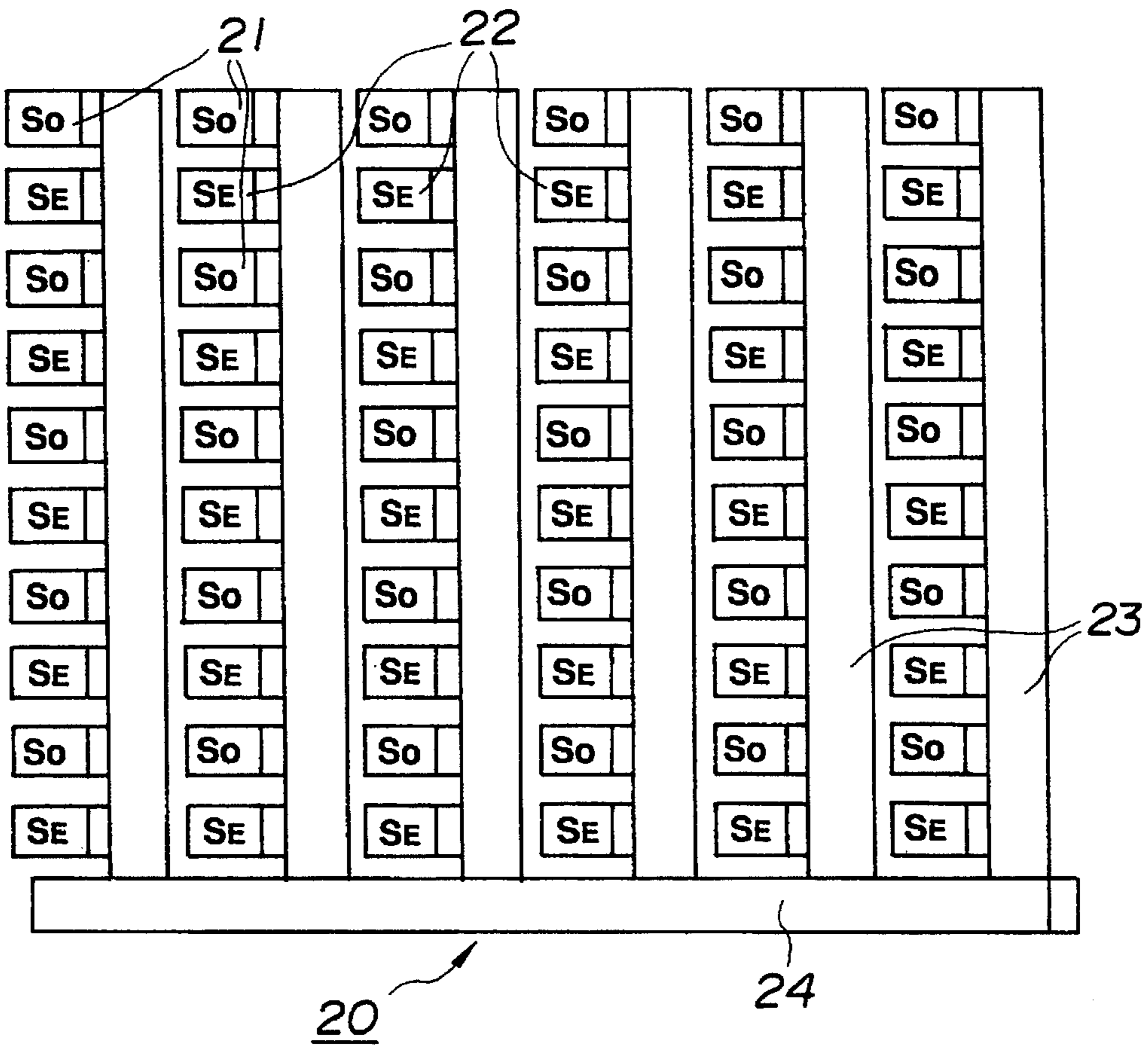
FIG.5 (PRIOR ART)
