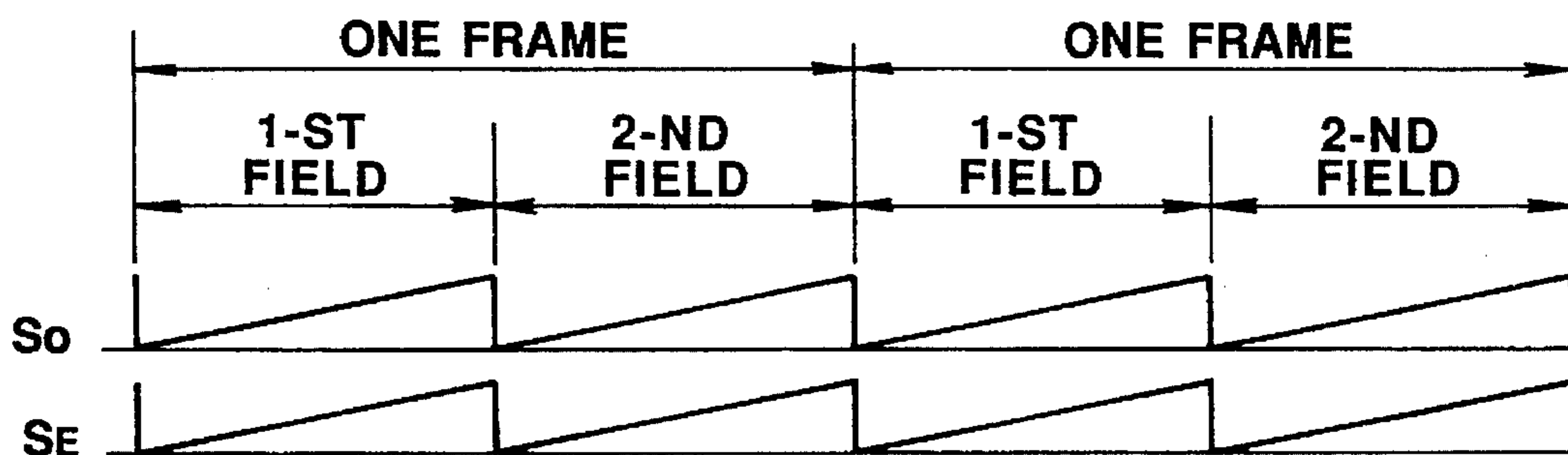
FIG.7 (PRIOR ART)
