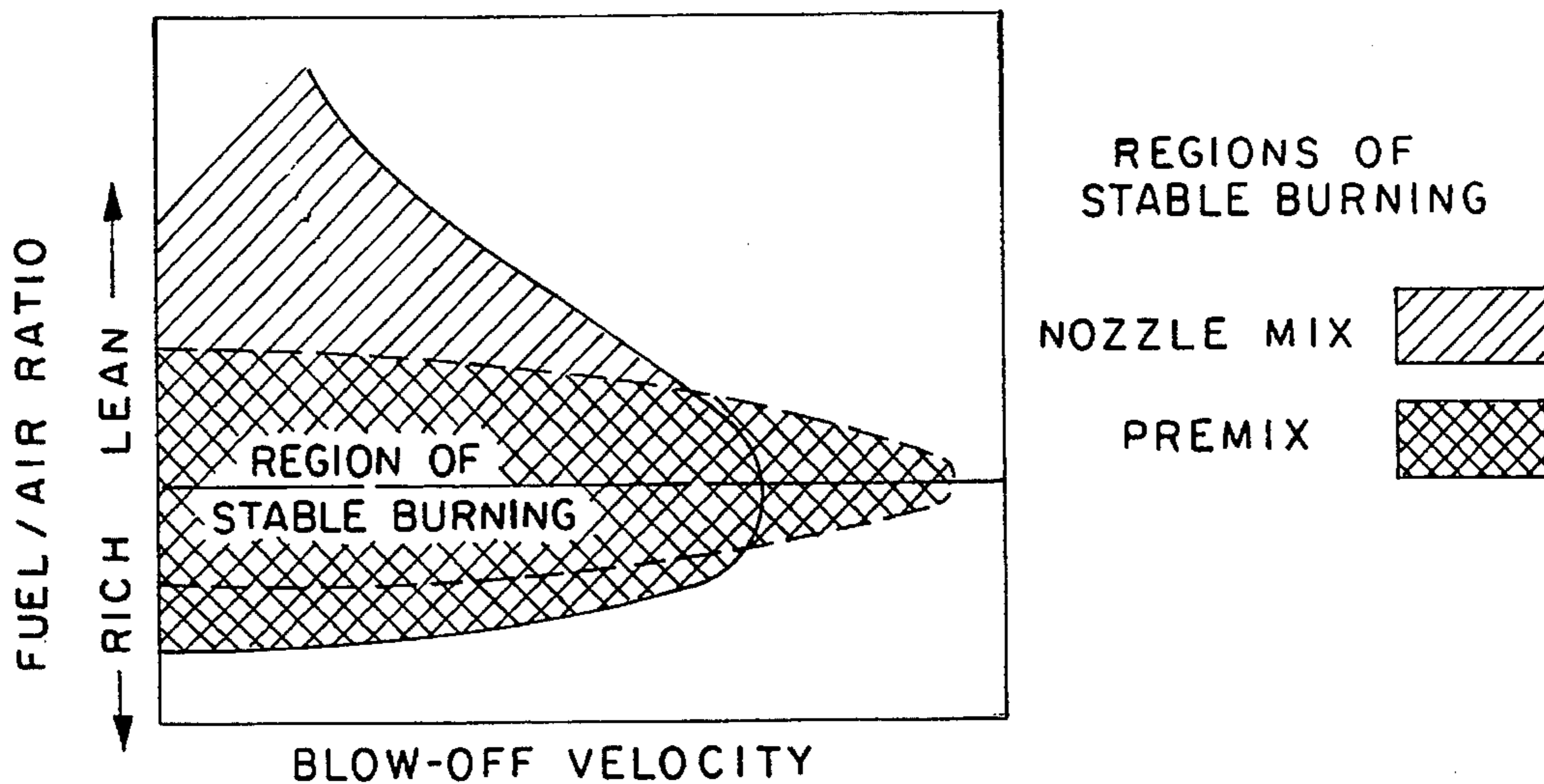
CHARACTERISTIC COMBUSTION STABILITY LOOPS
