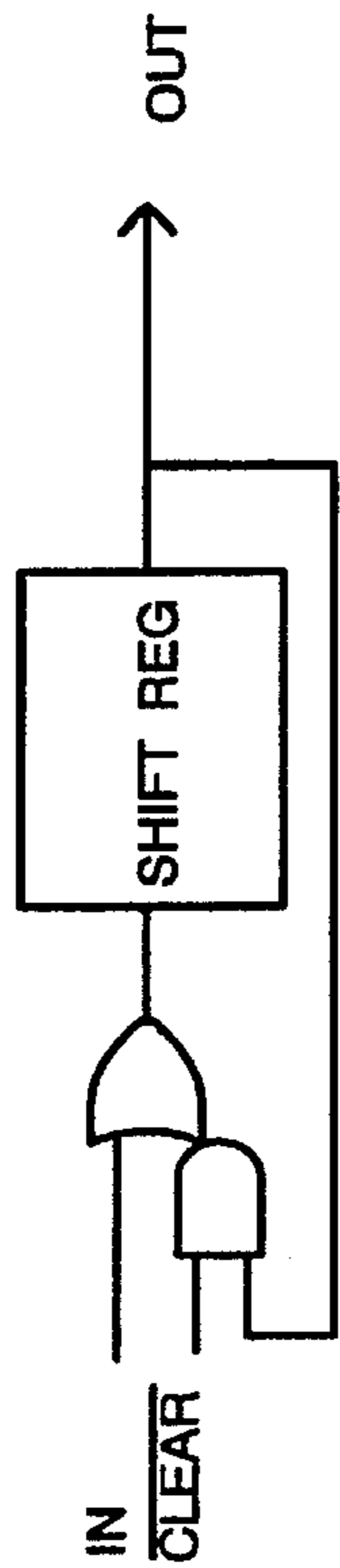
CS LATCH
