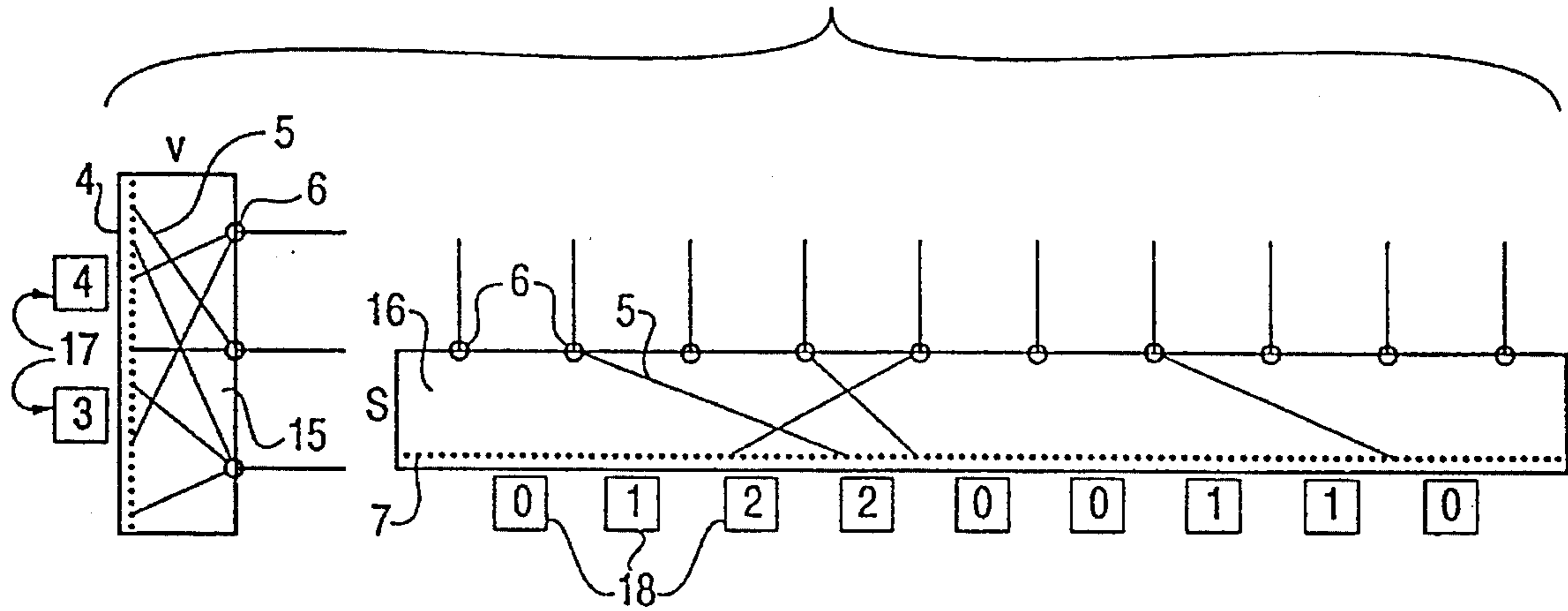
FIG. 3 PRIOR ART
