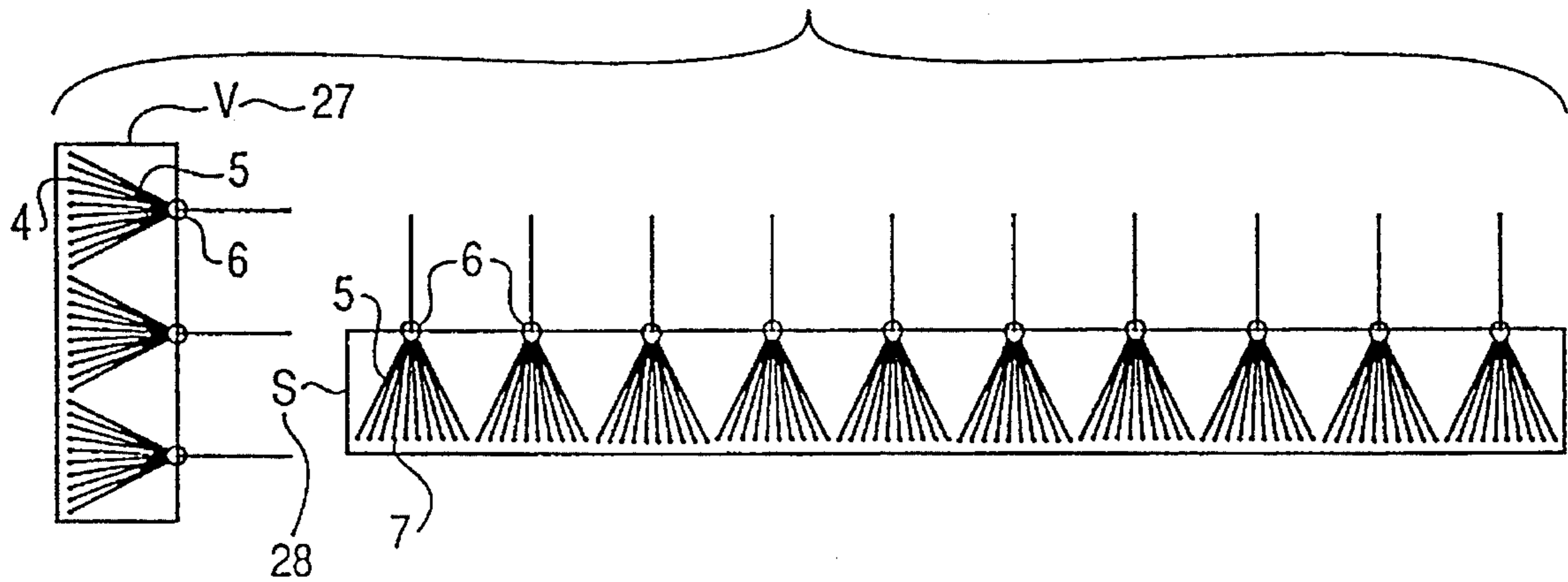
FIG. 2 PRIOR ART
