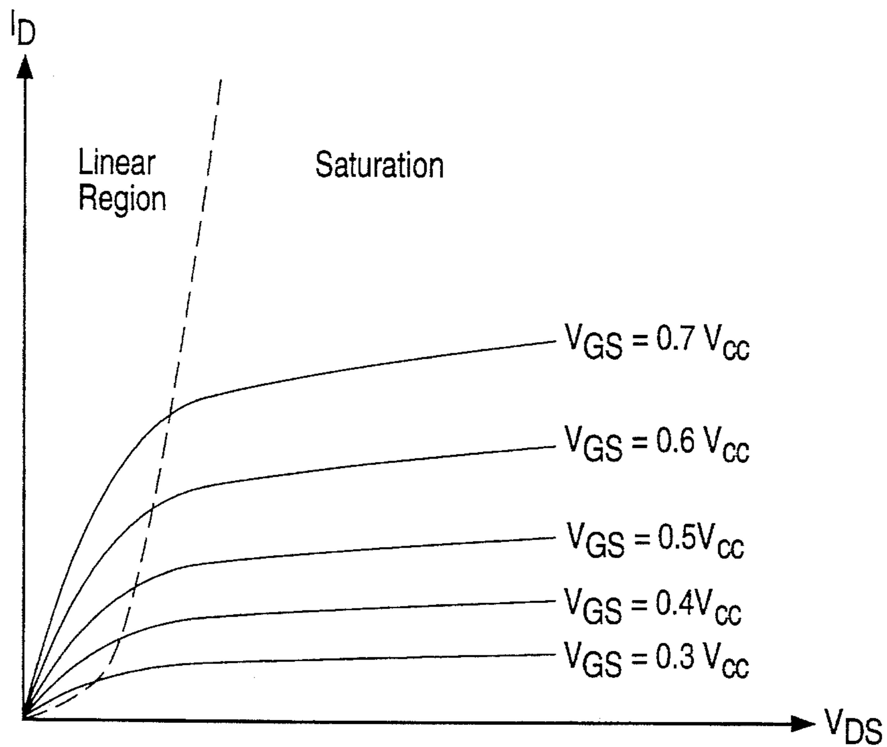
Output Characteristic of a Field Effect Transistor
