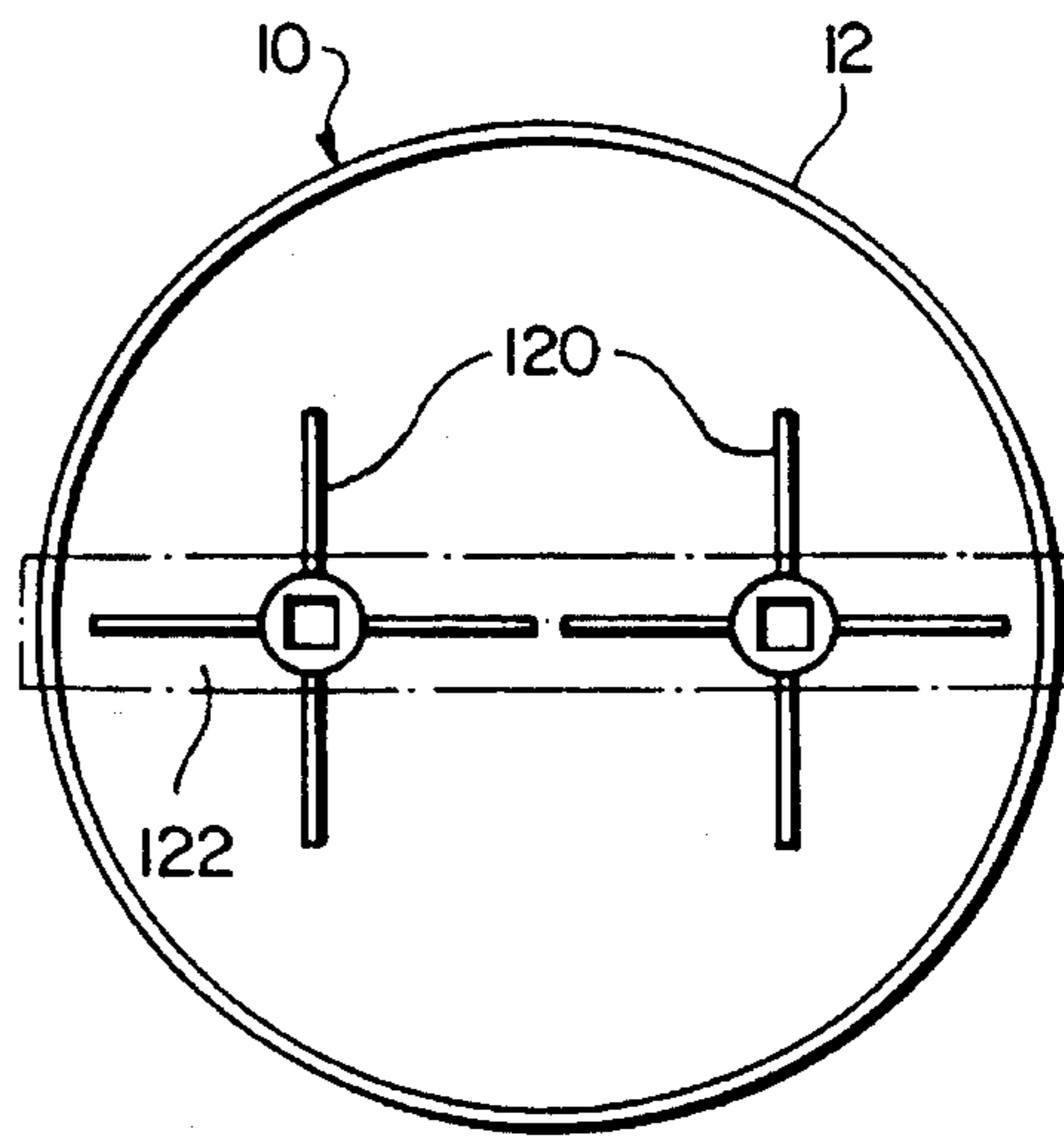
FIG. 15 PRIOR ART
