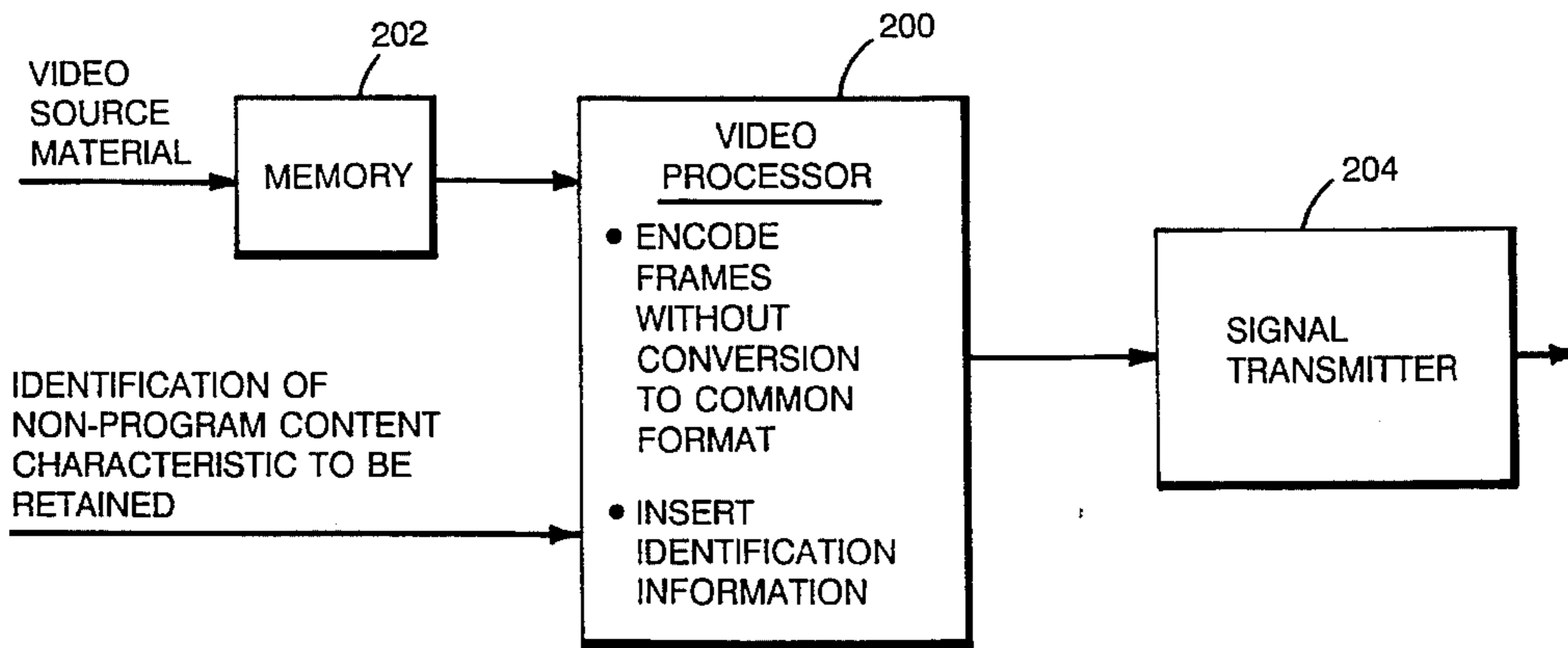
HDTV TRANSMITTER
