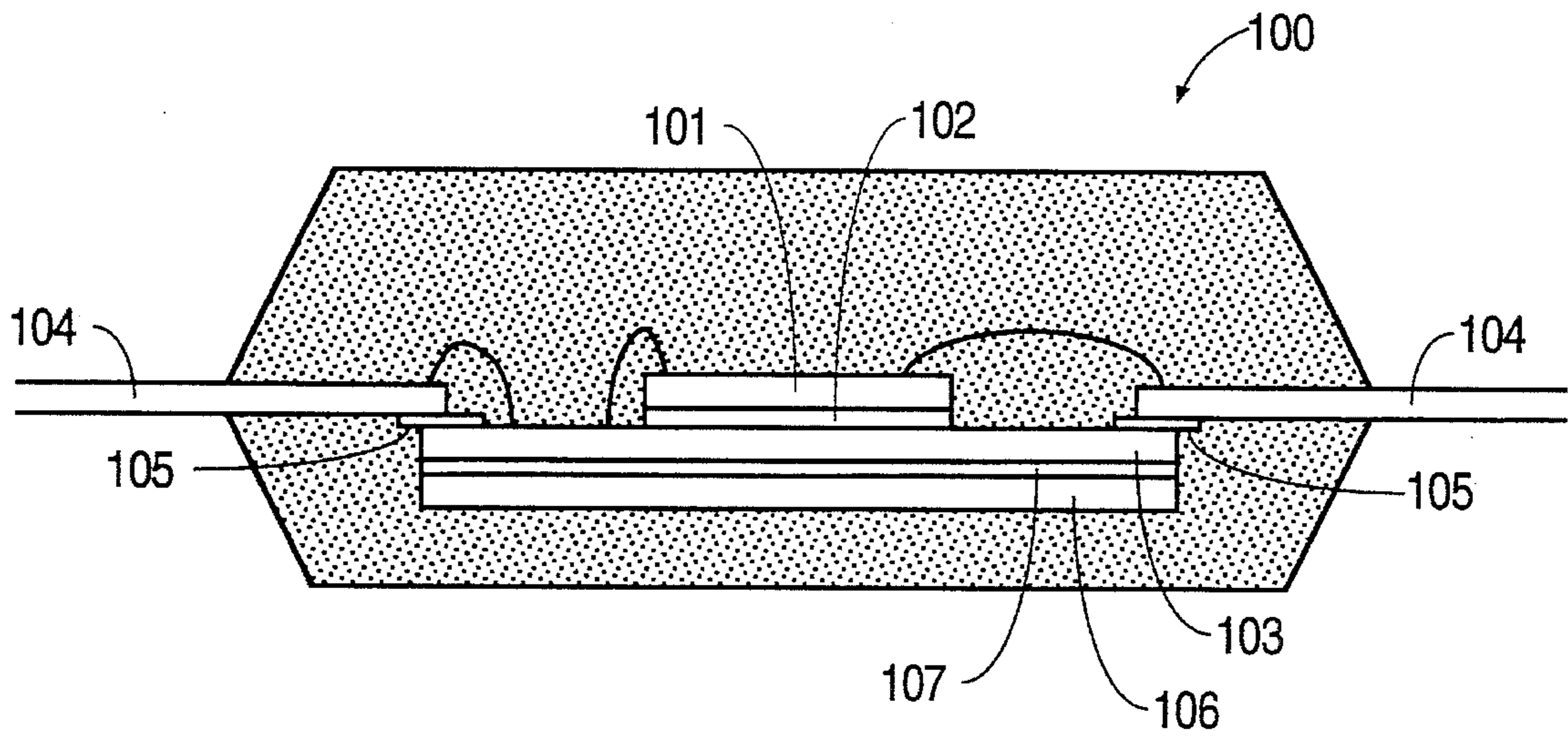
FIG. 1 (PRIOR ART)
